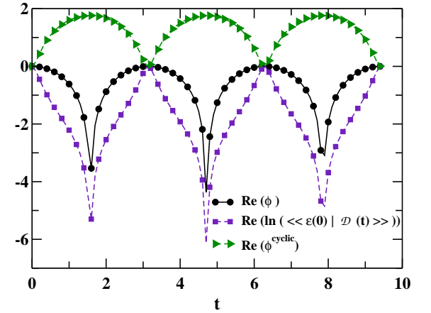
FIG. 3: (Color online) Real part of the GP for a two-level system under bit-flip as a function of time. The decoherence parameter \gamma_b is set to 0.1 (in units such that \omega = 1 ).
