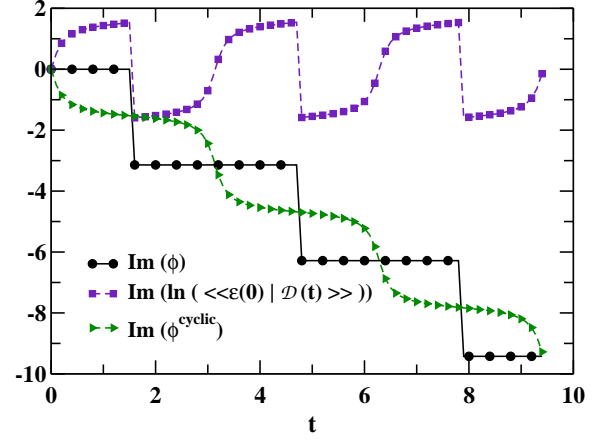
FIG. 2: (Color online) Imaginary part of the GP for a two-level system under bit-flip as a function of time. The decoherence parameter \gamma_b is set to 0.1 (in units such that \omega = 1 ).
