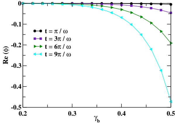
FIG. 1: (Color online) Real part of the geometric phase for a two-level system under bit-flip as a function of the decoherence parameter \gamma_b (in units such that \omega = 1 ).
