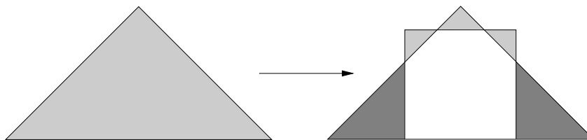
Figure 4.1: Subdivision rule
