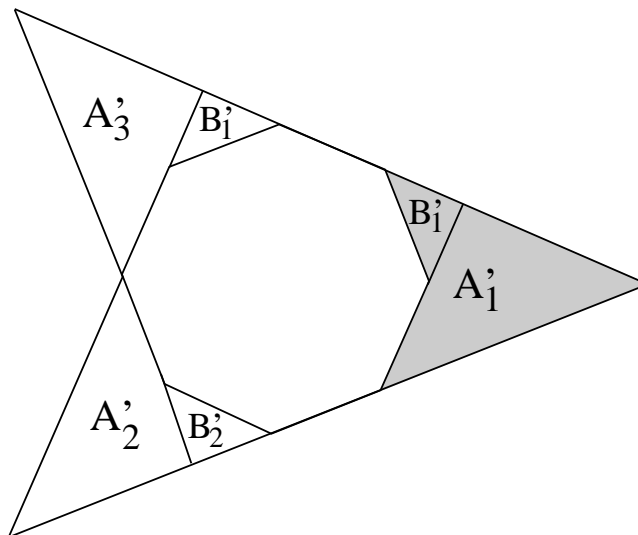
Figure 6.3: Renormalization Scheme
