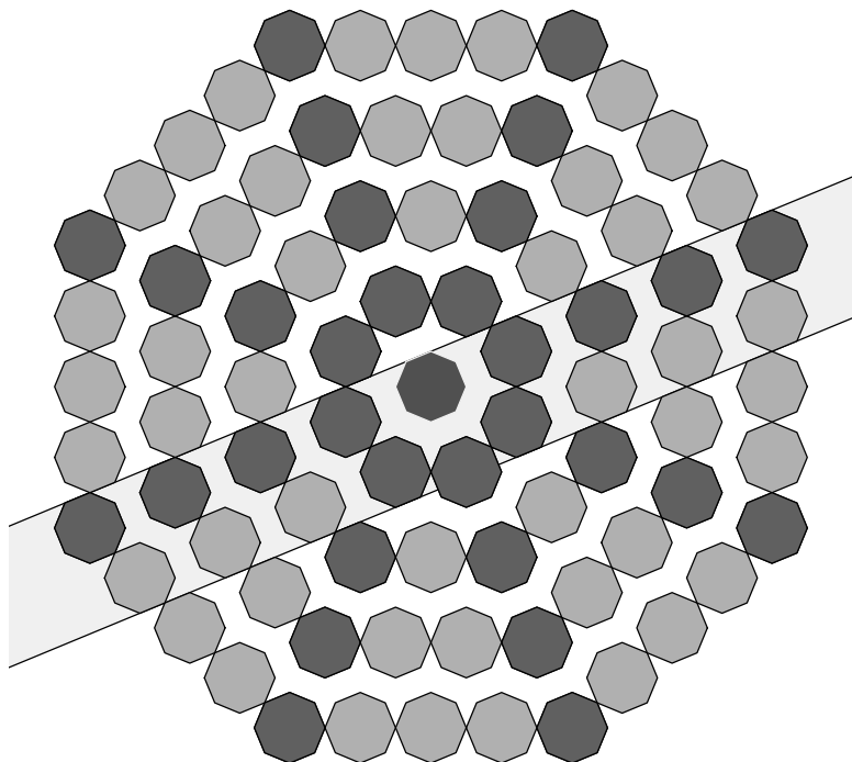
Figure 5.3: Octagonal orbits
