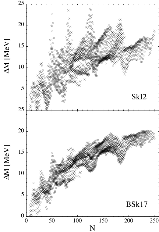
FIG. 1: Differences between the HFB energies estimated with and without the J^2 -terms for two Skyrme forces SkI2 (upper panel) and BSk17 (lower panel) for all even-even nuclei with Z, N > 8 and Z < 110 lying between the proton and neutron driplines.
