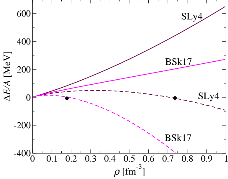
FIG. 2: Difference between the energy per particle in fully polarized neutron matter and in unpolarized neutron matter for two Skyrme forces SLy4 and BSk17, with (dashed line) and without (solid line) the J^2 and J_q^2 terms and their time-odd part. The black dots indicate the densities at which the difference vanishes.
