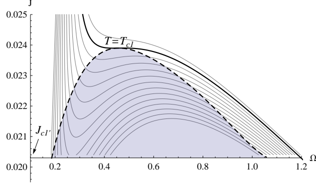
FIG. 5: The dashed curve is the coexistence curve of phase transition above T_{c1} . The coexistence curve ends at J_{c1'} , because the stable area is too small to apply the equal area law at the corresponding temperature T_{c1'} .
