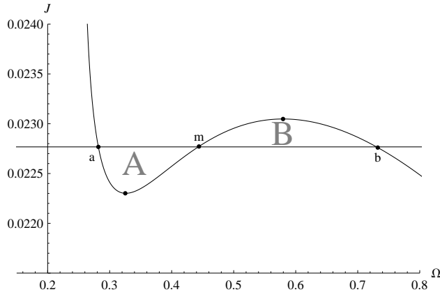
FIG. 4: Applying the equal-area law on an isotherm at a temperature T > T_{c1} .
