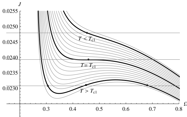
FIG. 2: The critical isotherms near the critical temperature T_{c1} .
