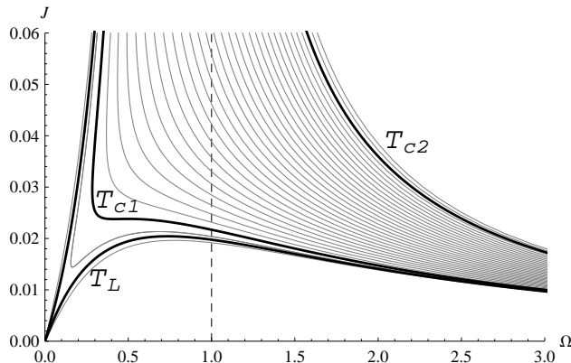
FIG. 1: The isotherms on the (J, \Omega) space. Three isotherms has been labeled by their temperatures, T_L , T_{c1} and T_{c2} . T_L > T_{c1} > T_{c2} .
