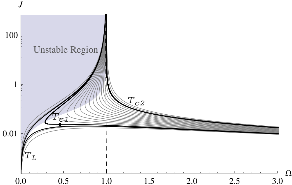
FIG. 3: The diagram contains all three critical phenomena with their features. Here J is plot on the log coordinate.
