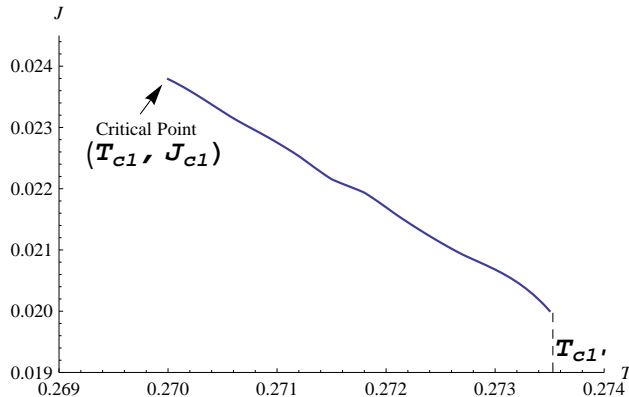
FIG. 6: Phase diagram near critical point T_{c1} . Similar to the phase diagram of liquid/gas phase transition[23, 27].
