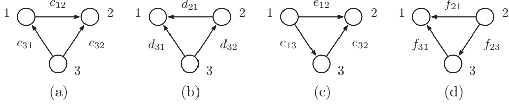
Figure 3: Alternative DAGs.
