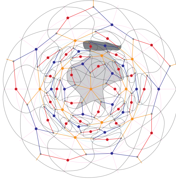
FIGURE 38. The z^4 -polygon (lighter one) and the yz^2 -polygons (darker one)
