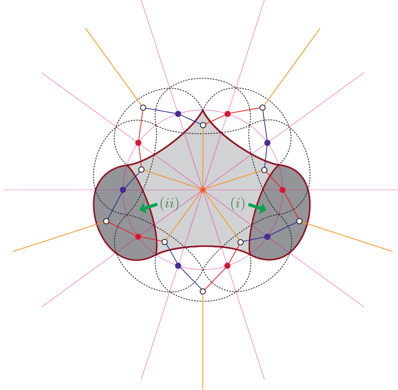
FIGURE 34. Polygons contributing to z^{r-2k}
