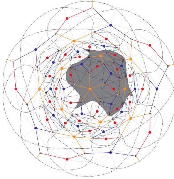
FIGURE 39. The z^3 -polygon
