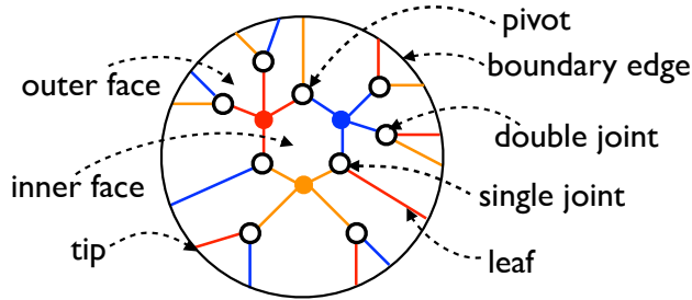
FIGURE 15. Terminology on a cellulation. Red (Apple), blue (Blueberry) and orange (Cantaloup) colors represent A, B and C labels.
