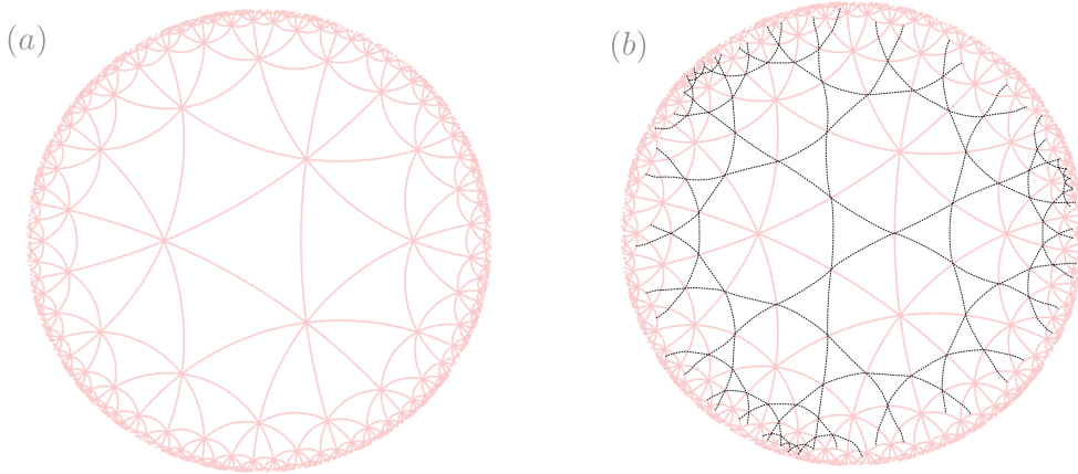
FIGURE 2. (a) Tessellation of the universal cover of \mathbb{P}_{4,4,4}^1 by real equator, (b) Seidel Lagrangian in \mathbb{H}^2
