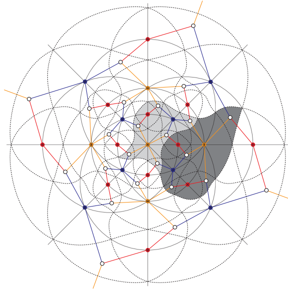
FIGURE 37. yz^2 - and z^2 - polygons
