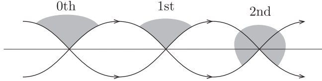
FIGURE 13. Corners of a holomorphic polygon
