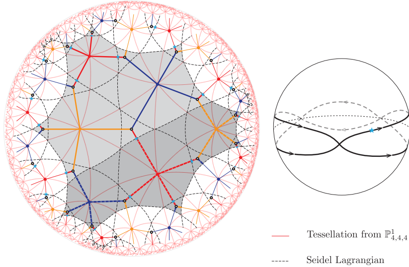
FIGURE 17. An elementary move from a hexagon in a (4, 4, 4) -diagram to a 9-gon.
