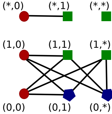
Figure 1: Graph \mathcal{H} = \pi(\mathcal{G}) when a_{1,i_2} = 1 .
