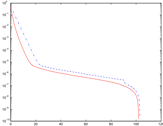
Figure 2: Normalized norm of the error on the iterate vs computation time (in seconds) for Experiment 1 (blue, dash-dot line) and Experiment 2 (red, continuous line).
