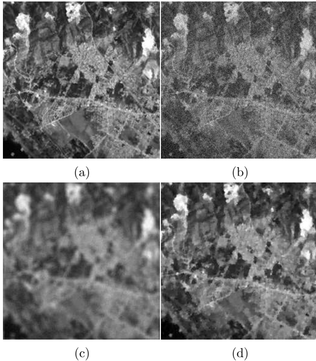
Figure 1: Original image \bar{x} (a), noisy image w_1 (SNR = 5.87 dB) (b), blurred image w_2 (SNR = 16.63 dB) (c), and restored image \tilde{x} (SNR = 21.61 dB) (d).
