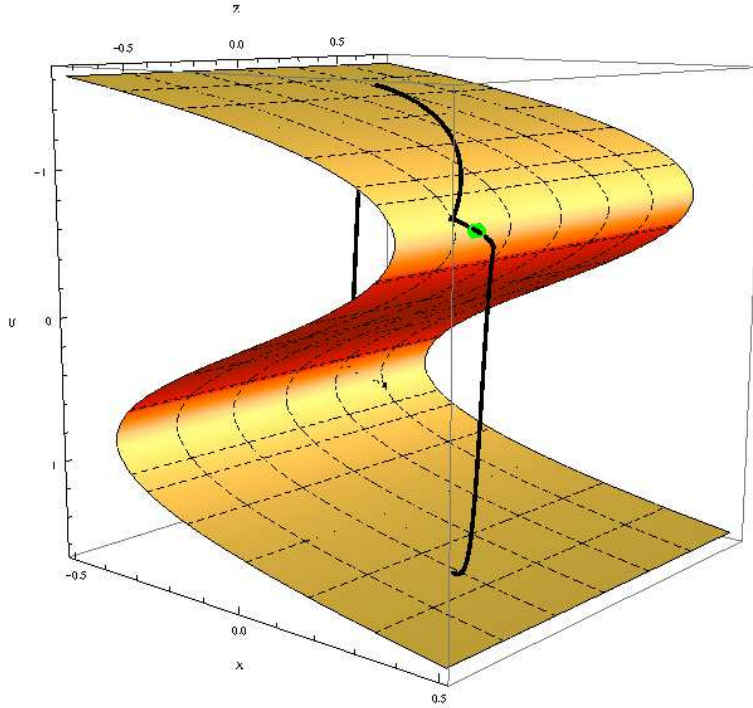
FIGURE 3. Canards solutions of Chua’s system (18).
