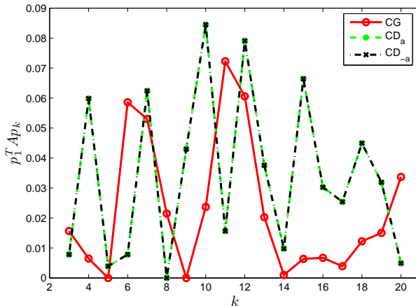
Fig. 3 Conjugacy loss for an illconditioned problem described by the coefficient matrix A_{1_0} in [13], using only the CG, CD_a (the CD class setting \gamma_0 = 1 and \gamma_k = a_k , k \geq 1 ) and CD_{-a} (the CD class setting \gamma_0 = 1 and \gamma_k = -a_k , k \geq 1 ). The quantity p_1^T A p_k is reported for k \geq 3 . The choices \gamma_k = a_k and \gamma_k = -a_k are definitely comparable, and are preferable to the CG for k \in \{3, 6, 8, 11, 20\} .
