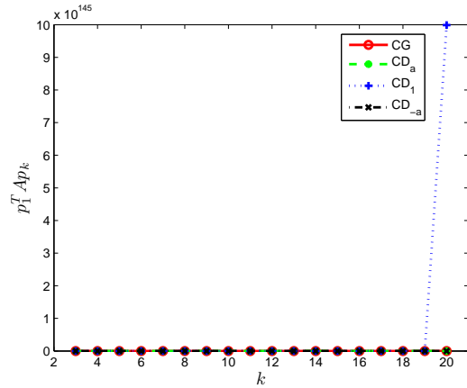
Fig. 2 Conjugacy loss for an illconditioned problem described by the coefficient matrix A_{10} in [13], using the CG, CD_a (the CD class setting \gamma_0 = 1 and \gamma_k = a_k , k \geq 1 ), CD_1 (the CD class setting \gamma_k = 1 , k \geq 0 ) and CD_{-a} (the CD class setting \gamma_0 = 1 and \gamma_k = -a_k , k \geq 1 ). The quantity p_1^T A p_k is reported for k \geq 3 . As evident, the choice \gamma_k = 1 , k \geq 0 , can yield very harmful results when the coefficient matrix is illconditioned
