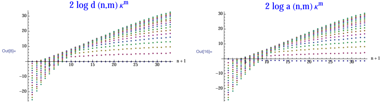
Figure 2: Amplitude coefficients of Figure 1 in the form 2 \log(\kappa^m d(n, m)) and 2 \log(\kappa^m a(n, m)) appearing in Eqs. (4.6)-(5.6). The label n = 0, 1, \dots, 32 is shown along the horizontal axis and the sequence of curves corresponds to m = 0, 2, \dots, 32 with m increasing from bottom to top (on the right of each plot).
