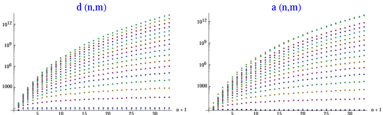
Figure 1: Coefficients d(n, m) and a(n, m) for generating functions of amplitudes (3.23)-(3.24) at threshold, from Ref. [5]. The label n = 0, 1, \dots, 32 is shown along the horizontal axis and the sequences of curves correspond to m = 0, 2, \dots, 32 from bottom to top. \kappa = M_W/M_h \simeq 0.6397 .
