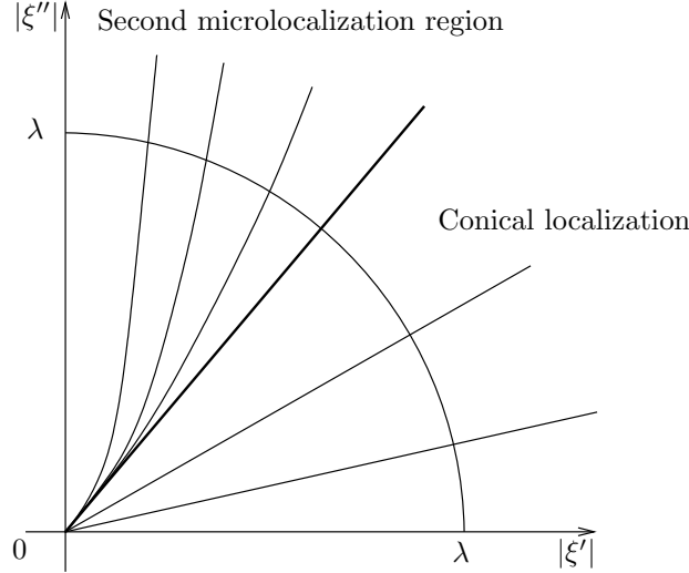
Figure 1: Classical conical localization and second microlocalization on the singular set.
