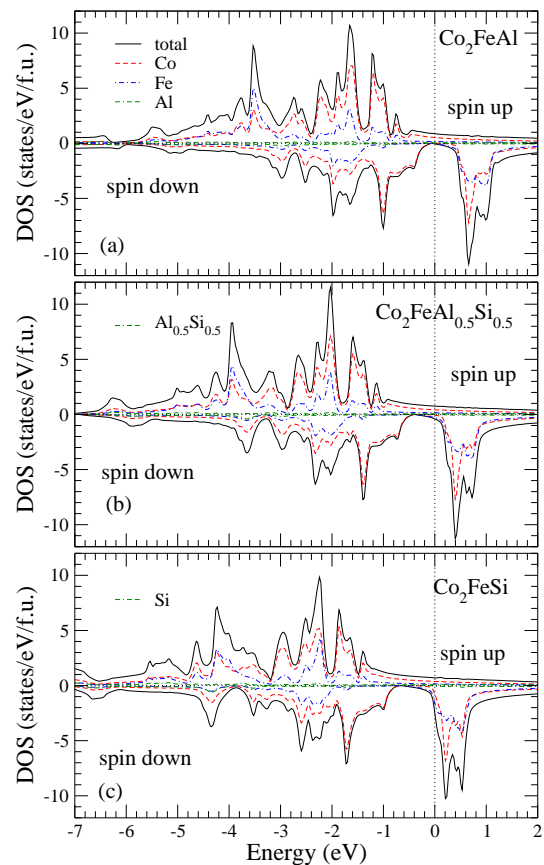
FIG. 1. (color online) Total and site decomposed density of states (DOS) for (a) \text{Co}_2\text{FeAl} , (b) \text{Co}_2\text{FeAl}_{0.5}\text{Si}_{0.5} and (c) \text{Co}_2\text{FeSi} . The Fermi level is at zero.
