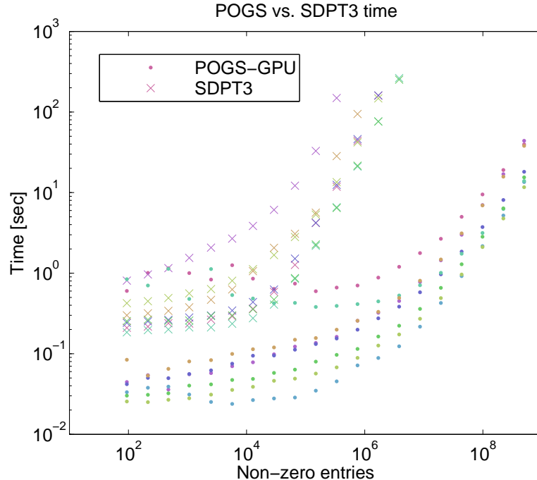
Figure 1: POGS (GPU version) vs. SDPT3 for dense matrices (color represents problem class).
