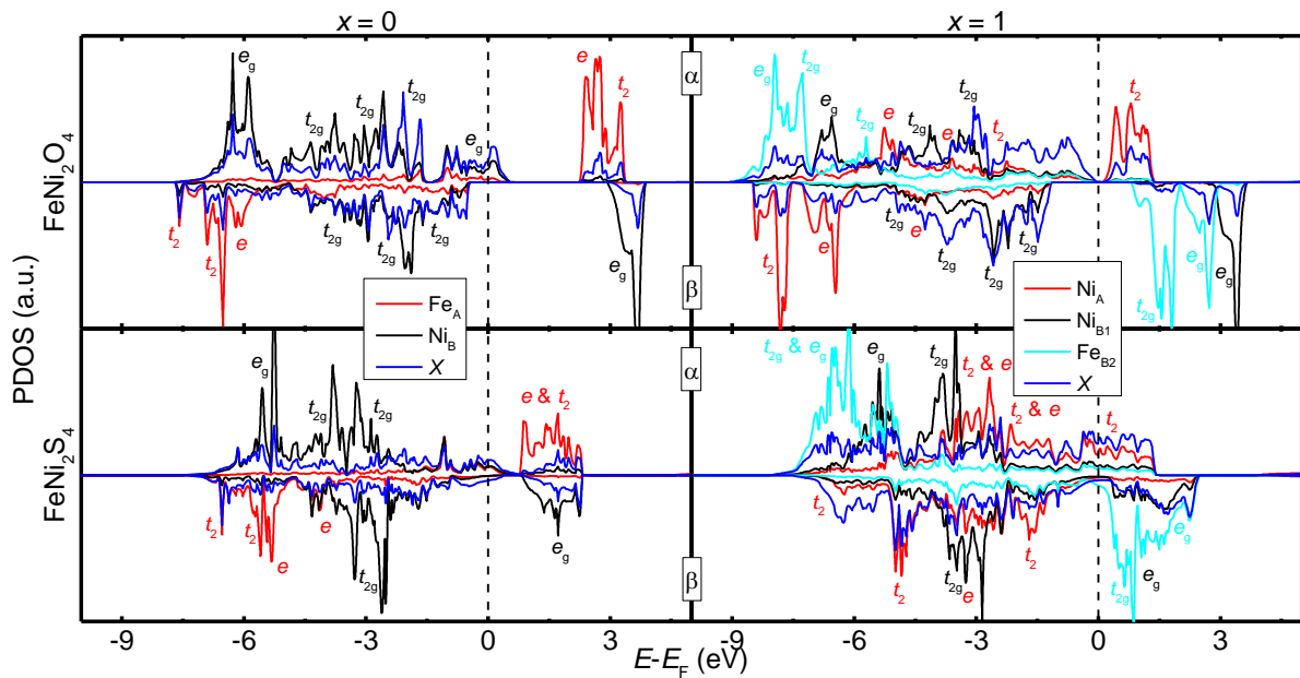
FIG. 6. Atomic projections of the spin decomposed total density of states (PDOS) for \text{FeNi}_2\text{O}_4 and \text{FeNi}_2\text{S}_4 . Fe and Ni contributions are from the 3d bands. O and S contributions are from the 2p and 3p orbitals respectively.
