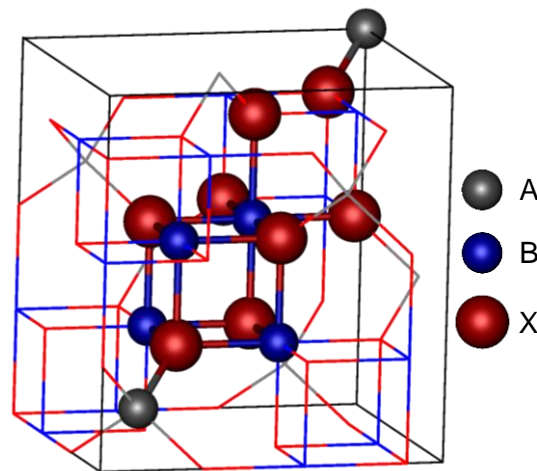
FIG. 1. Schematic representation of one full unit cell of a perfect spinel, highlighting one of the four primitive rhombohedral cells. The spinel structure has the symmetry group Fd\bar{3}m with three ion sites: tetrahedral (A), octahedral (B) cation positions and the anion (X) position.
