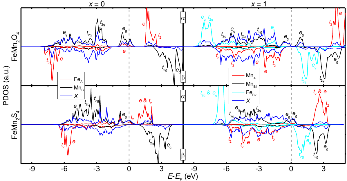
FIG. 4. Atomic projections of the spin decomposed total density of states (PDOS) for \text{FeMn}_2\text{O}_4 and \text{FeMn}_2\text{S}_4 . Fe and Mn contributions are from the 3d bands. O and S contributions are from the 2p and 3p orbitals respectively.
