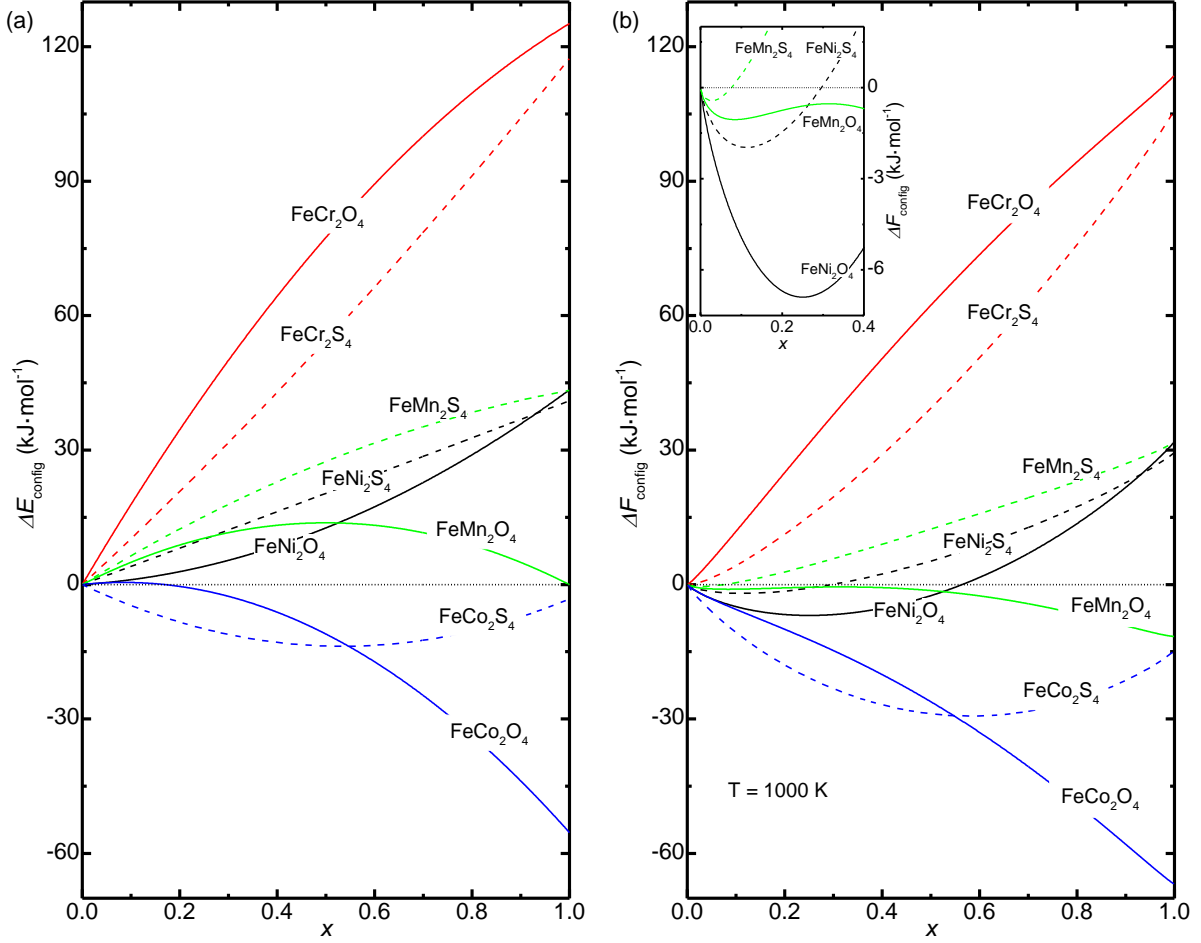
FIG. 2. (a) Configurational inversion energy ( \Delta E_{\text{config}} ) and (b) configurational inversion free energy ( \Delta F_{\text{config}} ) as a function of the inversion degree for \text{FeM}_2\text{X}_4 spinels. Inset shows enlargement of \Delta F_{\text{config}} for the \text{FeMn}_2\text{X}_4 and \text{FeNi}_2\text{X}_4 (thio)spinels.
