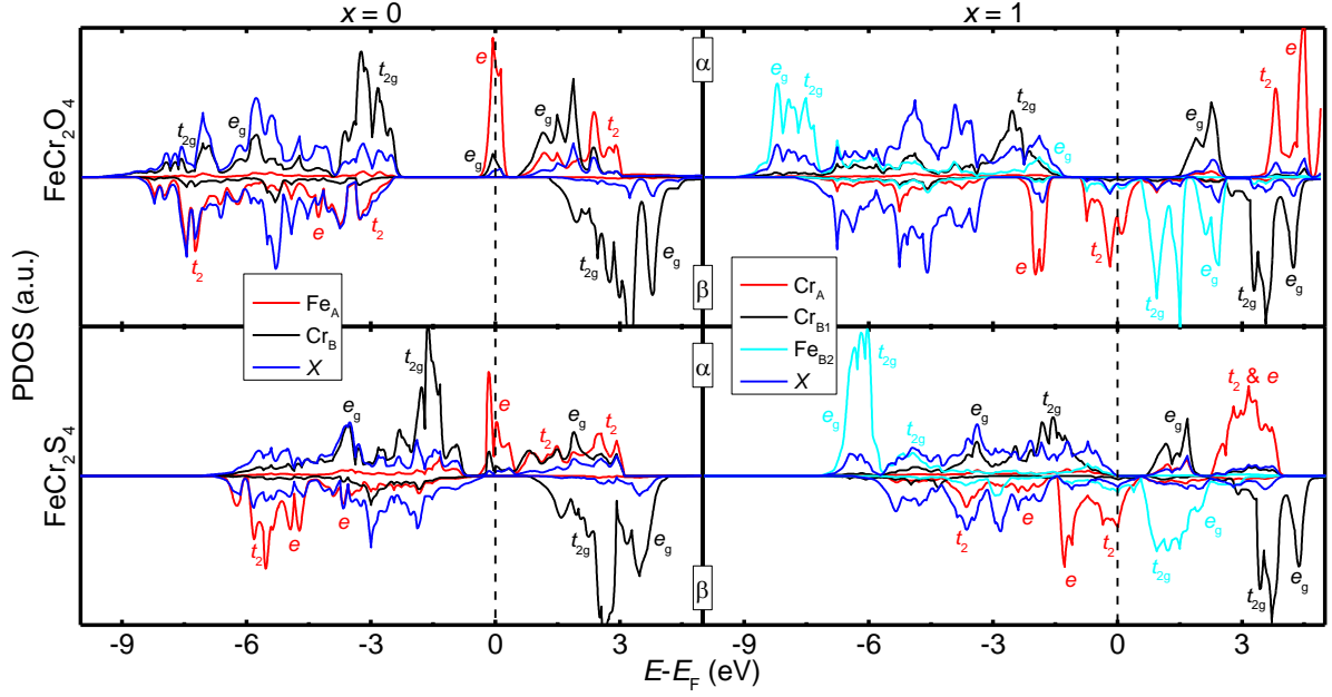
FIG. 3. Atomic projections of the spin decomposed total density of states (PDOS) for \text{FeCr}_2\text{O}_4 and \text{FeCr}_2\text{S}_4 . Fe and Cr contributions are from the 3d bands. O and S contributions are from the 2p and 3p orbitals respectively.
