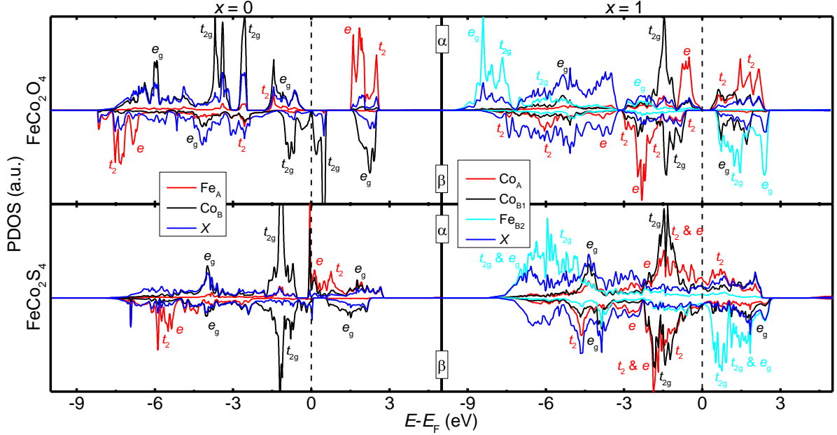
FIG. 5. Atomic projections of the spin decomposed total density of states (PDOS) for \text{FeCo}_2\text{O}_4 and \text{FeCo}_2\text{S}_4 . Fe and Co contributions are from the 3d bands. O and S contributions are from the 2p and 3p orbitals respectively.
