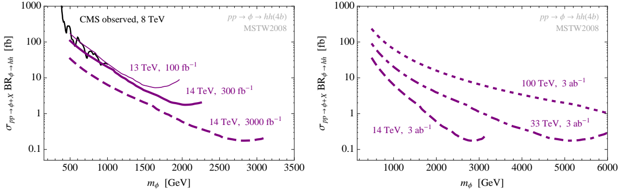
Figure 4. Left: CMS 95% C.L. exclusion (black) on \sigma_{pp \rightarrow \phi} \times \text{BR}_{\phi \rightarrow hh} from the 4b channel, together with the projections for the LHC at 13 TeV with 100 \text{ fb}^{-1} (thin purple), and at 14 TeV with 300 \text{ fb}^{-1} (solid purple) and 3000 \text{ fb}^{-1} (purple dashed). Right: reach in the hh \rightarrow 4b channel of the HL-LHC (dashed), HE-LHC (dot-dashed) and FCC-hh (dotted) with 3 \text{ ab}^{-1} .
