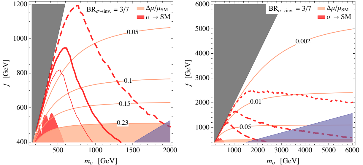
Figure 10. Model with \text{BR}_{\sigma \rightarrow \text{inv.}} = 3/7 . Shaded regions: excluded at 95% C.L. by Higgs couplings (pink), excluded by direct searches (red), \Gamma_\sigma > m_\sigma (blue), unphysical parameters (grey). The notation for the lines is as in figure 7.
