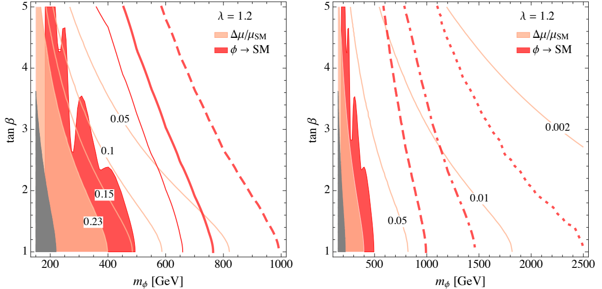
Figure 8. NMSSM with “strong” coupling, \lambda = 1.2 and \Delta = 70 GeV. Shaded regions and lines as in figure 7.
