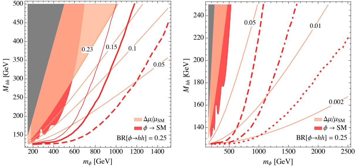
Figure 7. Left: Comparison between the combined direct LHC exclusion and reaches (red) and the deviations in Higgs couplings (pink), with \text{BR}[\phi \rightarrow hh] = 0.25 . Right: the same comparison, in the region relevant for future colliders. The coloured regions are excluded at 95% C.L. and the notation for the lines is the same as in figures 5 and 6.
