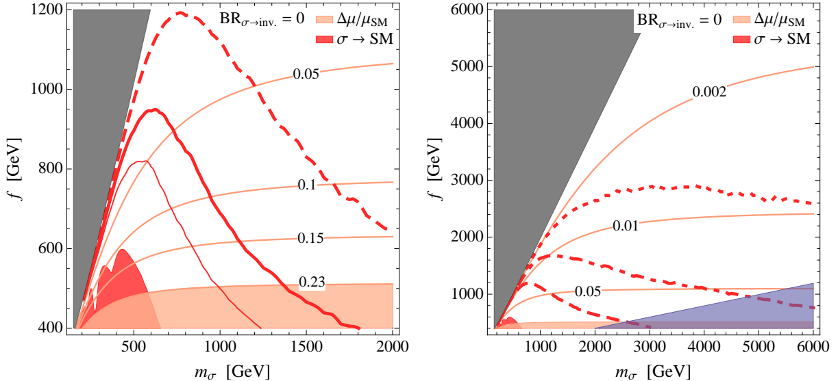
Figure 11. Model with \text{BR}_{\sigma \rightarrow \text{inv.}} = 0 . Notation as in figure 10.
