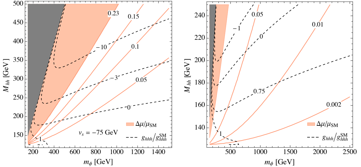
Figure 2. Same as figure 1, but with v_s = -75 GeV.
