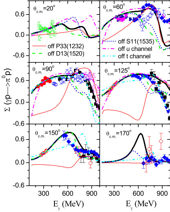
FIG. 6: (Color online) Photon energy dependent beam asymmetry of the \gamma p \rightarrow \pi^0 p reaction. The data are taken from [84] (right triangles), [83] (open up triangles), [85] (open diamonds), [11] (solid diamonds), [13] (down triangles), [86] (open circles), [14] (solid squares), [87] (solid circles), and [88] (open squares). The results by switching off the contributions from various partial waves are indicated explicitly by different legends in the figure.
