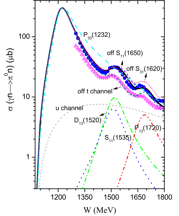
FIG. 13: (Color online) Total cross section as a function of the c.m. energy W for the \gamma n \rightarrow \pi^0 n reaction. Data are taken from [3]. The results by switching off the contributions from N(1650)S_{11} , \Delta(1620)S_{31} , and t channel; and the partial cross sections for \Delta(1232)P_{33} , N(1535)S_{11} , N(1520)D_{13} , N(1720)P_{13} and u channel are indicated explicitly by different legends in the figure.
