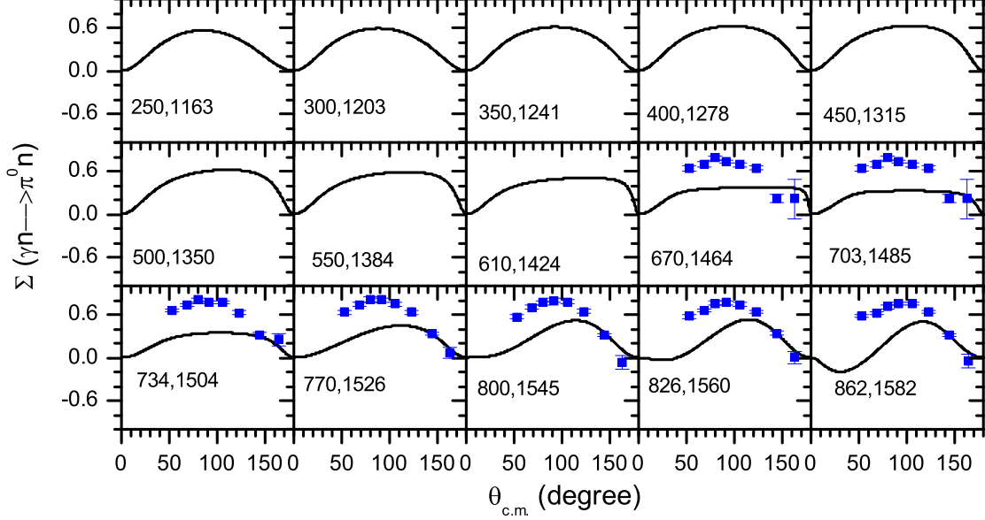
FIG. 15: (Color online) Beam asymmetry of the \gamma n \rightarrow \pi^0 n reaction as a function of scattering angle. Data are taken from [19]. The first and second numbers in each figure correspond to the photon energy E_\gamma (MeV) and the \pi N center-of-mass energy W (MeV), respectively.
