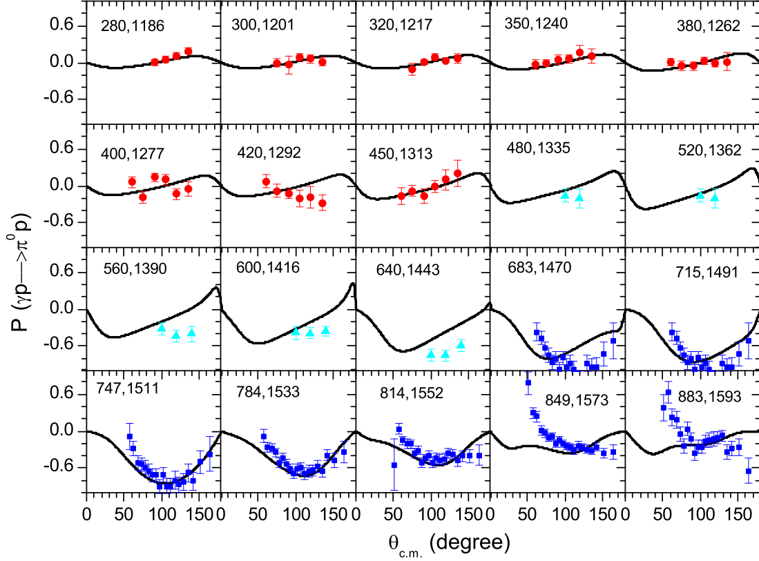
FIG. 7: (Color online) Polarization of recoil protons P of the \gamma p \rightarrow \pi^0 p reaction as a function of scattering angle. Data are taken from [85] (circles), [89] (triangles), and [10] (squares). The first and second number in each figure correspond to the photon energy E_\gamma (MeV) and the \pi N center-of-mass energy W (MeV), respectively.
