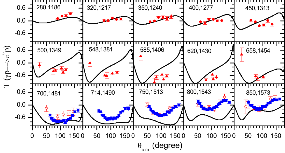
FIG. 9: (Color online) Target asymmetry of the \gamma p \rightarrow \pi^0 p reaction as a function of scattering angle. The data are taken from [85] (solid circles), [100] (solid triangles), [101] (open circles), and [10] (solid squares). The first and second number in each figure correspond to the photon energy E_\gamma (MeV) and the \pi N center-of-mass energy W (MeV), respectively.
