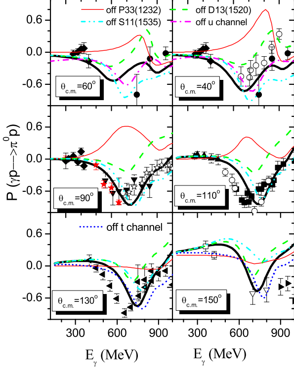
FIG. 8: (Color online) Photon energy dependent polarization of recoil protons for the \gamma p \rightarrow \pi^0 p reaction. Data are taken from [90] (open circles), [91] (solid circles), [92] (diamonds), [93] (solid down triangles), [94] (solid stars), [95] (open stars), [96] (solid squares), [85] (solid up triangles), [97] (solid left triangles), [98] (open down triangles), and [99] (solid right triangles). The results by switching off the contributions from various partial waves are indicated explicitly by different legends in the figure.
