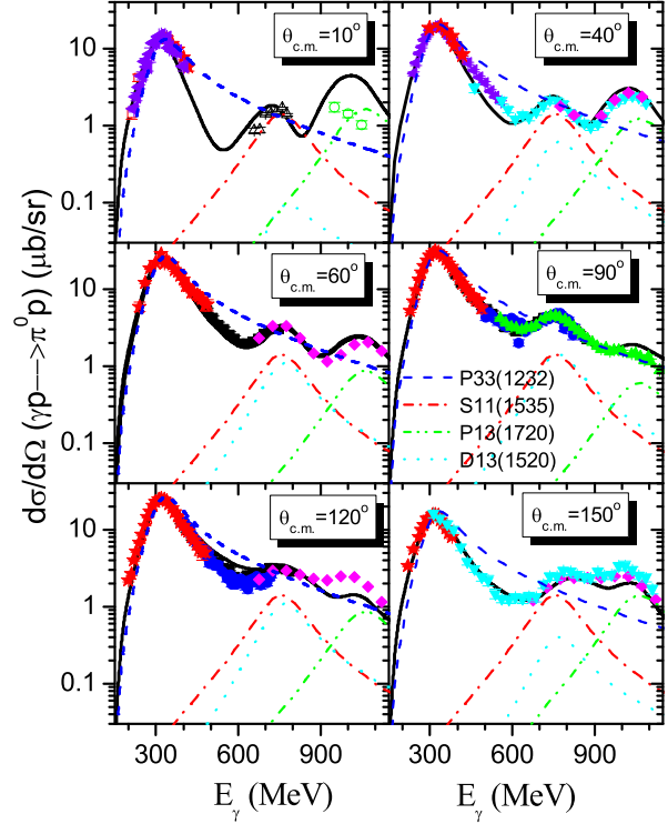
FIG. 3: (Color online) Photon energy dependent differential cross section of the \gamma p \rightarrow \pi^0 p reaction. Data are taken from [5] (left triangles), [77] (open squares), [78] (solid stars), [79] (open triangles), [80] (open circles), [81] (solid squares), [82] (solid circles), [9] (down triangles), [11] (up triangles), [12] (diamonds). The partial cross sections for \Delta(1232)P_{33} , N(1535)S_{11} , N(1520)D_{13} and N(1720)P_{13} are indicated explicitly by different legends in the figure.
