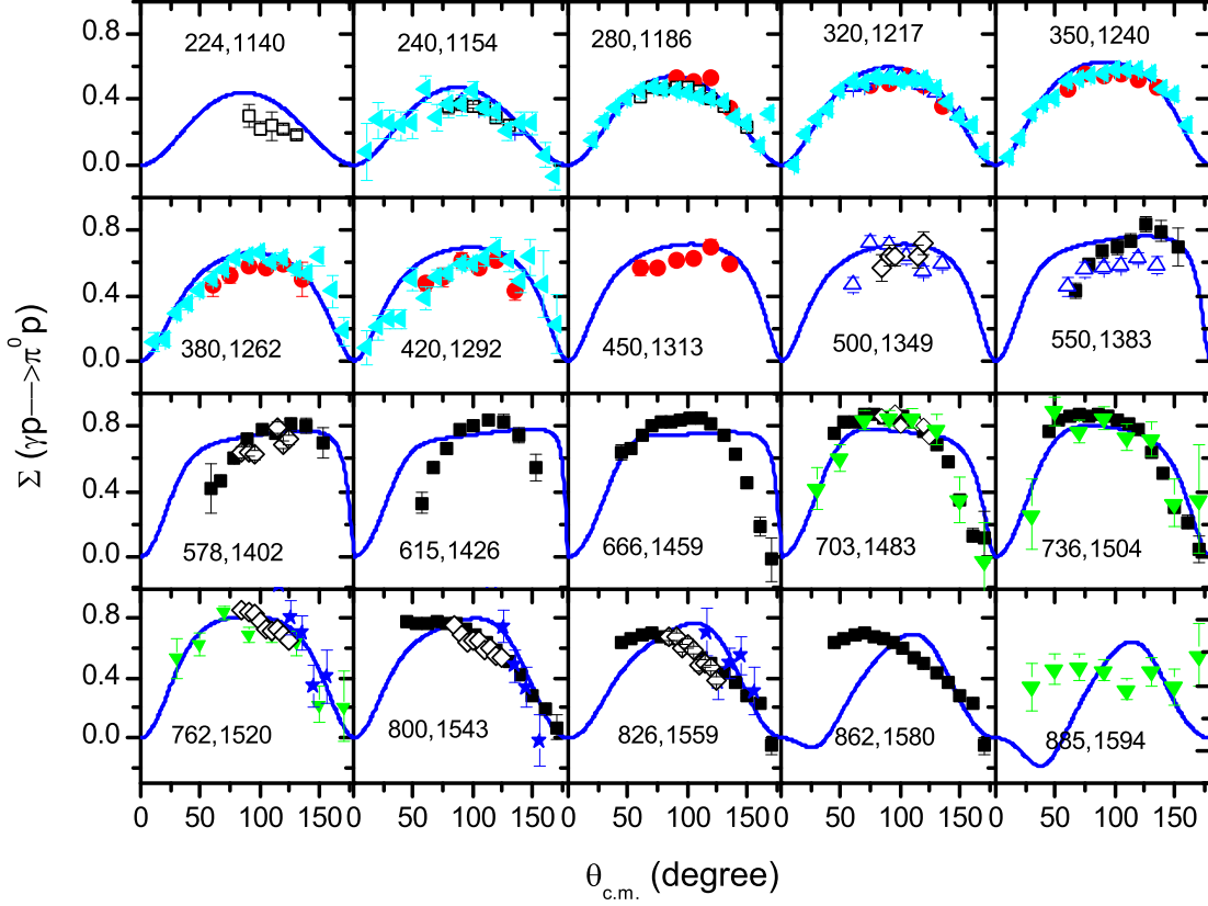
FIG. 5: (Color online) Beam asymmetry of the \gamma p \rightarrow \pi^0 p process as a function of scattering angle. The data are taken from [5] (solid left triangles), [83] (open squares), [84] (open up triangles), [85] (solid circles), [11] (solid squares), [13] (diamonds), [86] (solid down triangles), [14] (stars). The first and second number in each figure correspond to the photon energy E_\gamma (MeV) and the \pi N center-of-mass energy W (MeV), respectively.
