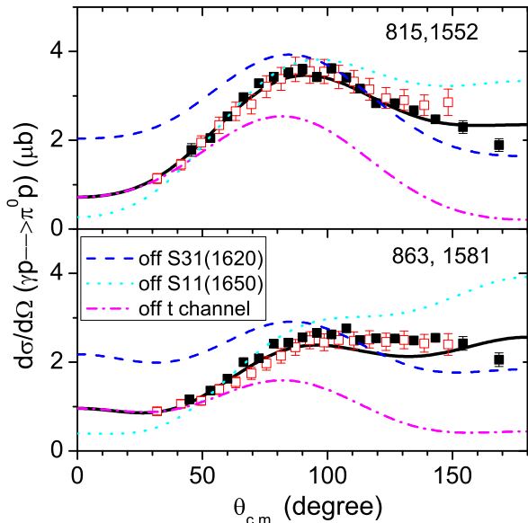
FIG. 4: (Color online) Effects of N(1650)S_{11} , \Delta(1620)S_{31} and t channel on the differential cross sections of the \gamma p \rightarrow \pi^0 p process. Data are taken from [9] (open squares) and [11] (solid squares). The results by switching off the contributions from N(1650)S_{11} , \Delta(1620)S_{31} , and t channel are indicated explicitly by different legends in the figure. The first and second number in each figure correspond to the photon energy E_\gamma (MeV) and the \pi N center-of-mass energy W (MeV), respectively.
