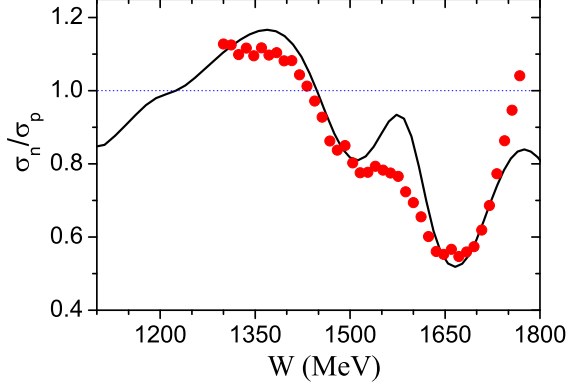
FIG. 14: (Color online) Cross section ratio \sigma_n/\sigma_p between the reactions \gamma n \rightarrow \pi^0 n and \gamma p \rightarrow \pi^0 p as a function of the center-of-mass energy W . Data are taken from Ref. [3].
