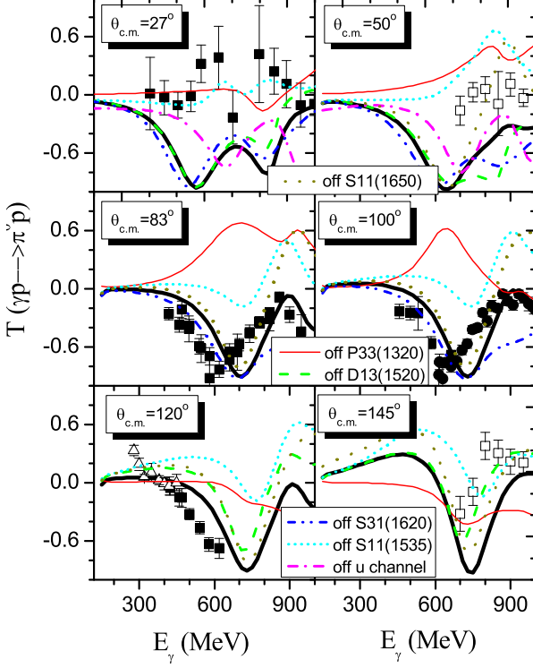
FIG. 10: (Color online) Photon energy dependent target asymmetry of the \gamma p \rightarrow \pi^0 p reaction. The data are taken from [100] (solid squares), [101] (open squares), [102] (solid circles), and [85] (open triangles). The results by switching off the contributions from various partial waves are indicated explicitly by different legends in the figure.
