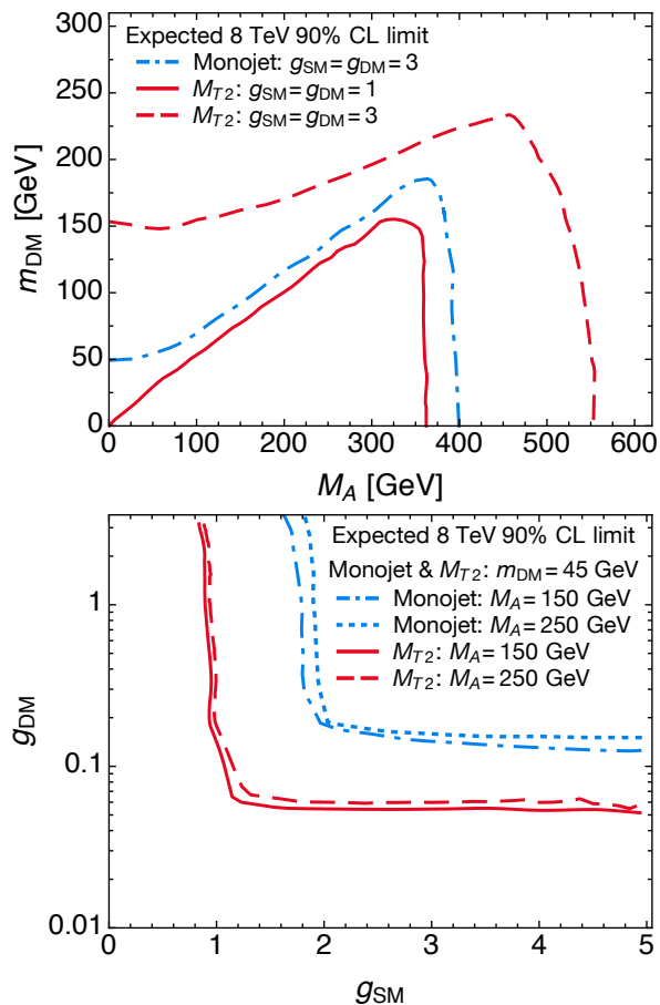
FIG. 1. Comparison of the expected 90% CL exclusion contours from our mono-jet (blue line) and M_{T2} (red line) analyses. Regions below and above the lines are excluded in the upper and lower panels, respectively. The expected M_{T2} limits are significantly better than the expected mono-jet limits over the entire parameter space.
