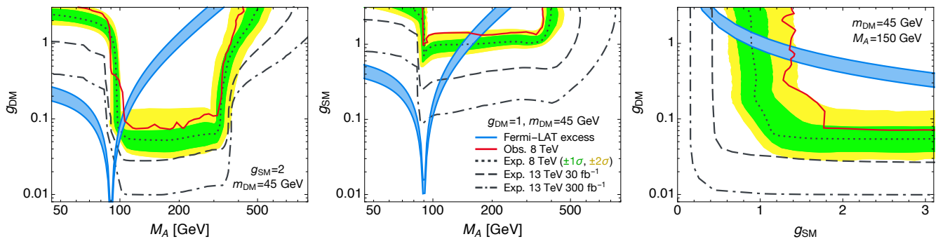
FIG. 2. Comparison of the region consistent with the Fermi-LAT excess (blue shaded) and the observed (red) and expected (black dotted) 90% CL exclusion contours of the M_{T2} analysis. The green and yellow shaded regions show the \pm 1\sigma and \pm 2\sigma bands of the expected M_{T2} limits. The black dashed and dot-dashed lines show projected limits at 13 TeV. The region above the lines is excluded. In each panel, we fix m_{\text{DM}} = 45 GeV and one of \{M_A, g_{\text{DM}}, g_{\text{SM}}\} , as indicated.
