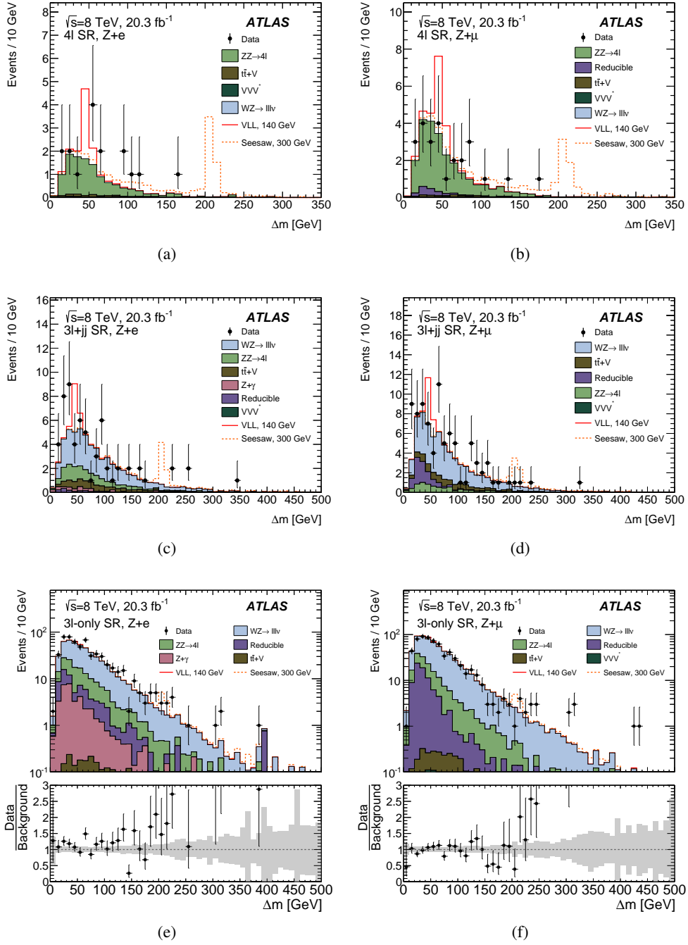
Figure 3: The \Delta m = m_{3\ell} - m_{\ell+\ell-} distributions for the 4\ell (top), 3\ell+jj (middle), and 3\ell -only (bottom) categories, divided into the Z + e (left) and Z + \mu (right) flavour channels. The observed data are shown as black points, while the pre-fit background expectations are shown in the coloured histograms. Also shown are examples for signal contributions for a 140 GeV L^\pm in the VLL model and a 300 GeV L^\pm in the type-III seesaw model. The error bars on the data points represent statistical uncertainties, and the shaded bands represent the systematic uncertainties on the background predictions.
