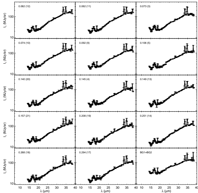
FIG. 4.— Extracted spectra of the selected 14 “dark” regions (i.e., without contamination of point sources) arranged in order of increasing \Sigma_{24\mu\text{m}} (shown in top left corner of each panel in \text{g cm}^{-2} ; the number in parentheses is the region number, see Fig. 1). The summed spectrum from the background (BG) regions is shown in the lower-right panel. The photometric error bars are estimated by CUBISM. All spectra are shown before the zodiacal correction has been applied.
