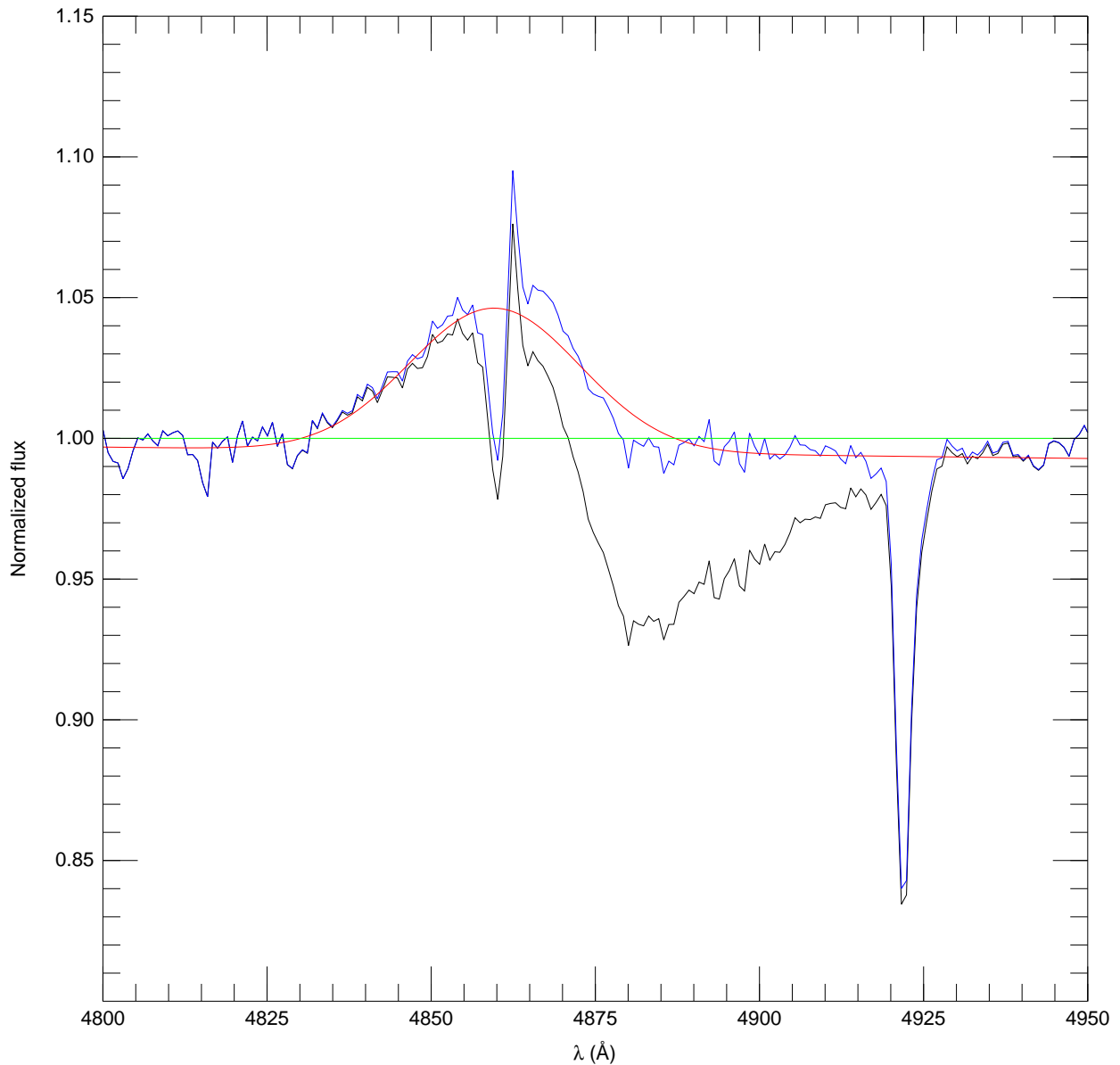
Fig. 4.— The region of H\beta in the spectrum of the extremely reddened star Cygnus OB2-12 ( E_{B-V} = 3.54 , or E(4405-5495) = 3.79 ; Maíz Apellániz 2013), as observed (black) and with the strong DIBs subtracted (blue), together with an approximate gaussian fit to the broad emission component (red). While the fit is not perfect, it indicates that the asymmetry of the observed broad wings is essentially caused by the longward DIBs. These data are from the Galactic O-Star Spectroscopic Survey (GOSSS; Maíz Apellániz et al. 2011); they have a resolving power of 2500 obtained at the Gran Telescopio Canarias and will be fully discussed in a subsequent publication.
