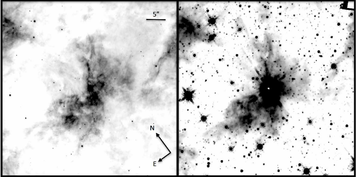
Fig. 5.— HST ACS H\alpha + [N\text{II}] (left) and WFC3 H -band (right) images of VFTS 458 (centered) and surrounding nebulosity. The brightest nebulosity has a roughly bipolar shape with numerous bright and dark condensations, suggestive of ejecta. The most prominent structures are similar between the two bands. (Note vestiges of the stellar diffraction spikes in the cardinal directions of the H -band image.) However, there is similarly structured nebulosity outside the frames to the W and E, so further data are required to establish the nature of the apparently associated nebulosity.
