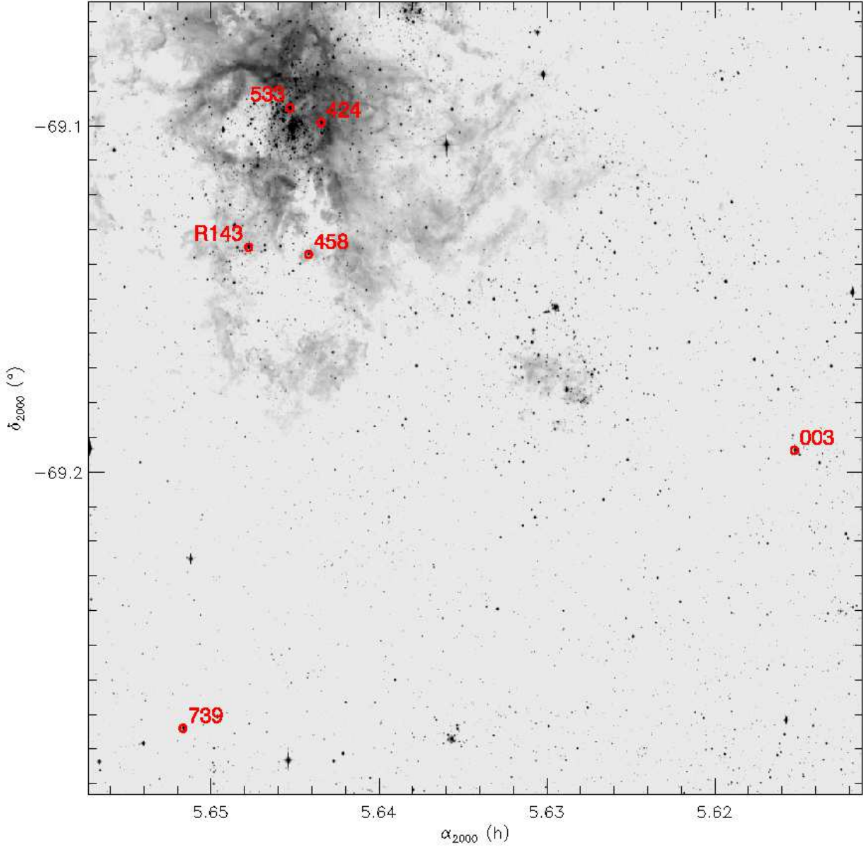
Fig. 1.— Locations of the five VFTS objects in the 30 Dor field. The known LBV R143 is also identified. The extended stellar object at upper left is the cluster core R136. The image is in the V band from the Wide Field Imager on the ESO/MPG 2.2 meter telescope.
