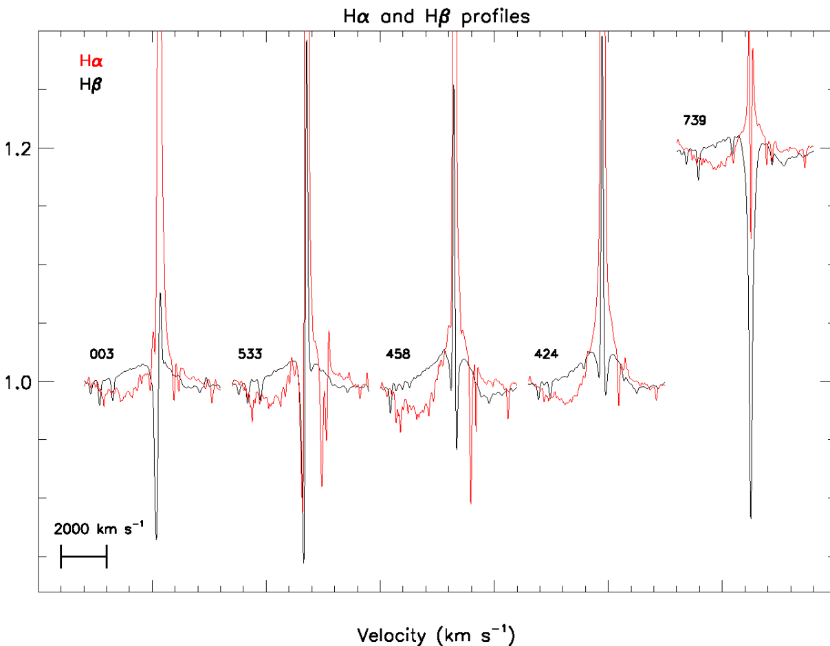
Fig. 3.— Enlargements of the H \beta profiles (black) to show the very similar, extensive asymmetrical wings in all of the spectra, with the corresponding H \alpha profiles (red) superimposed. The narrow H \beta emission in VFTS 533 is a blend of a stellar P Cygni profile and nebular emission, whereas in VFTS 003 it is dominated by the stellar profile, but in VFTS 458 and 424 it is entirely nebular. The apparent shortward, broad absorption troughs in the H \alpha profiles are actually the diffuse interstellar band (DIB) at 6533 Å (Herbig 1995; Walborn & Howarth 2000); E_{B-V} ranges from 0.30 to 0.68 for these objects, with the largest value corresponding to VFTS 458. The VFTS 739 profile has been shifted by +0.2 continuum unit for clarity.
