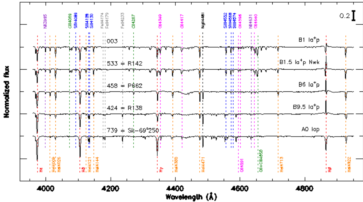
Fig. 2.— The full violet through green spectra of the five VFTS objects. Note the extreme differences between the CNO spectra of VFTS 003 and 533 despite their similar spectral types, as discussed in the text. Some features near those identified in the earlier-type spectra arise from different, lower-ionization species in the later types; e.g., O II \lambda 4349 is replaced by Fe II \lambda 4352. Enlargements of the H \beta profiles are shown in Fig. 3.
