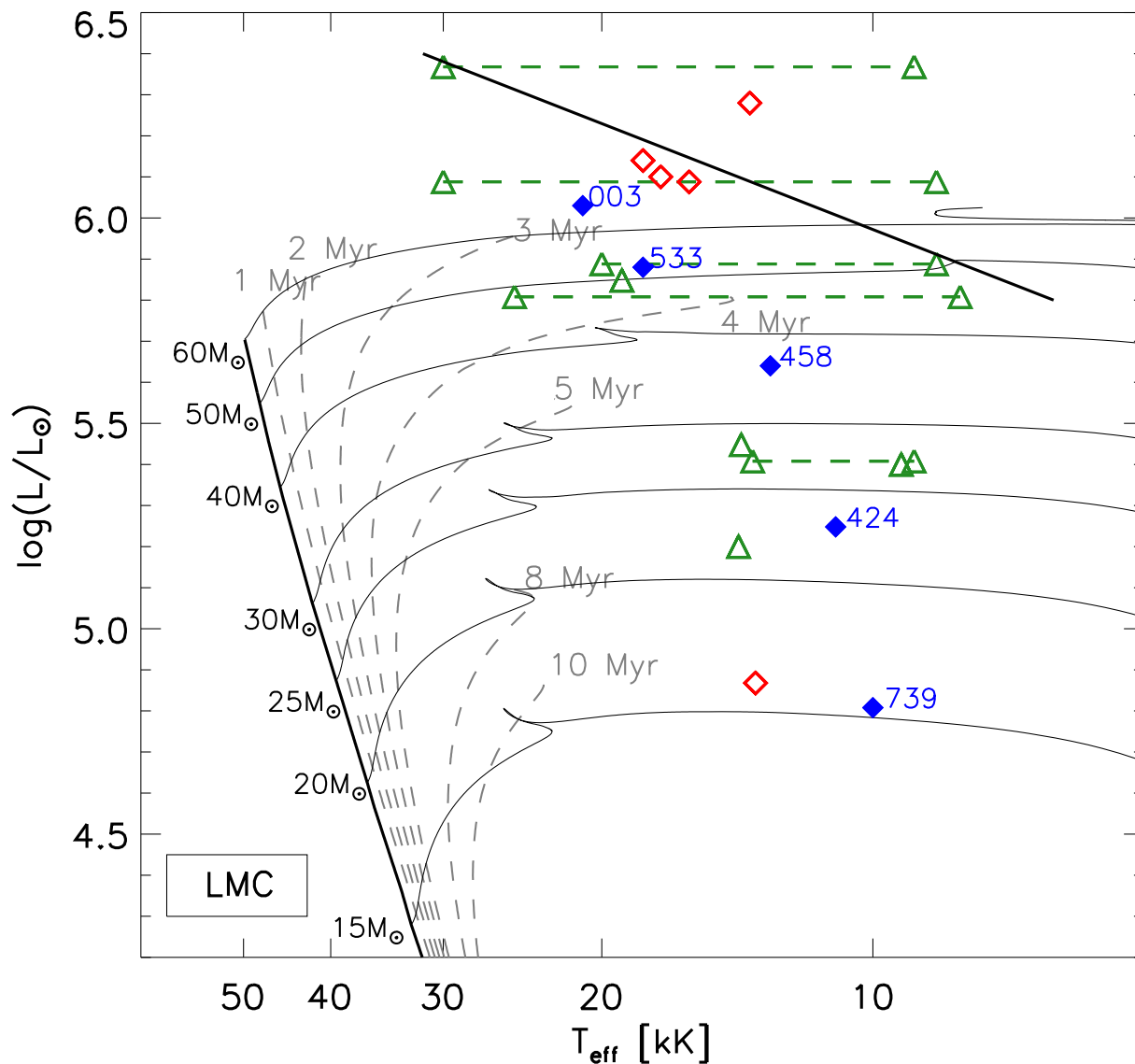
Fig. 6.— HRD comparing the locations of our VFTS objects (labeled blue diamonds; McEvoy et al. 2015; this paper) to those of Galactic hyper/supergiants (red diamonds—top to bottom Cyg OB2-12, HD 190603, \zeta^1 Sco, HD 80077, HD 4841; Lennon et al. 1992; Mel’nik & Dambis 2009; Marco & Negueruela 2009; Clark et al. 2012) and LBVs or candidates (green triangles—top to bottom AG Car, R127, R143, P Cyg, S Dor, HR Car, R71, HD 168607, HD 168625; Humphreys & Davidson (HD) 1994; van Genderen 2001). The diagonal line at upper right is the HD Limit. The LMC evolutionary models are from Brott et al. (2011).
