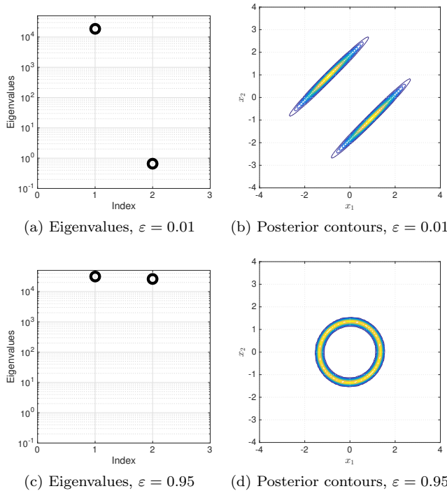
Fig. 5.1: Two cases of \mathbf{A} in the forward map (5.1). The first uses \varepsilon = 0.01 in (5.2) (top row) and the second uses \varepsilon = 0.95 (bottom row). The leftmost figures show the two eigenvalues from \mathbf{C} in (2.2) computed with a high order Gauss-Hermite quadrature rule. The rightmost figures show the contours of the posterior density conditioned on \mathbf{d} = 0.9 . (Colors are visible in the electronic version.)
