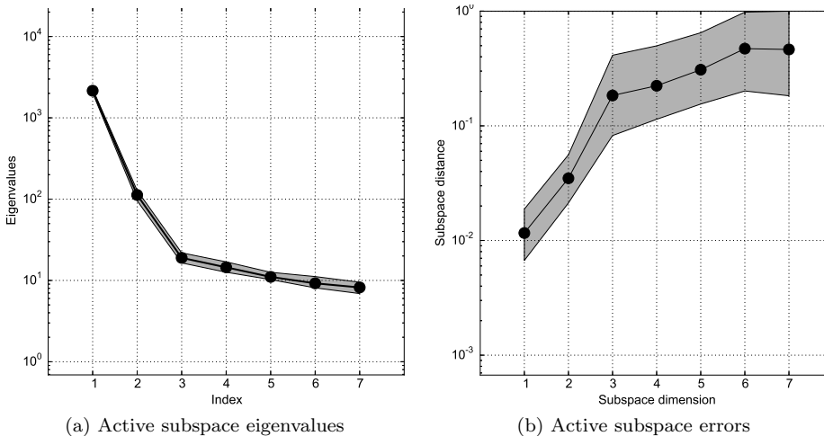
Fig. 5.5: The left figure shows the first seven of the m = 100 eigenvalues \hat{\lambda}_i from the active subspace analysis; see (2.2). The large gaps between eigenvalues \hat{\lambda}_1, \hat{\lambda}_2 and eigenvalues \hat{\lambda}_2, \hat{\lambda}_3 indicate a one-dimensional and a two-dimensional active subspace. The right figure shows the estimated subspace error \varepsilon from (2.12) using the bootstrap as described in [11].
