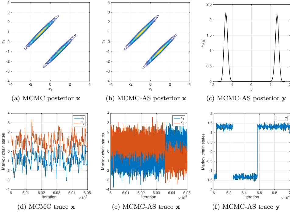
Fig. 5.2: Comparison of standard Metropolis-Hastings MCMC to the active subspace accelerated MCMC. Figure 5.2a shows density estimate of the posterior contours for the standard MCMC, and Figure 5.2b shows the same contours for the samples from Algorithm 1 using the reconstruction (4.2). The plots directly beneath them show trace plots for steps 600000 to 605000; notice that the active subspace-accelerated chain mixes better. The rightmost plots show the univariate posterior on the active variable \hat{y} (above) and its trace plot for 10000 representative steps (below). (Colors are visible in the electronic version.)
