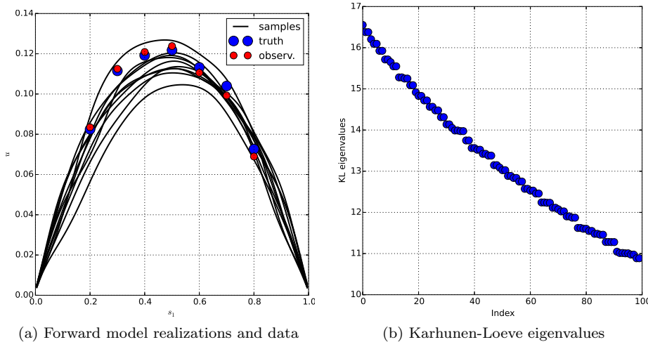
Fig. 5.4: On the left, Figure 5.4a shows ten realizations of the PDE solution with the parameters drawn according to the prior. The blue dots are the observations corresponding to \mathbf{x} = \mathbf{x}_{\text{true}} , and the red dots show the observations perturbed by 1% noise to generate synthetic data for the inverse problem. Figure 5.4b shows the eigenvalues of the Karhunen-Loeve expansion in (5.4). The slow decay corresponds to the short correlation length. (Colors are visible in the electronic version.)
