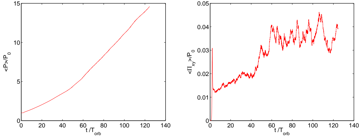
Figure 2. The time evolution of the gas pressure P (left panel) and the total stress normalized by the initial gas pressure (right panel) for the zero-net-flux L = 4H_0 simulation.
