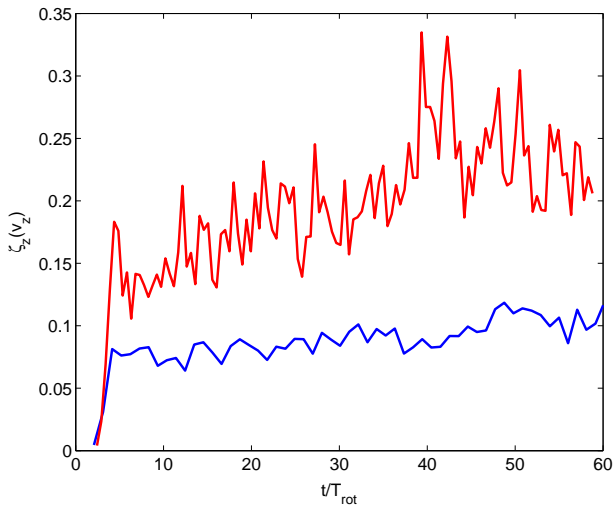
Figure 5. The time evolution of the correlation length, defined in Eq. (13), for the L = 4H_0 simulation without physical diffusivities (blue curve), and the L = 4H_0 simulation with physical diffusivities (red curve).
