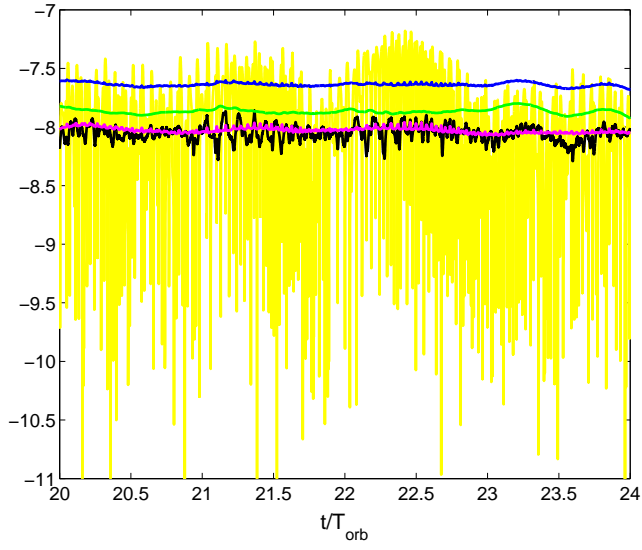
Figure B2. Various box-averaged thermal energy input terms plotted on a \log_{10} scale over 4 orbits. The green curve is the Ohmic heating, pink is the viscous heating, blue is the sum of the Ohmic and the viscous heating, yellow is the pressure heating term and the black curve is the numerical heating.
