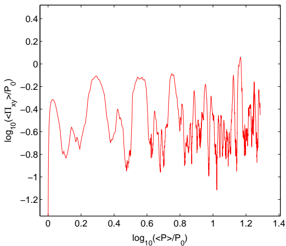
Figure 14. The time evolution of the total stress normalized by the initial gas pressure, as a function of the volume averaged pressure for the (2H_0, 5H_0, H_0) simulation with \Delta = 1/32 , \beta = 500 and reduced heating. The plot should be compared with the right panel of Fig. 13.
