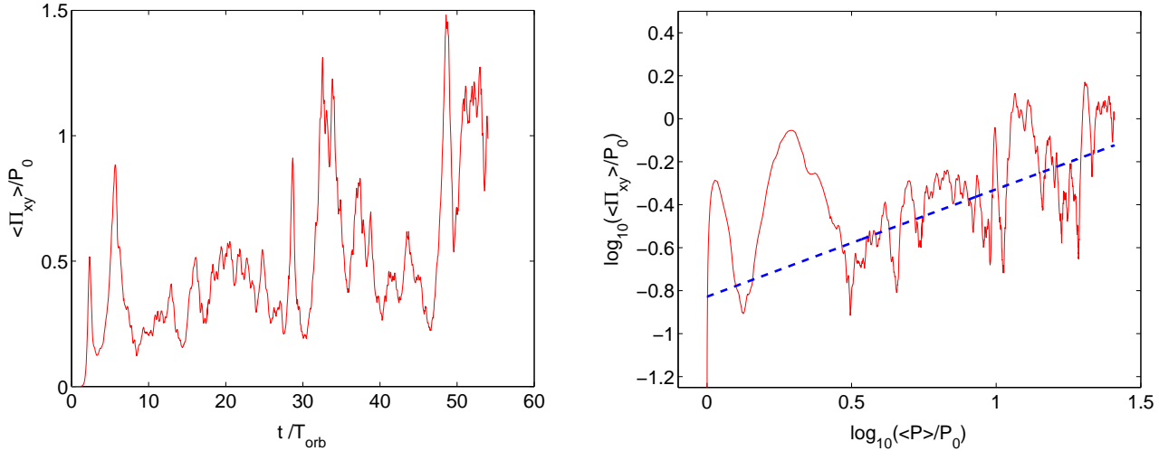
Figure 13. The time evolution of the total stress normalized by the initial gas pressure for the (4H_0, 5H_0, 2H_0) simulation with resolution \Delta = 1/32 , \beta = 500 and reduced heating. The left panel shows \Pi_{xy} as a function of time, the right panel as a function of P . The dashed line has q = 0.5 .
