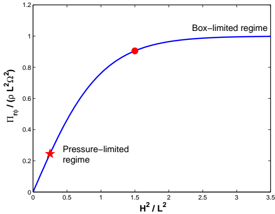
Figure 1. A schematic graph of how we expect the stress \Pi_{r\phi} to depend on scale height H in an unstratified MRI simulation with a box size of L . In monotonically heating runs the stress will evolve by following the blue curve from left to right. Very roughly, the box-limited regime is to the right of the red dot, whereas the pressure-limited regime is to the left of the red star. Ideally, simulations should begin to the left of the red star.
