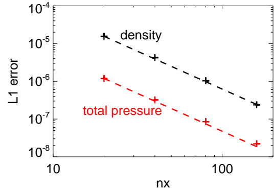
Figure A2. Error on the density (black) and total pressure (red) after one orbit of evolution for the magnetic shearing wave.
