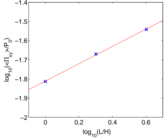
Figure 12. Total stress, normalised by the pressure, as a function of the ratio of the box size to scale height for isothermal net-toroidal simulations. For comparison, a curve with \alpha \propto (L/H_0)^{0.45} is overlaid.
