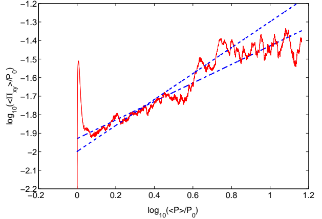
Figure 3. The time evolution of the stress normalized by the initial gas pressure, as a function of the volume averaged pressure for a L = 4H_0 simulation (red solid curve). The blue dashed lines have slopes 0.5 and 0.7.
