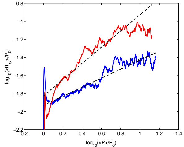
Figure 6. The time evolution of the total stress normalized by the initial gas pressure, as a function of the volume averaged pressure for L = 4H_0 simulations. The red curve is from a simulation with explicit diffusivities. The blue curve is from a simulation identical in all respects other than that explicit diffusivities are omitted. Lines of slopes 0.5 and 0.9 have been superimposed for clarity.
