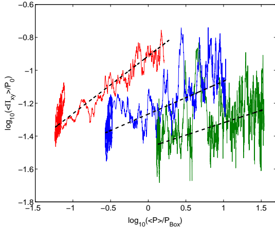
Figure 9. The time evolution of the total stress normalized by the initial gas pressure, as a function of the volume averaged pressure for the net-toroidal simulations with L = 4H_0 (red curve), L = 2H_0 (blue curve) and L = H_0 (green curve). The superimposed lines have slopes 0.15, 0.2, 0.35.
