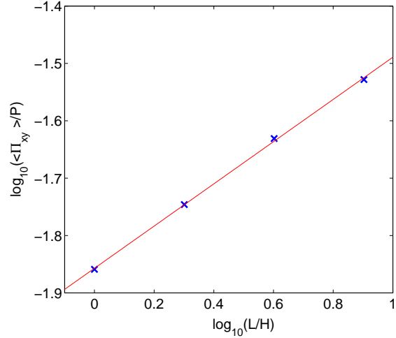
Figure 8. Total stress, normalised by the pressure, as a function of the ratio of the box size to scale height for isothermal zero-net-flux simulations. For comparison, a curve with \alpha \propto (L/H_0)^{0.37} is overlaid.
