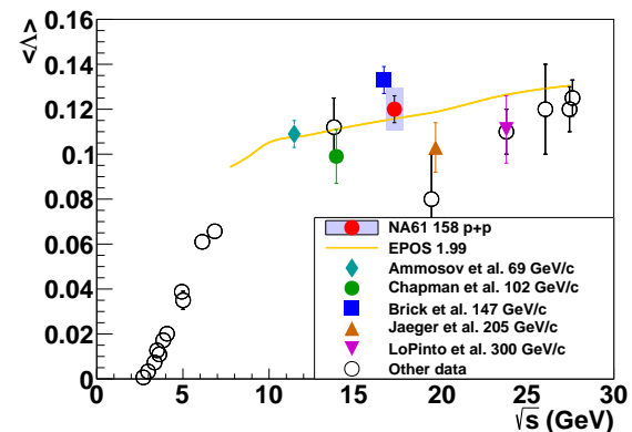
Fig. 16 Collision energy dependence of mean multiplicity of \Lambda hyperons produced in inelastic p+p interactions. Full symbols indicate bubble chamber results [23–27], the solid red dot shows the NA61/SHINE result. Open symbols depict the remaining world data [28]. The EPOS1.99 [19] prediction is shown by the curve. The systematic uncertainty of the NA61/SHINE result is indicated by the shaded bar.
