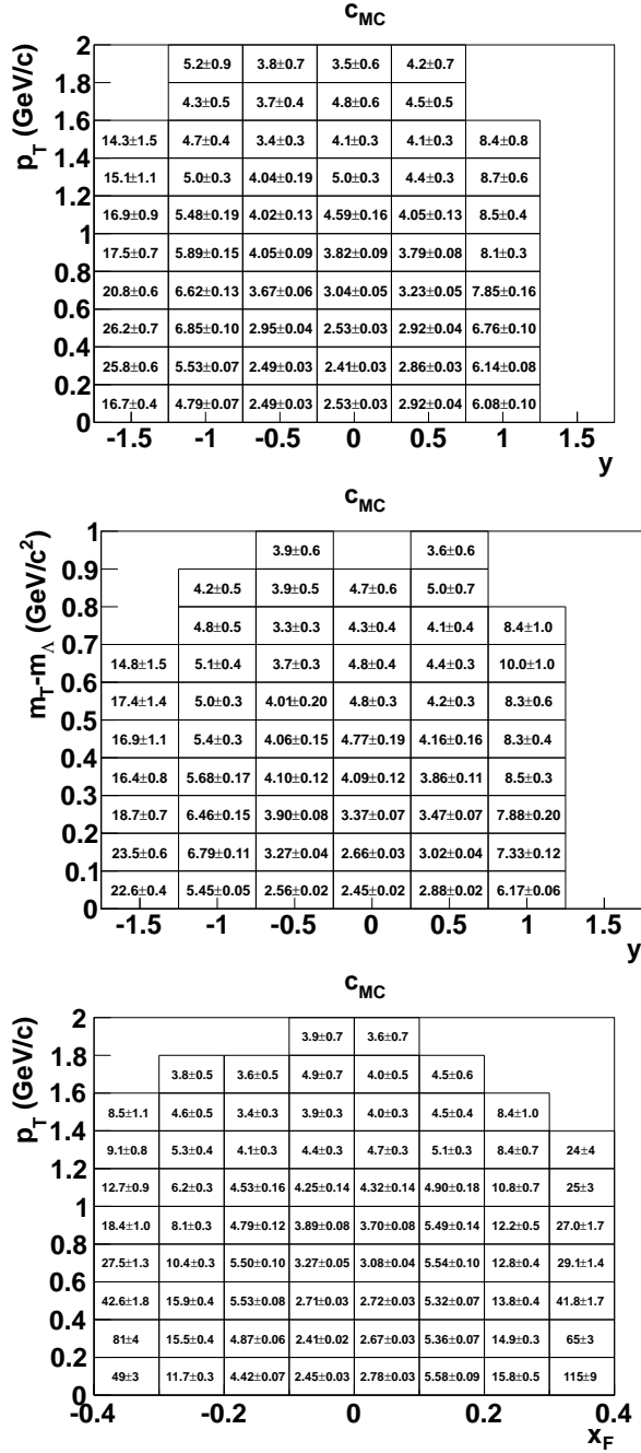
Fig. 9 Correction factors c_{MC} for binning in (y, p_T) at top, (y, m_T - m_\Lambda) at centre and (x_F, p_T) at bottom. The error \Delta c_{MC} ranges from 0.02 to 1.48 for binning in (y, p_T) and (y, m_T) , and from 0.02 to 8.70 for (x_F, p_T) .
