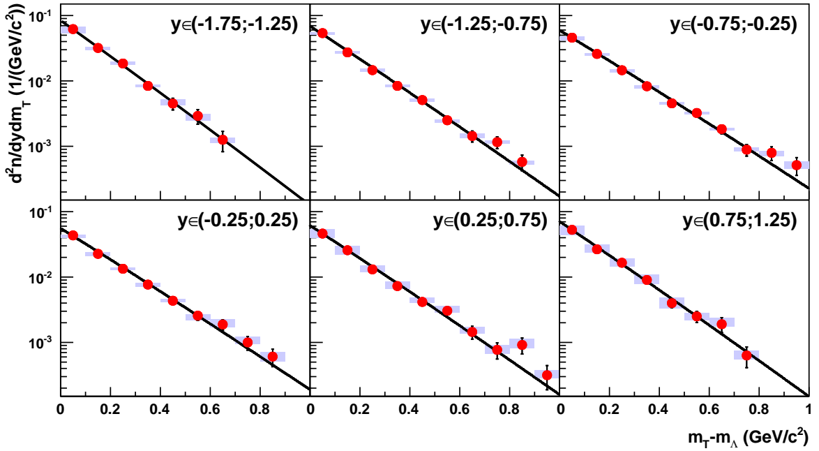
Fig. 12 Spectra \frac{d^2n}{dydm_T} for six bins in rapidity y . The fitted function is given by Eq. (12). The numerical data are listed in Table 2 and the mean transverse mass \langle m_T \rangle - m_\Lambda for each of the bins in Table 5.
