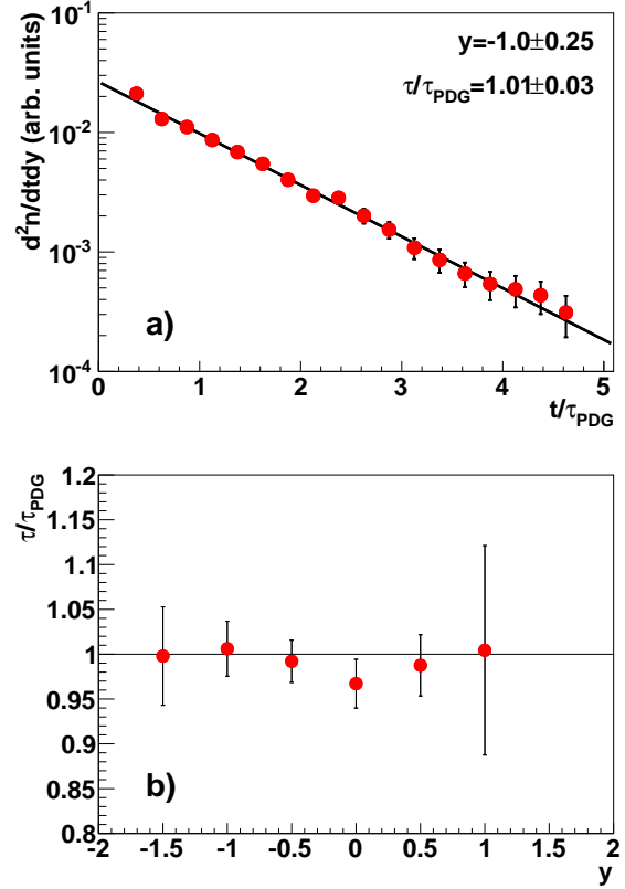
Fig. 10 Top: An example of the corrected proper life-time distribution for \Lambda hyperons produced in inelastic p+p interactions at 158 GeV/c in the rapidity interval y = -1.0 \pm 0.25 . Bottom: The ratio of the fitted mean life-time to its PDG [18] value as a function of rapidity.
