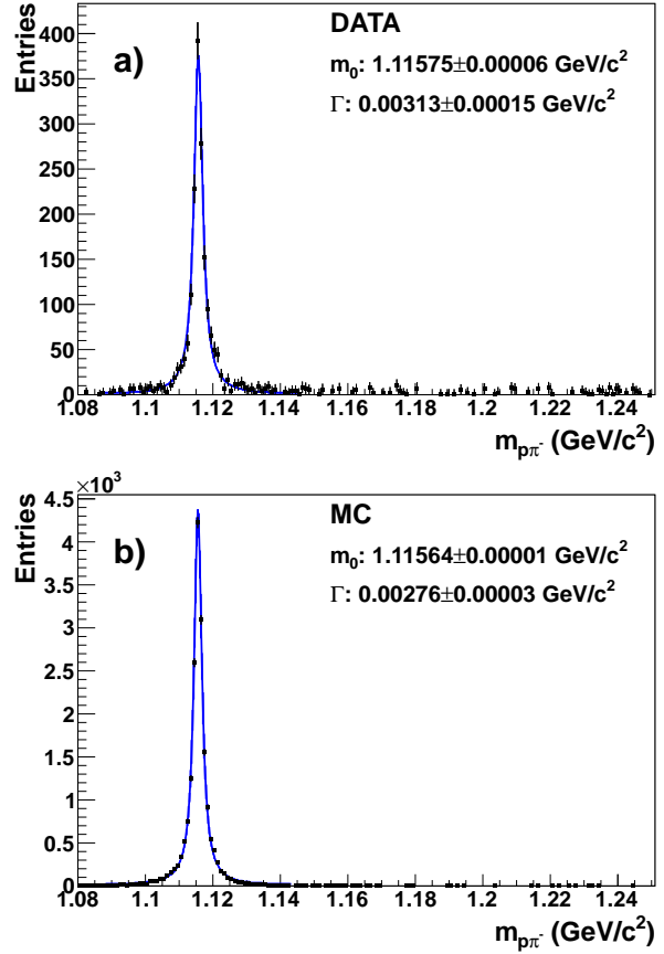
Fig. 7 The invariant mass distribution of \Lambda candidates for y \in [-0.25, 0.25] and p_T \in [0.2, 0.4] GeV/c with the LH inserted after subtraction of the fitted background (a), and for the simulation (b).
