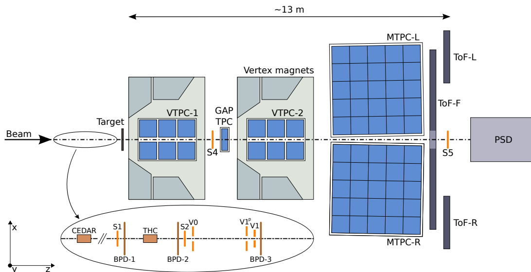
Fig. 1 Schematic layout of the NA61/SHINE experiment at the CERN SPS (horizontal cut in the beam plane, not to scale). The beam and trigger counter configuration used for data taking on p+p interactions in 2009 is presented. The chosen right-handed coordinate system is shown on the plot. The incoming beam direction is along the z axis. The magnetic field bends charged particle trajectories in the x-z (horizontal) plane. The drift direction in the TPCs is along the y (vertical) axis [6]. See details in Section 2.
