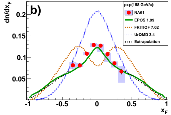
Fig. 20 Comparison of \frac{dn}{dy} (a), and \frac{dn}{dx_F} (b) distributions with calculations of the EPOS [19], UrQMD [34, 35] and FRITIOF [36] models. The chain line was used to extrapolate the NA61/SHINE measurements to full phase space. For details see text.
