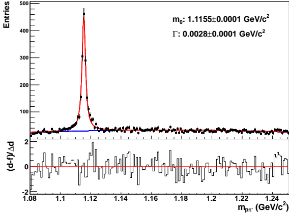
Fig. 6 The invariant mass distribution of \Lambda candidates for y \in [-0.75, -0.25] and p_T \in [0.2, 0.4] GeV/c is shown in the upper plot (LH inserted). The solid line shows a fit to signal plus background, while the dashed line represents the background contribution. The lower part of the plot shows the difference between the data points and the fit, normalised to the statistical error of the data points.
