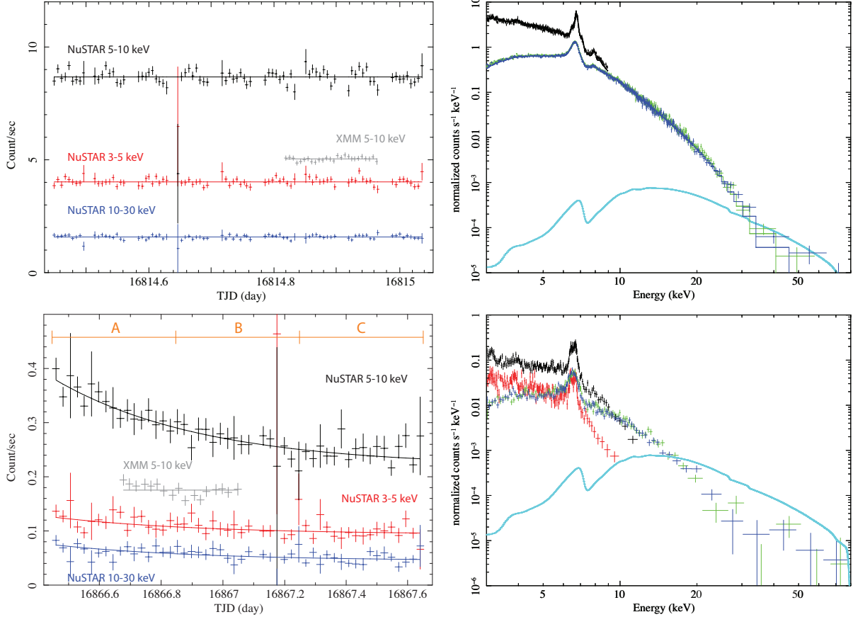
Fig. 3.— Light curves ( left ) and spectra ( right ) of the first ( top ) and second ( bottom ) observations. Left : XMM-Newton /EPIC-pn ( grey , 5–10 keV) and NuSTAR /FPMA+FPMB ( red : 3–5 keV, black : 5–10 keV, blue : 10–30 keV) light curves. Each light curve bin has 500 sec for the first observation and 2000 sec for the second observation, respectively. Right : XMM-Newton /EPIC-pn, MOS1 ( black , red ) and NuSTAR /FPMA, /FPMB ( green , blue ) spectra of \eta Car. The solid lines on the June 6 spectra show the best-fit model in Table 2. The solid cyan line on each panel for spectra shows the power-law component measured from the Suzaku observations (Hamaguchi et al. 2014b), convolved with the NuSTAR /FPMA response. We do not simultaneously fit the XMM-Newton and NuSTAR spectra for July 28 because the NuSTAR spectrum changed significantly during the second observation.
