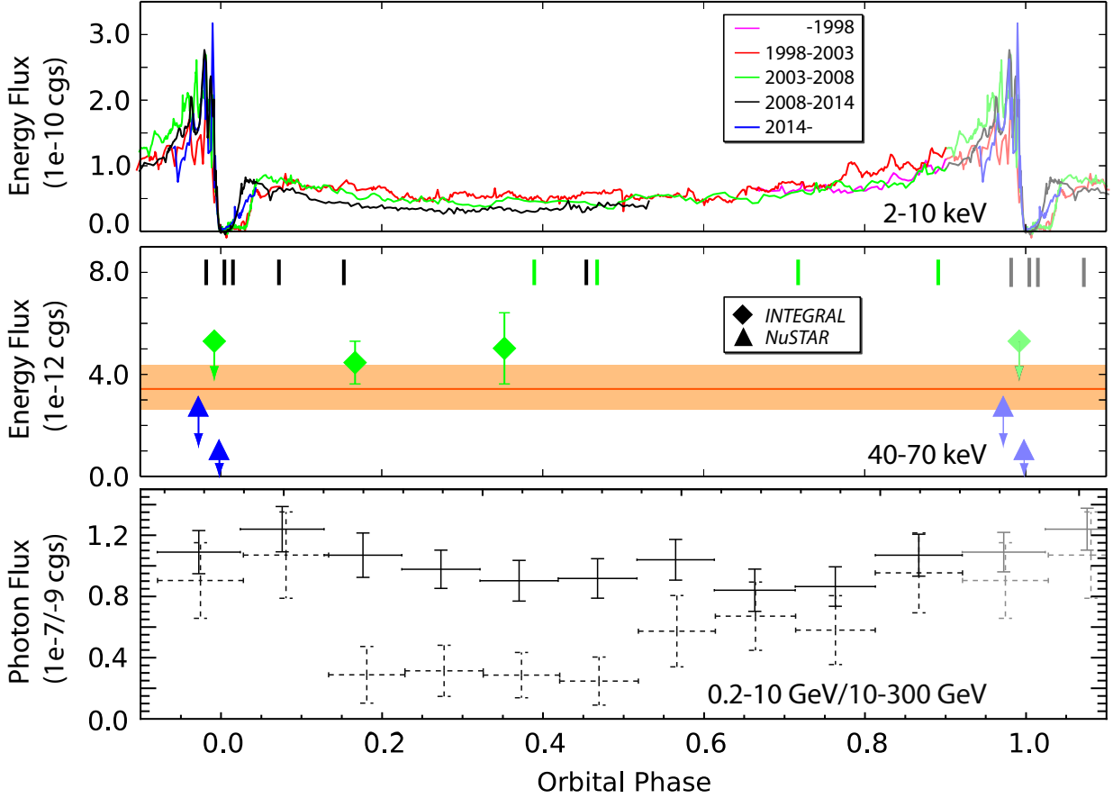
Fig. 6.— X-ray flux between 2–10 keV measured with RXTE and Swift (top: Corcoran et al. 2010, Corcoran et al. in prep.) and between 40–70 keV measured with Suzaku , INTEGRAL , and NuSTAR (middle: Leyder et al. 2008; Hamaguchi et al. 2014b), and 0.2–10 GeV (solid line) and 10–300 GeV (dotted line) \gamma -ray fluxes measured with Fermi (bottom: Reitberger et al. 2015). The orange line and shaded area in the middle panel show the best-fit flux and its 90% error range of the power-law component, derived from the Suzaku HXD/PIN spectra below 40 keV assuming a \Gamma = 1.4 power-law (Hamaguchi et al. 2014b). The multiple vertical bars on the ceiling of the middle panel show the timings of the Suzaku observations used for this spectral fit.
