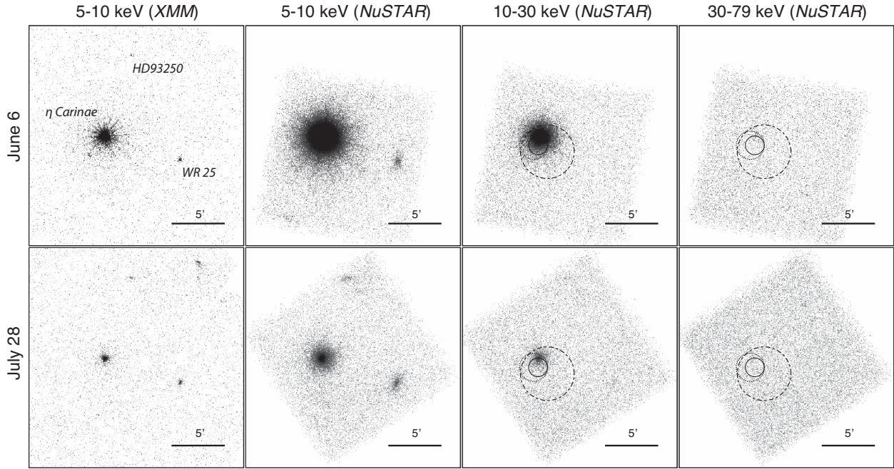
Fig. 2.— XMM-Newton /EPIC-MOS2 (5–10 keV) and NuSTAR /FPMA+FPMB (5–10 keV, 10–30 keV and 30–79 keV) images of the \eta Car field during the first ( top ) and second ( bottom ) observations. The grey scales of all images are adjusted with the event count rate. In the images in the right two columns, the dashed-dot bar circles show the 90% confidence range of the INTEGRAL source (Leyder et al. 2010) and the solid and dotted circles the 95.4% confidence ranges of the Fermi source in the low-energy and high-energy bands, respectively (Reitberger et al. 2015). The EPIC-MOS2 data were not used for the timing and spectral analysis because the \eta Car suffered severe pile-ups.
