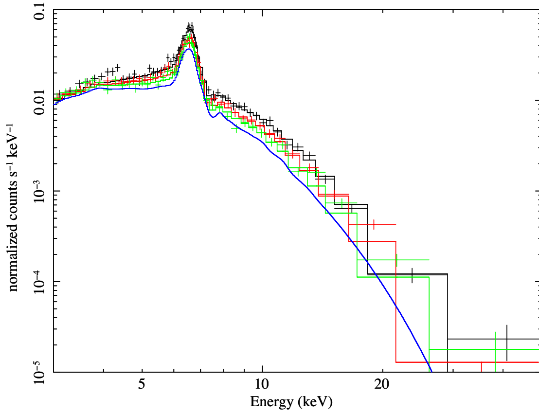
Fig. 5.— NuSTAR /FPMA+FPMB spectra of the second observation in 3 intervals (A: black , B: red , C: green ). The solid blue line shows the deep minimum spectrum, estimated from the Suzaku observation on August 6th and convolved with the NuSTAR response.
