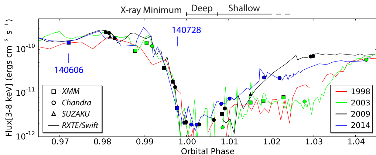
Fig. 1.— RXTE and Swift light curves of \eta Car (Corcoran et al. 2015, in prep.) and the pointed observations (Hamaguchi et al. 2014a, Hamaguchi et al., in prep.). The designations, 140606 and 140728, are timings of the coordinated observations of XMM-Newton and NuSTAR . The horizontal axis shows the orbital phase defined by Corcoran (2005). The phase 1.0 corresponds to 2014 August 2 7:00:29 UT in this cycle.
