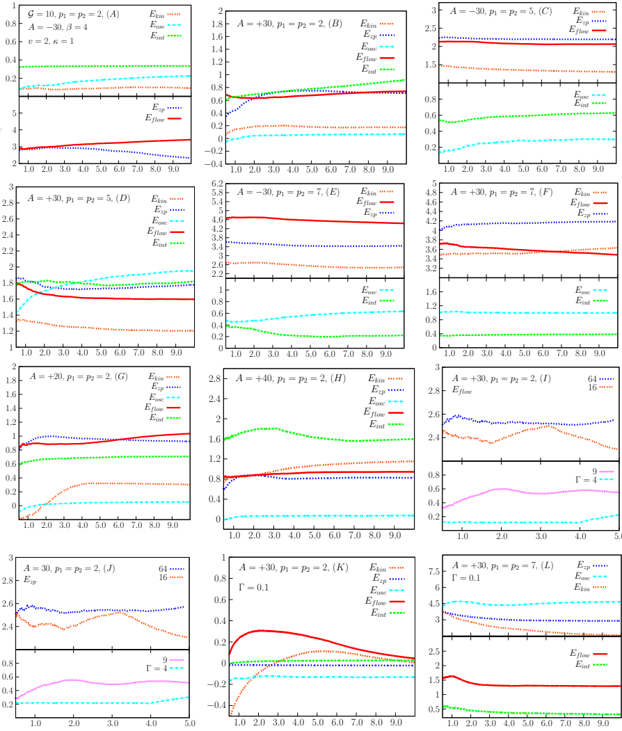
FIG. 14: (Color online) Lyapunov exponents for the energy dynamics of all the previous systems in Figs. 1–3 as a function of evolution time. Energy is along the y -axis and time along the x -axis. G = 10 , v = 2 , \beta = 4 and \kappa = 1 . Frame (A): A = -30 , p_1 = p_2 = 2 ; (B) +30 , 2; (C) -30 , 5; (D) +30 , 5; (E) -30 , 7; (F) +30 , 7; (G) 20, 2; (H) +40 , 2. Frames (I) and (J) display the effects of increasing the relative Planck's constant \Gamma for A = +30 and p_1 = p_2 = 2 . Dotted line: \Gamma = 64 ; triple-dotted line: 16; fine-dotted line: 9; and dashed-dotted line: 4. Frames (K) and (L) display the reduced quantum effects with \Gamma = 0.1 . Frame (K) A = +30 , p_1 = p_2 = 2 ; (L) +30 , 7. Frames (A–H), (K), and (L) all have the same labels although the locations of the observables in the frames tend to vary: triple-dotted line: E_{kin} ; dashed-dotted line: E_{osc} ; dashed line: E_{int} ; dotted line: E_{zp} ; solid line: E_{flow} . The time is in units of 10^4 .
