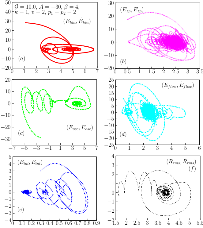
FIG. 10: (Color online) As in Fig. 9; but for A = -30 (system in Fig. 1[(i) and (j)]).
