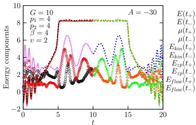
FIG. 5: (Color online) Checking for the presence of physical or numerical chaos in the Crank–Nicolson code applied in this work. The figure shows forward and backward evolving properties of a trapped BEC excited by an RDLP. The system is the same as in Fig. 1 for A = -30 ; except for p_1 = p_2 = 4 . The \pm subscripts in the labels are for forward/backward evolution in time: Thick solid line: total energy E(t_+) ; dashed line: E(t_-) ; double-dotted line: chemical potential \mu(t_+) ; triple-dotted line \mu(t_-) ; fine-dotted line: kinetic energy E_{kin}(t_+) ; dotted line: E_{kin}(t_-) ; open circles: zero-point energy E_{zp}(t_+) ; open triangles E_{zp}(t_-) ; diamonds: kinetic flow energy E_{flow}(t_+) ; and crosses: E_{flow}(t_-) . In this figure, the time at which time reversal begins is t_0 = 10 (see text); to the left of t_0 , the properties are evolving forward in time t , whereas to the right of t_0 , the time axis is for t = 2t_0 - t' , where t' is decreasing as the properties are evolving backward in time. Lengths and energies are in units of the trap, a_{ho} and \hbar\omega_{ho} , respectively. A is in units of \hbar\omega_{ho} , \mathcal{G} in (\sqrt{2}a_{ho}^2)^{-1} , v in a_{ho} , \beta in (a_{ho})^{-2} , and t = \tau\omega_{ho} is unitless.
