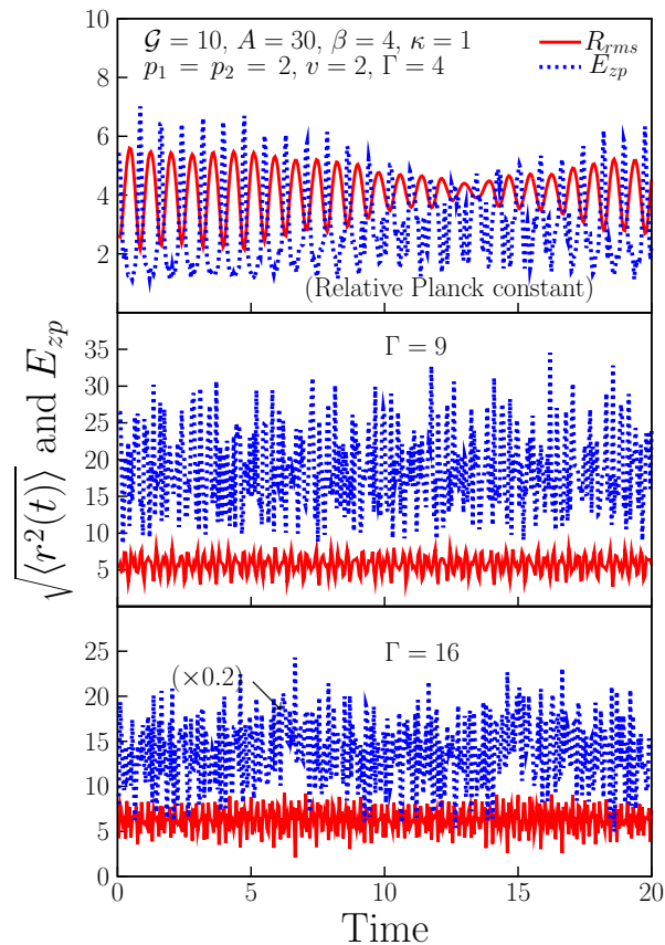
FIG. 3: (Color online) Quantum effects on the dynamics of a trapped Bose gas. The system is the same as in Fig. 1 for A = +30 ; but with increased relative constant \Gamma . The solid line is R_{rms}(t) = \sqrt{\langle r^2(t) \rangle} and the dashed line E_{zp}(t) . Top frame: \Gamma = 4 ; middle frame: 9; and bottom frame: 16. In the bottom frame E_{zp}(t) is reduced by a multiplicative factor of 0.2 to make R_{rms}(t) visible and not to clutter the figure. R_{rms}(t) is in units a_{ho} , E_{zp}(t) in \hbar\omega_{ho}/\sqrt{\Gamma} (see text), A in \hbar\omega_{ho}/\sqrt{\Gamma} , \mathcal{G} in (\sqrt{2}a_{ho}^2)^{-1} , v in a_{ho} , \beta in (a_{ho})^{-2} , and t = \tau\omega_{ho}/\sqrt{\Gamma} and \kappa are unitless.
