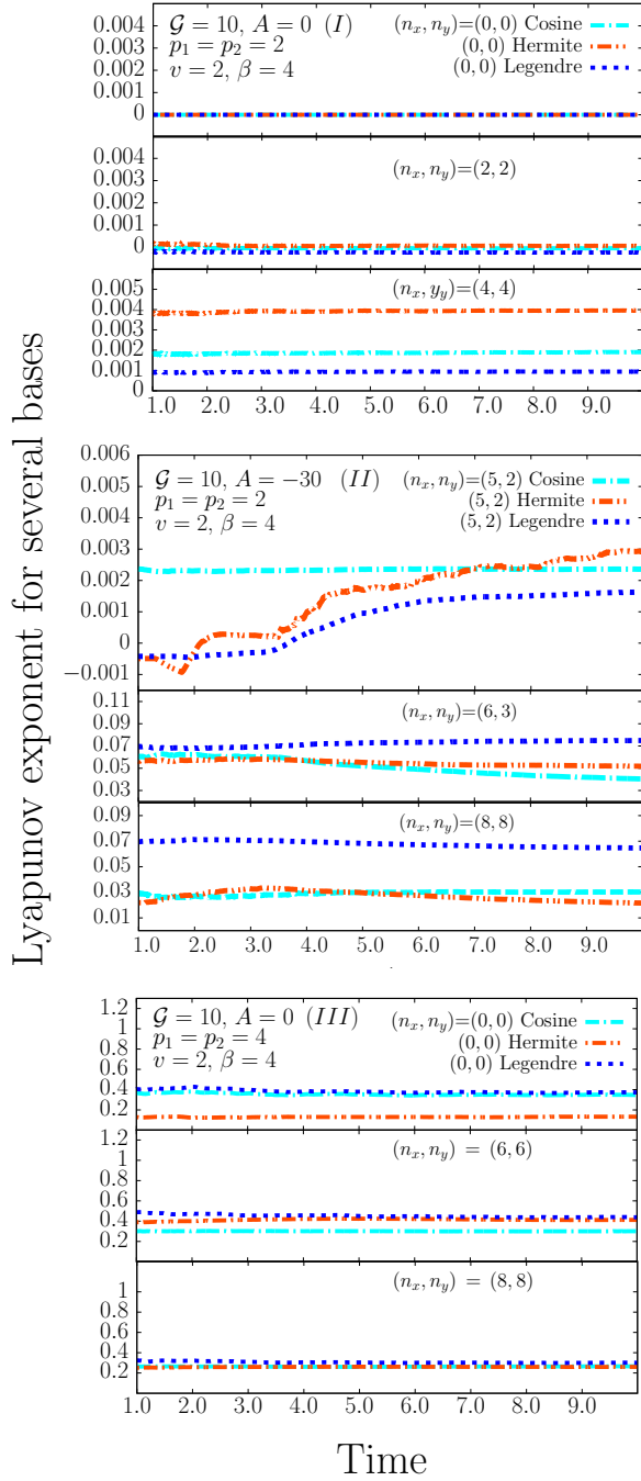
FIG. 7: (Color online) Lyapunov exponents of the weights |C_{n_x, n_y}(t)| [Eq. (15)] for different bases used in the expansion of the total wavefunction. The x -axis is the time t in units of 10^4 . The system is in principle that of Fig. 1. Frame (I) is for A = 0 and p_1 = p_2 = 2 . Dashed-dotted line: Cosine basis; dashed double-dotted line: Hermite; and dotted line: Legendre. Top subframe: state (n_x, n_y) = (0, 0) ; middle: (2, 2) ; and bottom: (4, 4) . Frame (II) is for A = -30 and p_1 = p_2 = 2 . Legends are the same as in (I). Top frame: (5, 2) ; middle: (6, 3) ; bottom: (8, 8) . Frame (III) is for A = 0 and p_1 = p_2 = 4 . Legends are again as above. Top subframe: (0, 0) ; middle: (6, 6) ; and bottom: (8, 8) . A is in units of \hbar\omega_{ho} , \mathcal{G} in (\sqrt{2}a_{ho}^2)^{-1} ; \beta in (a_{ho}^{-2}) ; and t = \tau\omega_{ho} is unitless.
