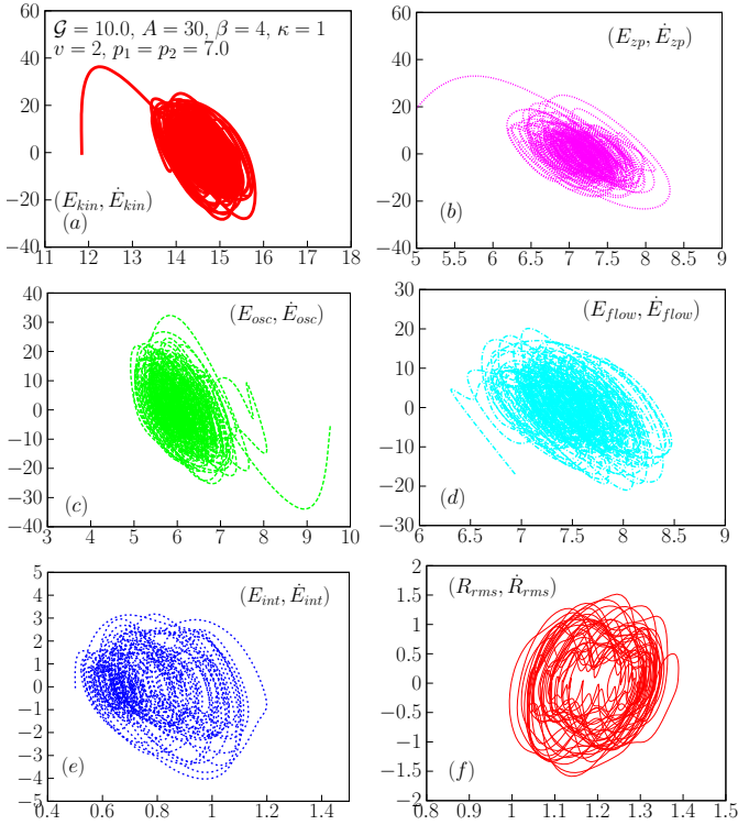
FIG. 11: (Color online) As in Fig. 9; but for p_1 = p_2 = 7 (system in Fig. 2 [frames (e) and (f)]).
