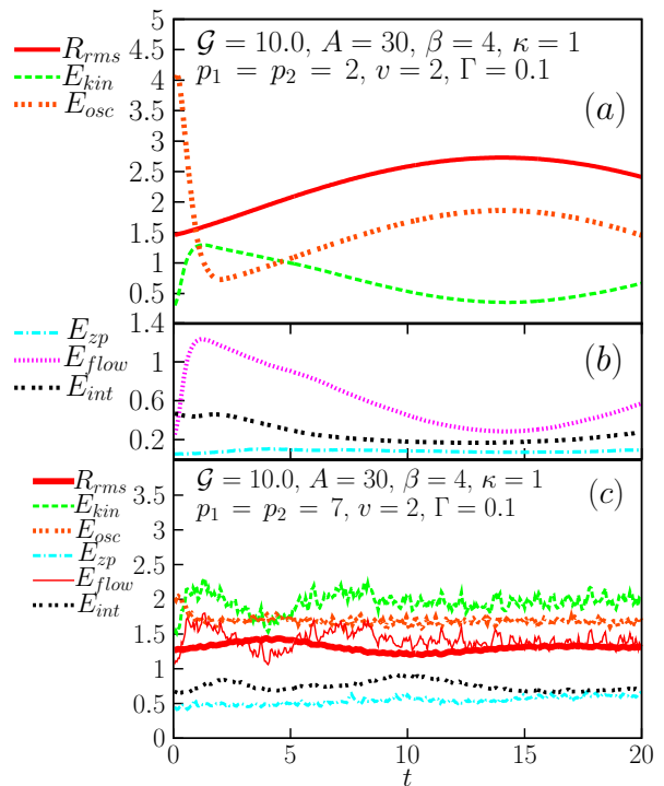
FIG. 4: (Color online) Frames (a) and (b): Dynamics of the harmonically trapped system in Fig. 1 at A = +30 for an artificially reduced relative constant \Gamma = 0.1 . Solid line: R_{rms}(t) ; dashed line: E_{kin}(t) ; triple-dotted line: E_{osc}(t) ; dashed-dotted line: E_{zp}(t) ; fine-dashed line: E_{flow}(t) ; double-dotted line: E_{int}(t) . Frame (c) is as in frames (a) and (b); but for the anharmonically trapped system in Fig. 2 [(e) and (f)] with A = +30 . Thick solid line: R_{rms}(t) ; dashed line: E_{kin}(t) ; triple-dotted line: E_{osc}(t) ; dashed-dotted line: E_{zp}(t) ; thin solid line: E_{flow}(t) ; and double-dotted line: E_{int}(t) . Lengths and energies are in units of the trap a_{ho} and \hbar\omega_{ho}/\sqrt{\Gamma} , respectively. A is in units of \hbar\omega_{ho}/\sqrt{\Gamma} , \mathcal{G} in (\sqrt{2}a_{ho}^2)^{-1} , v in a_{ho} , \beta in (a_{ho})^{-2} , and t = \tau\omega_{ho}/\sqrt{\Gamma} and \kappa are unitless.
