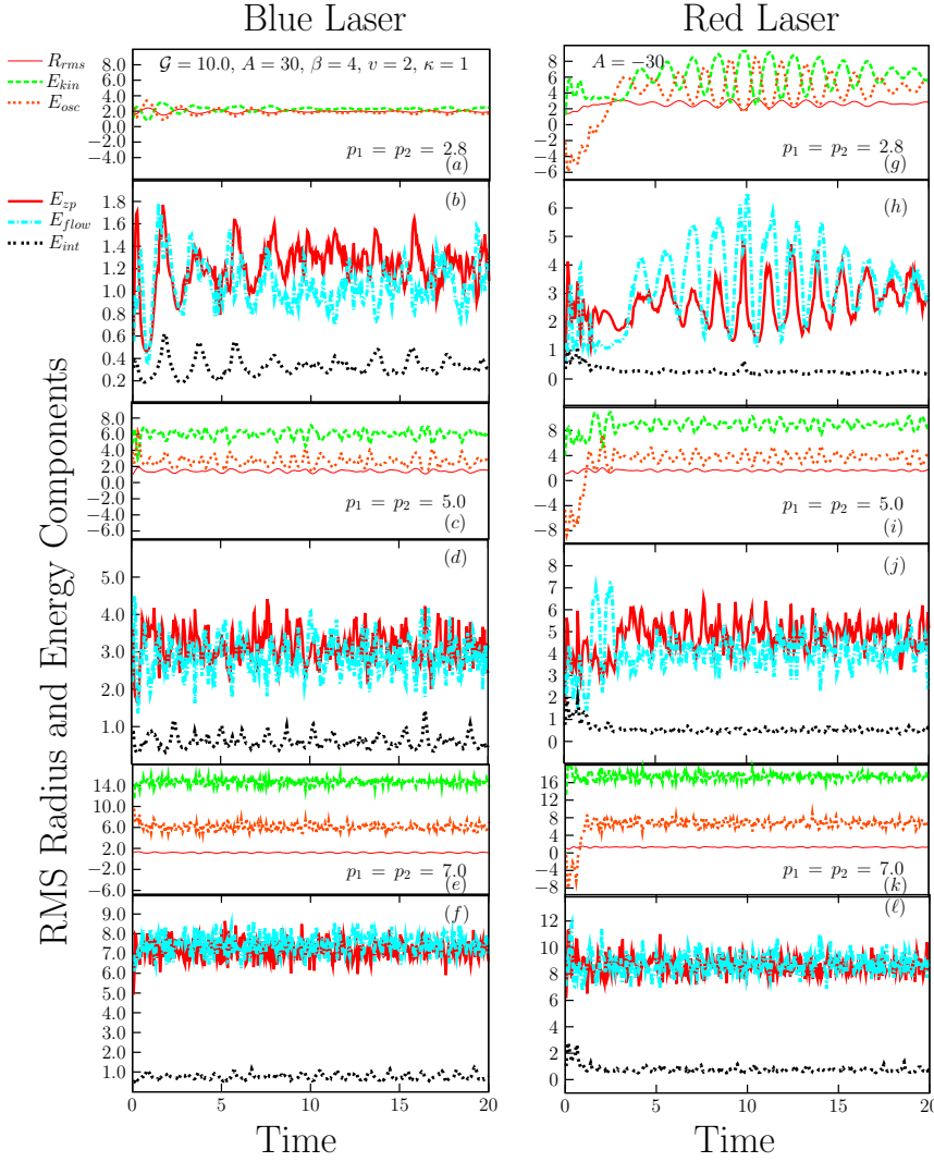
FIG. 2: (Color online) Same as in Fig. 1 with the same labels; but for varying anharmonicities p_1 = p_2 . The interactions are fixed at \mathcal{G} = 10 , the stirrer height is A = 30 in the left column and its depth is A = -30 in the right column. Frames (a),(b),(g),(h): p_1 = p_2 = 2.8 ; (c),(d),(i),(j): 5.0; (e),(f),(k),(l): 7.0. A is in units of \hbar\omega_{ho} , \mathcal{G} in (\sqrt{2}a_{ho}^2)^{-1} , v in a_{ho} , \beta in (a_{ho})^{-2} , and t = \tau\omega_{ho} and \kappa are unitless.
