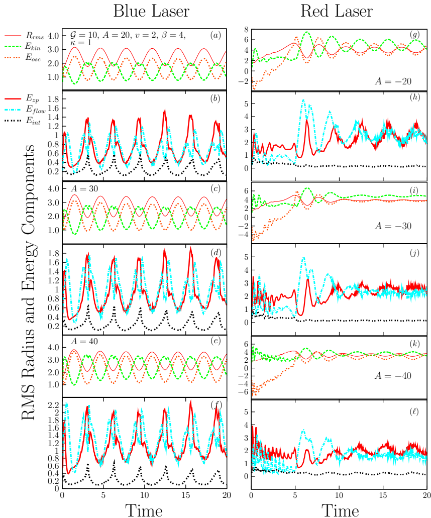
FIG. 1: (Color online) Spatial and energy dynamics of an interacting Bose gas confined by a two-dimensional harmonic trap cut off by a BP [74, 75] and various stirring laser amplitudes A . The side length of the BP is L = 20 such that x \in [-10, 10] and y \in [-10, 10] . The Bose gas is excited by a stirring blue-detuned laser ( A > 0 left column) and a red-detuned laser ( A < 0 right column). The parameters of the system are [74, 75]: \mathcal{G} = 10 , \beta = 4 , v = 2 , p_1 = p_2 = 2 , and \kappa = 1 . A = 20 [frames (a) and (b)], 30 [(c) and (d)], and 40 [(e) and (f)]. A = -20 [(g) and (h)], -30 [(i) and (j)], and -40 [(k) and (l)]. Solid line: R_{rms} ; dashed line: E_{kin} ; triple-dotted line: E_{osc} ; thick solid line: E_{zp} ; dashed-dotted line: E_{flow} ; double-dotted line: E_{int} . A is in units of \hbar\omega_{ho} , \beta in (a_{ho})^{-2} , v in a_{ho} , \mathcal{G} is in (\sqrt{2}a_{ho}^2)^{-1} , R_{rms} in a_{ho} , and energy is in \hbar\omega_{ho} . \kappa and t = \tau\omega_{ho} are unitless.
