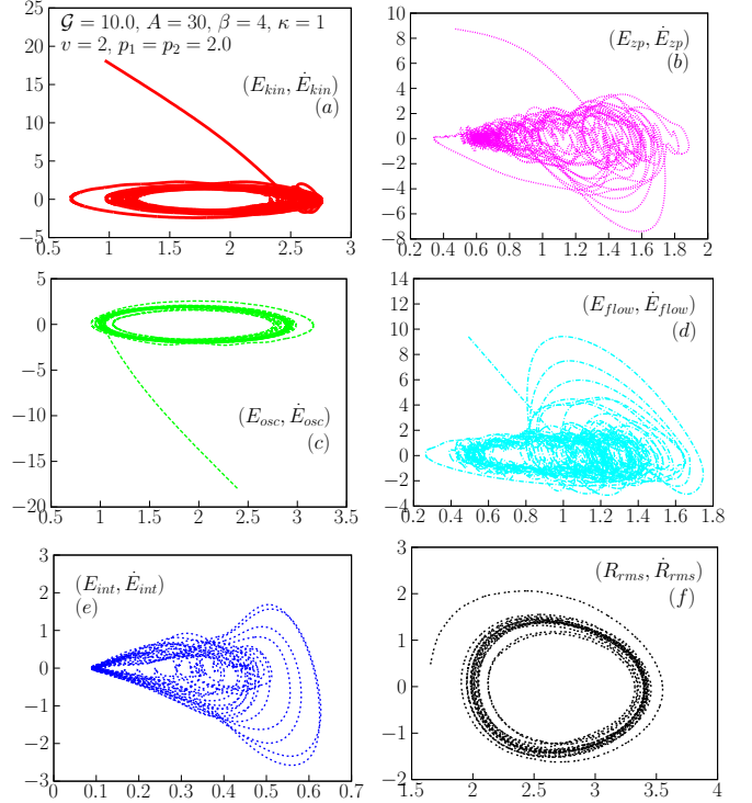
FIG. 9: (Color online) Energy trajectories (E, \dot{E}) of the system in Fig. 1[(c) and (d)] for a time of t = 20 . Frame (a) E = E_{kin} ; (b) E_{zp} ; (c) E_{osc} ; (d) E_{flow} ; (e) E_{int} ; and (f) additionally the phase-space trajectory (R_{rms}, \dot{R}_{rms}) . Lengths and energies are in units of the trap, a_{ho} and \hbar\omega_{ho} , respectively, and t is unitless.
