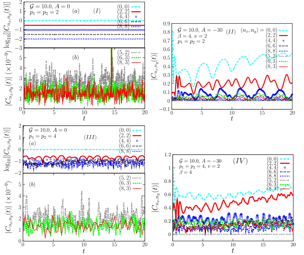
FIG. 6: (Color online) Dynamics of the weights of the harmonic oscillator states, |C_{n_x, n_y}(t)| of Eq. (15). In frame (I), the system is the same as in Fig. 1; but for A = 0 , i.e., no applied laser. Subframe (a) displays \log_{10}[|C_{n_x, n_y}(t)|] : dashed-dotted line: (n_x, n_y) = (0, 0) ; solid line: (2, 2) ; open circles: (4, 4) ; double-dotted line: (6, 6) ; dotted line: (8, 8) . Subframe (b) displays |C_{n_x, n_y}(t)| in units of 10^{-9} : quadro-triple dotted line: (5, 2) ; dashed line: (6, 3) ; and thin solid line: (8, 3) . Frame (II) is the same as (I) with the same labels; but with a laser applied of parameters A = -30 , \beta = 4 , and v = 2 . Frame (III) is the same as (I) with the same labels; but for p_1 = p_2 = 4 . The lower frame (III, b) displays |C_{n_x, n_y}(t)| in units of 10^{-9} . Frame (IV) is the same as (III) with the same labels; but with a laser of depth A = -30 . A is in units of \hbar\omega_{h_o} , \mathcal{G} in (\sqrt{2}a_{h_o}^2)^{-1} , v in a_{h_o} , \beta in (a_{h_o})^{-2} , and t = \tau\omega_{h_o} is unitless.
