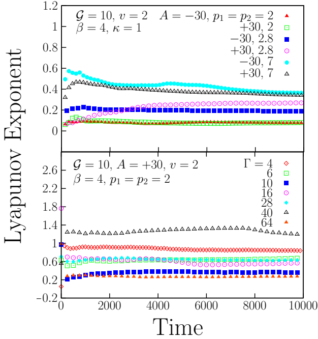
FIG. 8: (Color online) Evolution of the Lyapunov exponent \mathcal{L} for various systems considered from Figs. 1 and 2 after a very long simulation time t = 10000 . The interaction parameter is \mathcal{G} = 10 and the velocity of the stirrer is v = 2 with width parameter \beta = 4 . Upper frame: \mathcal{L} of R_{rms}(t) for various values of A and p_1 = p_2 . Solid triangles: A = -30 , p_1 = p_2 = 2 ; open squares: +30 , 2 ; solid squares: -30 , 2.8 ; open circles: +30 , 2.8 ; solid circles: -30 , 7 ; open triangles: +30 , 7 . Lower frame: \mathcal{L} at various values of \Gamma [cf. Eq.(18)] for A = +30 and p_1 = p_2 = 2 . Open diamonds: \Gamma = 4 ; open squares: 6 ; solid squares: 10 ; open circles: 16 ; solid circles: 28 ; open triangles: 40 ; and solid triangles: 64 . A is in units of \hbar\omega_{ho} , \mathcal{G} in (\sqrt{2}a_{ho}^2)^{-1} , v in a_{ho} , \beta in (a_{ho})^{-2} , and t = \tau\omega_{ho} is unitless.
