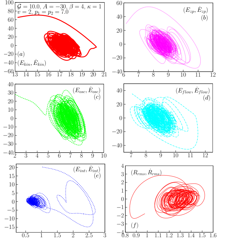
FIG. 12: (Color online) As in Fig. 10; but for p_1 = p_2 = 7 (system in Fig. 2 [frames (k) and (l)]).
