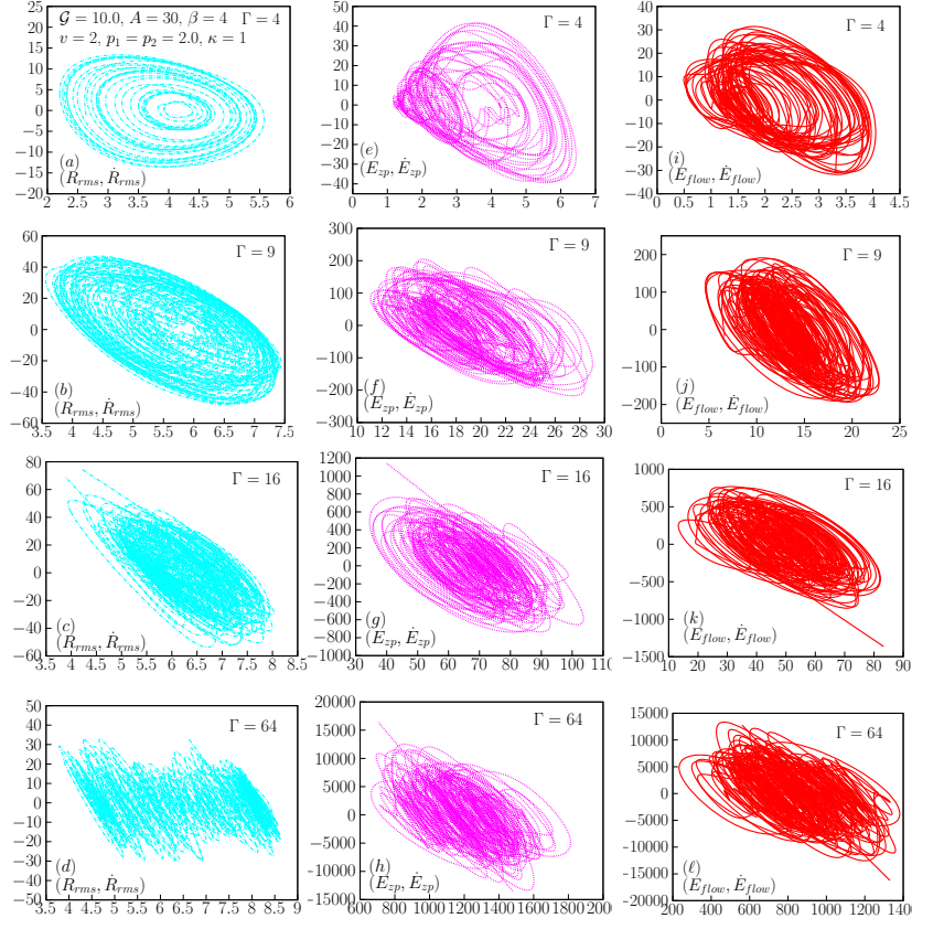
FIG. 13: (Color online) Quantum effects revealed by the phase-space and energy trajectories for the system of Fig. 3. In all frames, the relative Planck's constant \Gamma is increased from top to bottom according to the sequence 4, 9, 16, and 64. Left column [frames (a – d)]: phase-space trajectories ( R_{rms}, \dot{R}_{rms} ); middle column [frames (e – h)]: zero-point energy trajectories ( E_{zp}, \dot{E}_{zp} ); right column [frames (i – l)]: kinetic-flow energy trajectories ( E_{flow}, \dot{E}_{flow} ). R_{rms}(t) is in units of a_{ho} and E_{zp}(t) and E_{flow} are in units of \hbar\omega_{ho}/\sqrt{\Gamma} .
