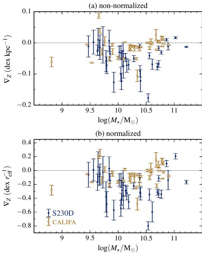
Fig. 3. Slopes of the non-normalized (upper panel) and normalized (lower panel) metallicity gradients of the stellar populations in the disc components as a function of total stellar mass of the simulated galaxies (solid, blue circles). The error bars correspond to a bootstrap errors of the linear regression fits. Observations from the CALIFA survey by Sánchez-Blázquez et al. (2014, open, yellow squares) have been included for comparison.
