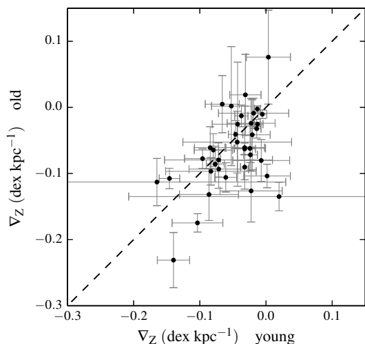
Fig. 8. Slopes of the normalized metallicity profiles of the old stellar population ( > 6 Gyr) versus those of the young stellar population ( < 2 Gyr) for the simulated disc components.
