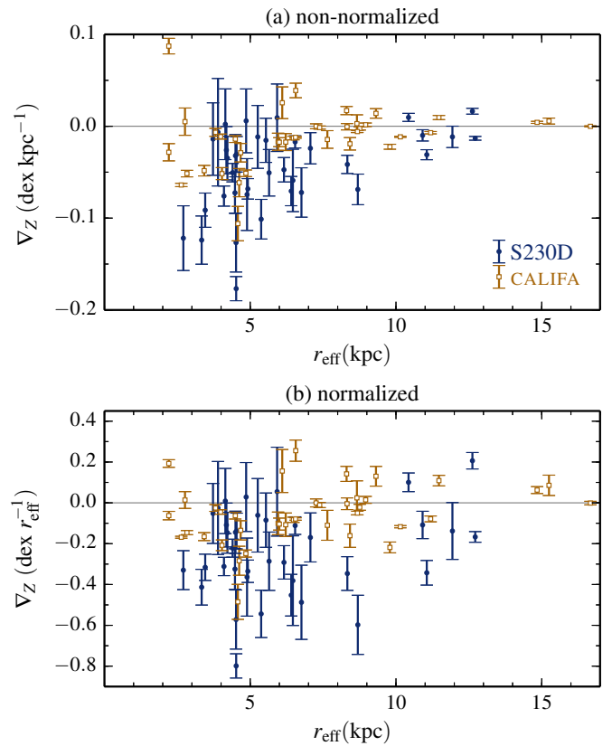
Fig. 4. Slopes of the non-normalized (upper panels) and normalized (lower panels) metallicity gradients of the SPs in the disc components as a function of r_{\text{eff}} (solid, blue circles). The error bars correspond to the bootstrap errors of the linear regression fits.
