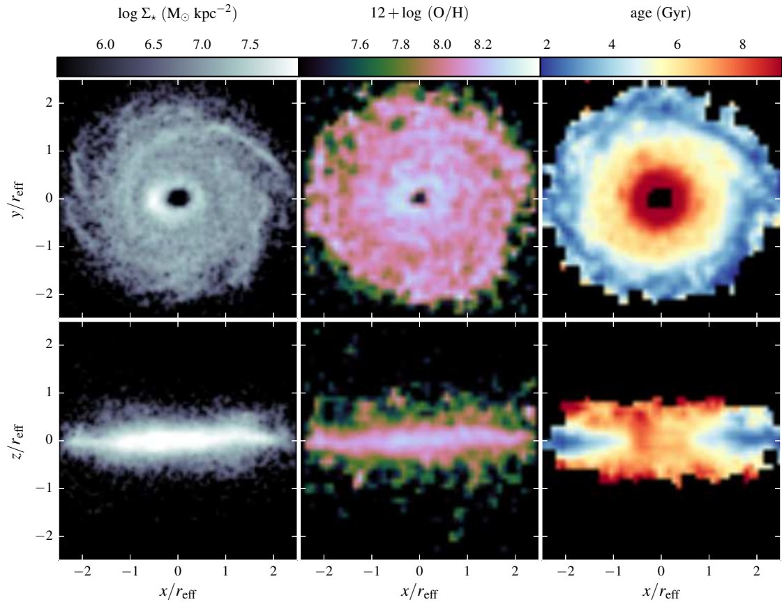
Fig. 1. Surface mass density, oxygen abundance, and ages for the stellar populations in a simulated discs shown for illustration purposes (only stars with \epsilon < 0.5 have been included). Each frame is 5r_{\text{eff}} wide, and the half-mass radius of this stellar disc is r_{\text{eff}} = 11 kpc.
