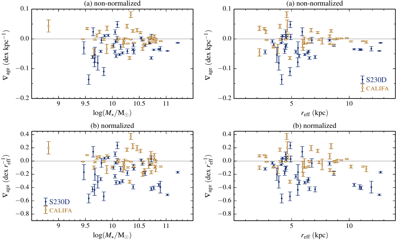
Fig. 6. Slopes of non-normalized (upper panel) and normalized (lower panel) age gradients of the stellar populations as a function of the stellar mass (left panles) and r_{\text{eff}} (right panels) the of the simulated galaxies. Similarly, observations from the CALIFA survey Sánchez-Blázquez et al. (2014, open, yellow squares) have been included for comparison.
