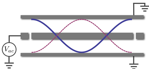
Figure 5. A coplanar waveguide resonator formed by three superconducting lines on a chip. The resonator can be excited via a microwave tone applied to the central conductor, which is intersected by two capacitances that play a similar role as the mirrors in a Fabry-Pérot cavity. The voltage profile of a resonance mode is indicated by the sinusoidal lines.
