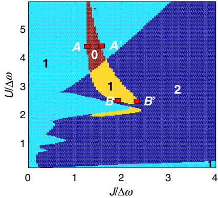
Figure 13. Number of mean-field solutions for \Omega/\Delta = 0.4 , \gamma/\Delta = 0.2 and \Delta > 0 . Note that the notation \Delta\omega = \Delta is used in the axes labels. Reproduced from [153].
