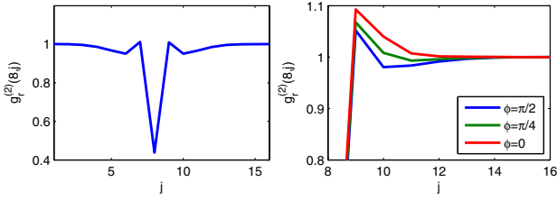
Figure 12. g_{s,j}^{(2)} for \Delta = 0 and U > \Omega > \gamma in a driven-dissipative Bose-Hubbard model. Right plot: Dependence of the correlations on the relative phase between adjacent driving fields. Reproduced from [107].
