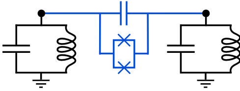
Figure 8. Circuit for a nonlinear coupler that gives rise to cross Kerr interactions as specified in equation (26).
