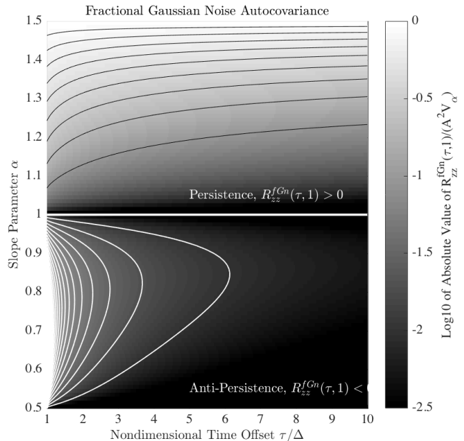
Figure F1. The fractional Gaussian noise autocovariance function R_{zz,1}^{fGn}(\tilde{\tau}) , as defined in (F4), here normalized by dividing by V_\alpha and A^2 . The time axis is interpreted as the normalized time \tilde{\tau} = \tau/\Delta . The shading shows \log_{10} of the magnitude of the normalized autocovariance function, which obtains a maximum of unity at \alpha = 3/2 for all \tilde{\tau} . A sign change occurs at \alpha = 1 , with positive values at higher \alpha and negative values at lower \alpha . Black lines are contours of positive values, with a contour interval of 0.1 beginning at zero, while thin white lines are contours of negative values with an interval of 0.01. The heavy white curve is the zero contour at \alpha = 1 .
