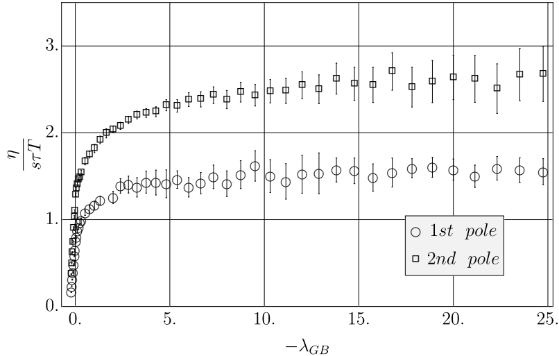
Figure 30: The ratios \eta/sT\tau_k , for k = \{1, 2\} , as functions of \lambda_{GB} in the shear channel of the Gauss-Bonnet theory. Here, \tau_k are defined as \tau_k = 1/|\text{Im}\omega_k| for the two smallest-in-magnitude non-hydrodynamical quasinormal frequencies \omega_k at \mathbf{q} = 0 . The error bars correspond to resolution errors in the \mathfrak{w} -plane.
