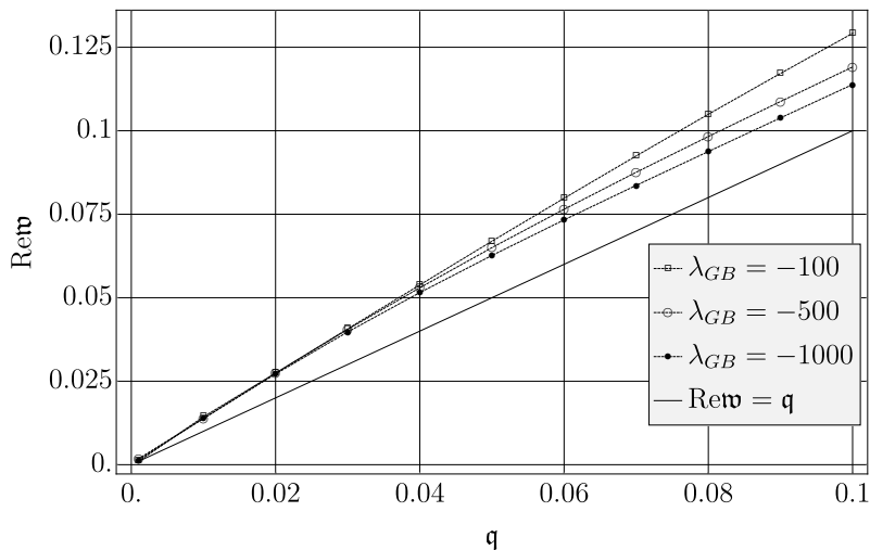
Figure 28: Position of the first pole in the shear spectrum of the Gauss-Bonnet theory, for \lambda_{GB} = \{-100, -500, -1000\} , as a function of momentum \mathfrak{q} . The point indicates where the hypothetical branch cut would begin in the limit of large |\lambda_{GB}| . The solid line corresponds to the expectation of where the position of \text{Re } \mathfrak{w} of the first pole should be in the limit of \lambda_{GB} \rightarrow -\infty , i.e. \text{Re } \mathfrak{w} = \mathfrak{q} .
