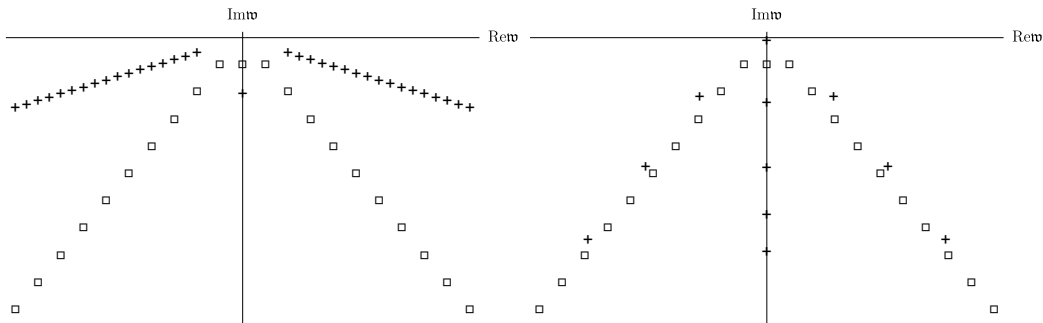
Figure 4: Singularities of thermal two-point correlation function of the energy-momentum tensor in the shear channel in the complex frequency plane at large coupling at \eta/s > \hbar/4\pi k_B (left panel) and at \eta/s < \hbar/4\pi k_B (right panel). Poles at infinitely large coupling are indicated by squares. At large but finite coupling, their new positions are shown by crosses.
