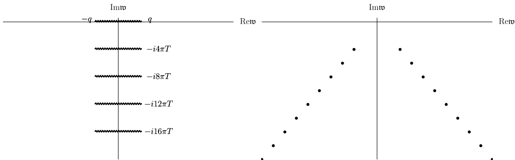
Figure 3: Singularities of a thermal two-point correlation function in the complex frequency plane at (vanishingly) small [61] (left panel) and infinitely large [60] (right panel) values of the coupling.
