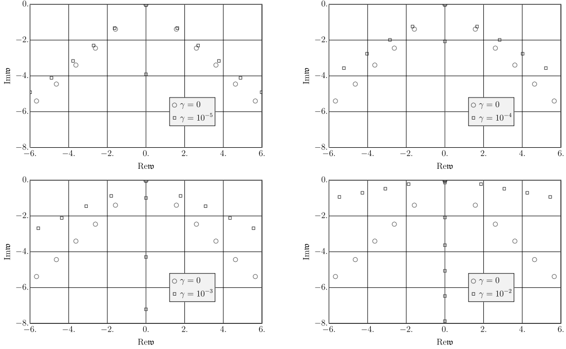
Figure 7: Poles (shown by squares) of the energy-momentum retarded two-point function of \mathcal{N} = 4 SYM in the shear channel, for various values of the coupling constant and \mathbf{q} = 0.1 . From top left: \gamma = \{10^{-5}, 10^{-4}, 10^{-3}, 10^{-2}\} corresponding to values of the 't Hooft coupling \lambda \approx \{609, 131, 28, 6\} . Poles at \gamma = 0 ( \lambda \rightarrow \infty ) are shown by circles.
