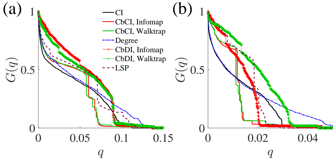
FIG. 3. Normalized size of the LCC, G(q) , plotted against the fraction of removed nodes, q , in two empirical networks. (a) E-mail communication network in Enron. (b) World Wide Web.
