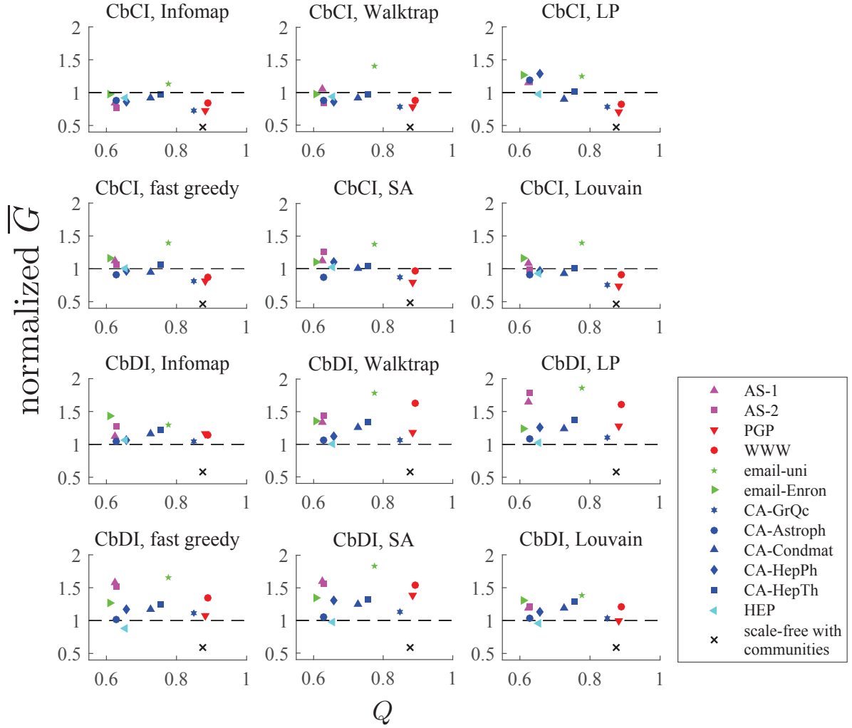
FIG. S4. The normalized size of the LCC averaged over q , i.e., \bar{G} , for the CbCI and CbDI algorithms. The shown values are normalized by those for the CI algorithm. See the caption of Fig. S3 for the legends. The results for Infomap and Walktrap are identical to those shown in Figs. 5(a), (b), (d), and (e).
