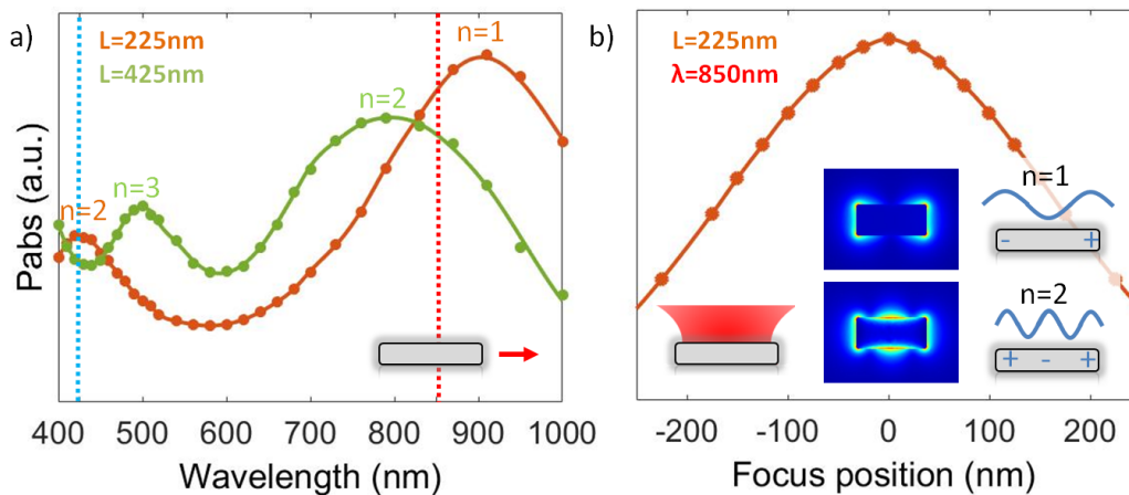
Figure 2: a) Simulated absorption spectra for a 225 nm (orange curve) and a 425 nm (green curve) aluminum nanoantennas excited by an electric point dipole in its vicinity. Plasmonic mode orders n are indicated over each resonance. Red and blue dashed lines indicate excitation and detection wavelengths used for all measurements, respectively. b) Simulated absorption spectra for a 225 nm scanned along its long axis under a focused beam at the fundamental frequency (850 nm). Inset: 2D maps of the scattered electric field norm at the fundamental and harmonic frequencies obtained inside the antenna when the focus of the microscope objective is centered on the antenna. They evidence the n = 1 fundamental and n = 2 excited plasmon modes, respectively. The excitation configurations for the absorption spectra are sketched by a) the red dipole and b) focused beam, respectively.
