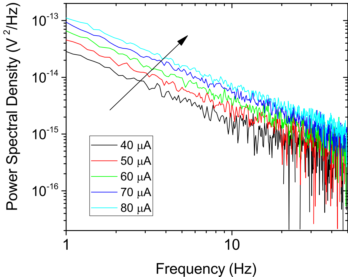
Figure 2. Power spectral density of voltage fluctuations at different dc current flows across H:ZnO nanowire. The arrow indicates the growth direction of dc bias current.
