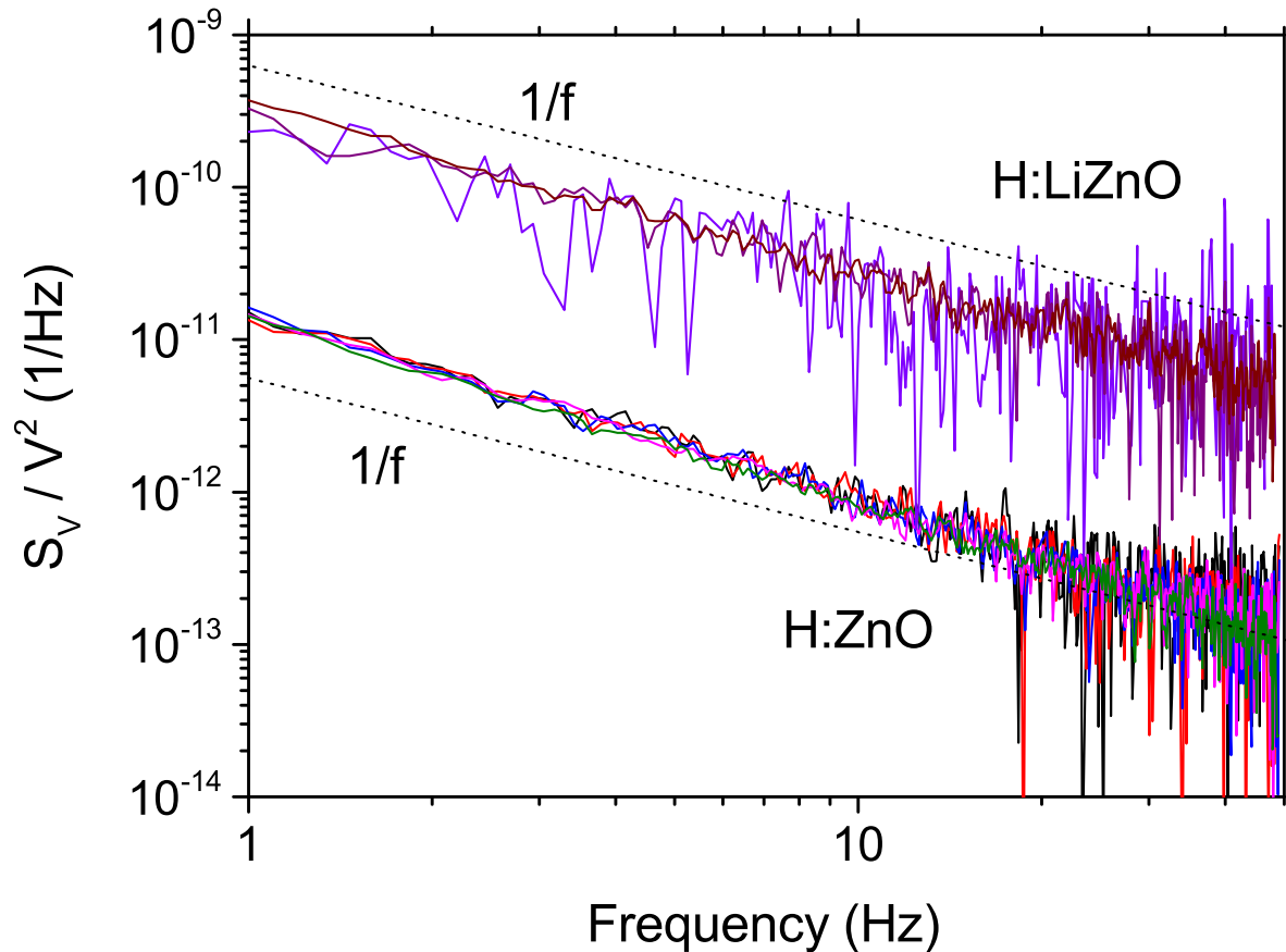
Figure 3. Normalized power spectral density (PSD) of voltage fluctuations for current biased H:ZnO and H:ZnLiO wires. The different colors of the experimental curves mean curves taken at different currents, see e.g. Fig. 2. The dashed lines represent 1/f^a with the spectral exponent a = 1 .
