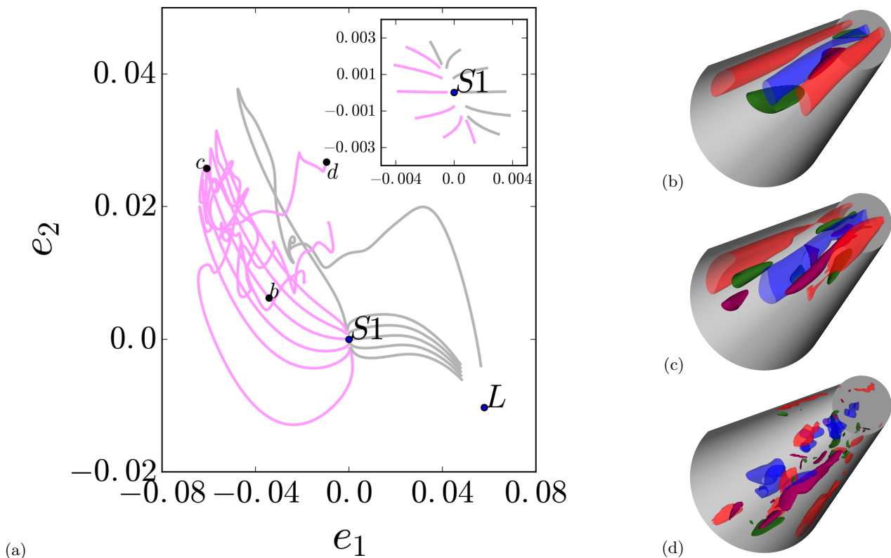
FIG. 4. (a) First approximation to the unstable manifold of S1 , as forward-integrated trajectories with initial conditions (30) visualized as projections onto the local coordinate frame (31). L : Laminar solution. Inset: Same 12 trajectories on the unstable manifold for time interval \tau \in [0, 2.5] , illustrating the initial almost uniform expansion. Isosurfaces of streamwise velocity and vorticity at (b) u = 0.36 (red), u = -0.50 (blue), \omega = \pm 0.99 (green/purple), (c) u = 0.50 (red), u = -0.62 (blue), \omega = \pm 1.5 (green/purple), (d) u = 0.66 (red), u = -0.71 (blue), \omega = \pm 9.0 (green/purple). Flow direction into the page.
