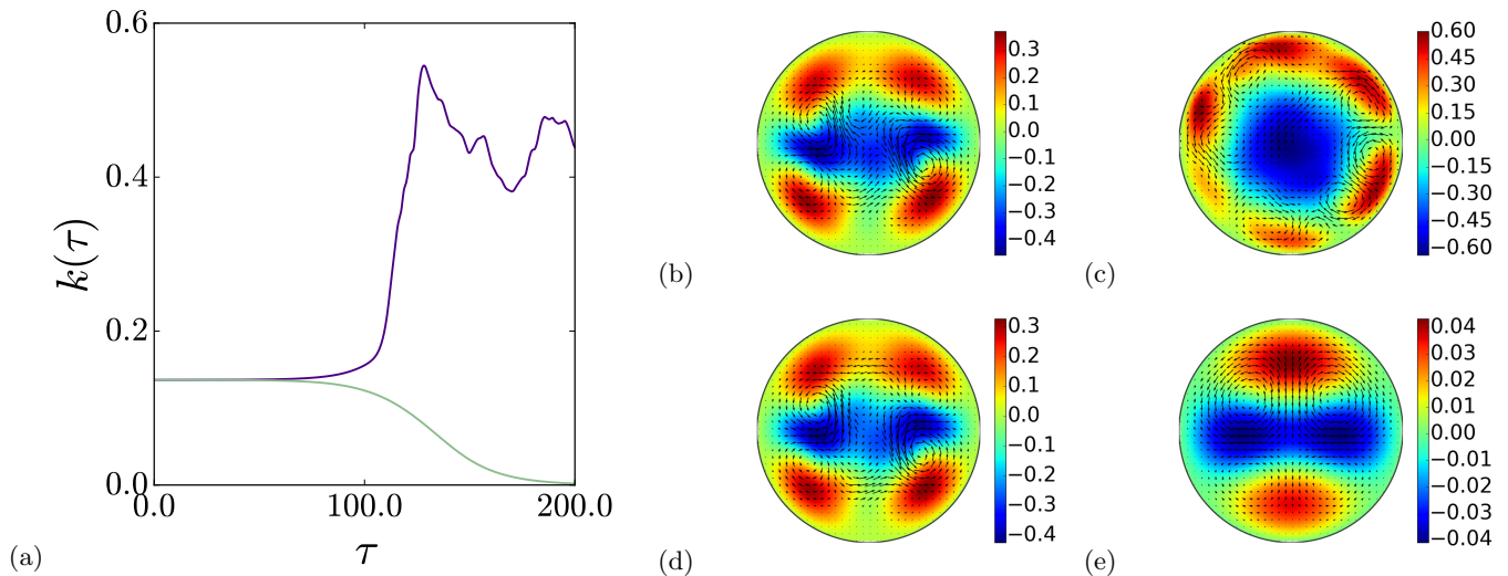
FIG. 9. (a) Time evolution of kinetic energy for trajectories starting from a_{S1N} \pm 10^{-4} V_{11}^{S1N} (green/purple). (b, c, d, e) Color-coded stream-wise velocity and cross-sectional velocity (arrows) averaged over half pipe-length ( z \in [0, L/2] ) at times \tau = 100, 200 respectively on left and right. (b, c) Transition to turbulence (purple on panel a). (d, e) Laminarization (green on panel a).
