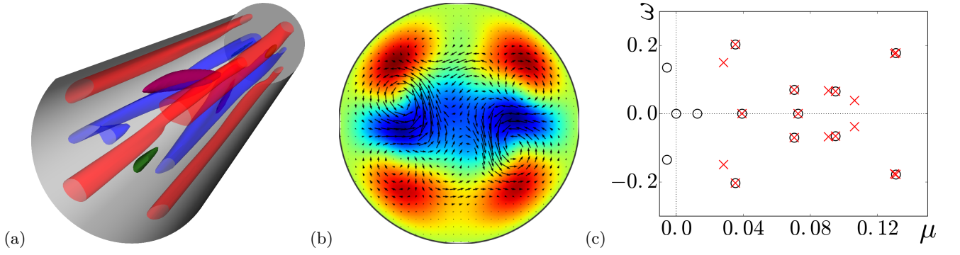
FIG. 7. (a) Isosurfaces of streamwise velocity at u = 0.27 / -0.38 (red / blue) and streamwise vorticity at \omega_z = \pm 0.96 (green / purple) of S1N. (b) Color-coded (fast/slow:red/blue) streamwise velocity and cross-sectional velocity (arrows) averaged over half pipe-length ( z \in [0, L/2] ) visualization of S1N. (c) Leading linear stability eigenvalues of S1N on complex plane computed in shift-and-reflect invariant subspace (black circles) and full state space (red crosses).
