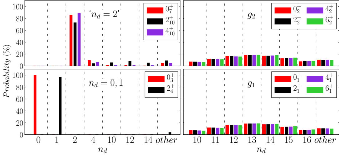
Figure 10. U(5) n_d -decomposition for spherical states (left panels) and for members of the deformed prolate ( g_1 ) and oblate ( g_2 ) ground bands (right panels), eigenstates of \hat{H}' (47) with parameters as in Fig. 9, resulting in spherical-prolate-oblate (S-P-O) shape coexistence. The column ‘other’ depicts a sum of probabilities, each less than 5%.
