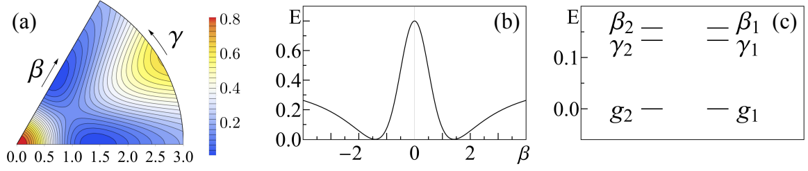
Figure 6. Prolate-oblate (P-O) shape coexistence. (a) Contour plots of the energy surface (38), (b) \gamma = 0 sections, and (c) bandhead spectrum, for the Hamiltonian \hat{H}' (40) with parameters h_0 = 0.2 , h_2 = 0.4 , \eta_3 = 0.571 , \alpha = 0.018 , \rho = 0 and N = 20 .
