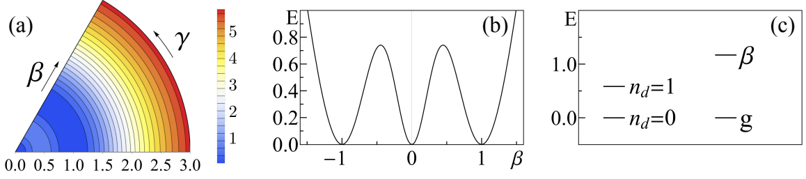
Figure 2. Spherical and \gamma -unstable deformed (S-G) shape coexistence. (a) Contour plots of the \gamma -independent energy surface (30), (b) \gamma=0 sections, and (c) bandhead spectrum, for the Hamiltonian \hat{H}' (32) with parameters r_2=10 , \rho_5=\rho_3=0 and N=20 .
