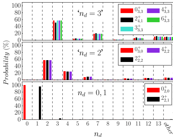
Figure 3. U(5) n_d -decomposition for spherical states, eigenstates of the Hamiltonian \hat{H}' (32) with parameters as in Fig. 2, resulting in spherical and \gamma -unstable deformed (S-G) shape coexistence. The column ‘other’ depicts a sum of probabilities, each less than 5%. The spherical states are dominated by a single n_d component, in marked contrast to the deformed states exhibiting a broad n_d -distribution.
