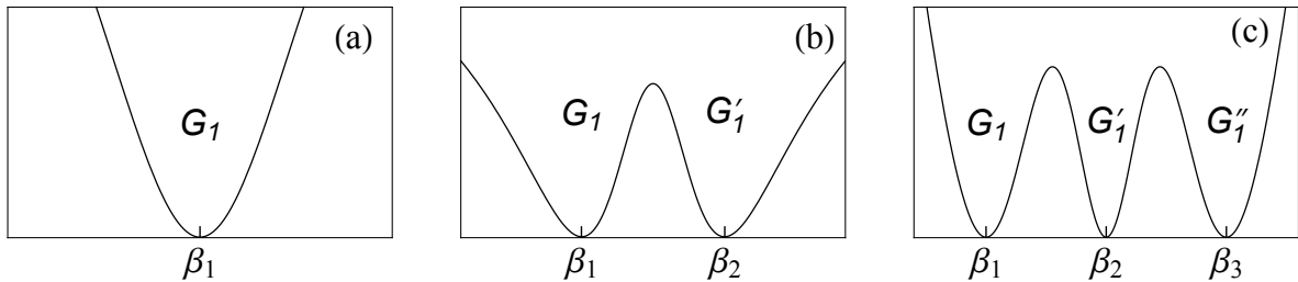
Figure 1. Energy surfaces accommodating: (a) single minimum, (b) double minima, (c) triple minima, associated with (a) G_1 -DS or a single G_1 -PDS, (b) coexisting G_1 -PDS and G'_1 -PDS, (c) coexisting G_1 -PDS, G'_1 -PDS and G''_1 -PDS.
