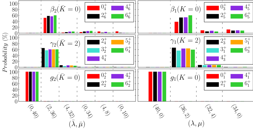
Figure 7. SU(3) (\lambda, \mu) - and \overline{\text{SU}}(3) (\bar{\lambda}, \bar{\mu}) -decompositions for members of the prolate ( g_1, \beta_1, \gamma_1 ) and oblate ( g_2, \beta_2, \gamma_2 ) bands, eigenstates of \hat{H}' (40) with parameters as in Fig. 6, resulting in prolate-oblate (P-O) shape coexistence. Shown are probabilities larger than 5%.
