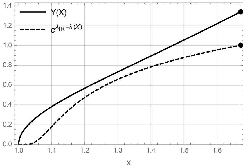
Figure 2: A numerical solution for the functions Y(X) and \lambda(X) in the case p = 5 . Notice that since (5.24) is quadratic in Y , the function -Y is also a solution with \lambda unchanged. The far UV region is at Y = 0 , X = 1 and the IR region where the S^6 smoothly caps off is indicated by the solid dots.
