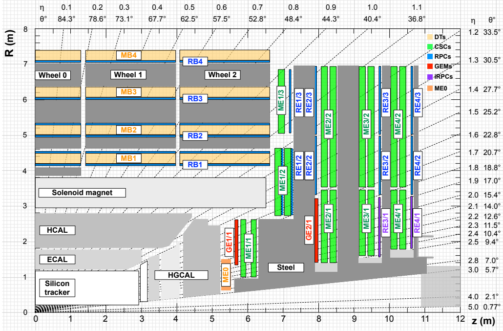
Figure 1. An R - z cross section of a quadrant of the CMS detector, including the Phase-2 upgrades (RE3/1, RE4/1, GE1/1, GE2/1, ME0). The interaction point is at the lower left corner. The acronym iRPCs in the legend refers to the new iRPC chambers RE3/1 and RE4/1. The locations of the various muon stations are shown in color (MB for DTs, ME for CSC, RB and RE for RPC, GE and ME0 for GEM (Gas Electron Multiplier)). M denotes Muon, B stands for Barrel and E for End-cap. The magnet yoke is represented by the dark gray areas.
