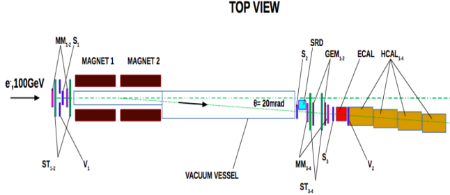
Figure 1: Setup of NA64 for the invisible decay channel search of A' \rightarrow \chi\chi [3].
