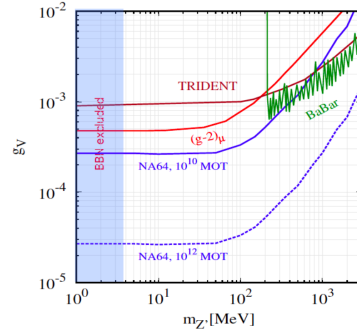
Figure 7: The NA64 \mu projected bounds calculated for 10^{10} and 10^{12} muons on target [13].
