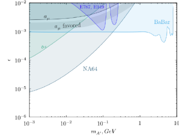
Figure 2: The NA64 90 % C.L. exclusion region in the (M_{A'}, \epsilon) plane [4].
