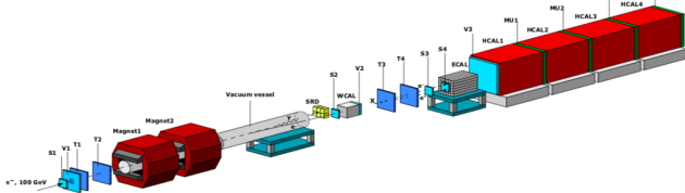
Figure 4: Setup of NA64 for the visible decay channel search of A' , X(17 \text{ MeV}) \rightarrow e^+e^- [7].
