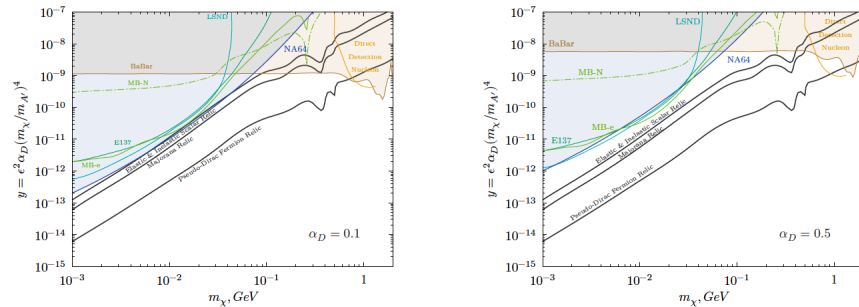
Figure 3: The NA64 sensitivity limits in the (M_\chi, y) plane along-with the limits from other experiments [4].
