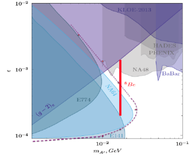
Figure 5: The parameter space for A' , X \rightarrow e^+e^- excluded by the NA64 experiment with the 2017 data (blue shadowed region) and with 2017+2018 data (dashed line). The red vertical line is the region that could explain the ^8\text{Be} anomaly [4].
