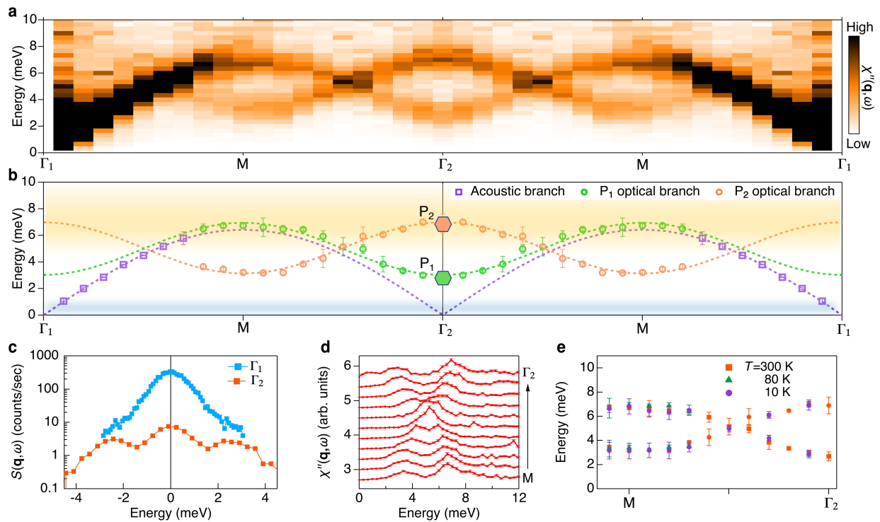
Figure 2 Room temperature phonon excitations in \alpha -RuCl 3 . (a) Low-energy phonon excitations determined by IXS along the \Gamma_1 (6, -3, 0)–M (6, -2.5, 0)– \Gamma_2 (6, -2, 0) direction. The plot shows the Bose-factor corrected IXS intensity. The extracted peak positions are presented in panel (b) revealing interlaced optical phonons intercepting with the transverse acoustic phonon branch. The optical phonon energies at \Gamma_2 are denoted by the green (P 1 ) and orange (P 2 ) hexagons, which are consistent with the phonon modes previously found by THz-spectroscopy 38 . The yellow
