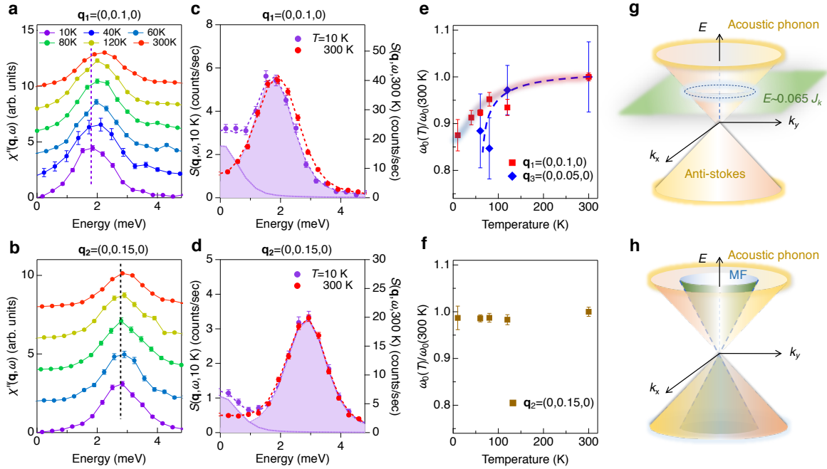
Figure 4 Giant acoustic phonon softening. (a) and (b) show the temperature-dependent \chi''(\mathbf{q}, \omega) at \mathbf{q}_1=(0,0,1,0) in reciprocal lattice units (r.l.u.), \omega \sim 2 meV and \mathbf{q}_2=(0,0,15,0) r.l.u., \omega \sim 3 meV, respectively. (c) direct comparison of the IXS raw data, S(\mathbf{q}_1, \omega) , at T=10 and 300 K. (d) shows
