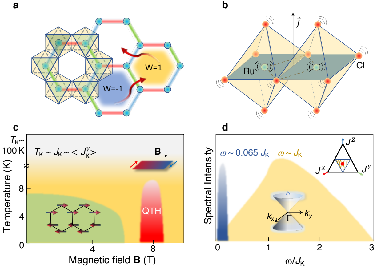
Figure 1 Schematics of a Kitaev-QSL and the phase diagram of \alpha - \text{RuCl}_3 . (a) Structure motif of \alpha - \text{RuCl}_3 based on a honeycomb lattice of edge-sharing Ru-Cl octahedra. The red, green and blue bonds represent three orthogonal Kitaev interactions J_K^{\gamma} . In the pure Kitaev model [Eq. (1)], the low-energy excitations fractionalize into itinerant MFs (red arrows) and anyonic Z_2 flux (blue and yellow hexagons). (b) The nearly 90^\circ Ru-Cl-Ru bonds and the moderate spin-orbit-coupling favor an Ising-type magnetic interaction that is perpendicular to the Ru-Cl-Ru plane highlighted in a blue-green-color. Lattice vibrations perturbatively modify the magnetic interactions, which induce a coupling between phonons and fractional excitations. (c) illustrates the phase diagram of \alpha - \text{RuCl}_3 on a logarithmic-scale: below T_K \sim J_K \sim 8 meV (the yellow area) the thermal Hall conductivity, \kappa_{xy} , becomes finite, indicating a proximate Kitaev-QSL with MF and Z_2 gauge flux.
