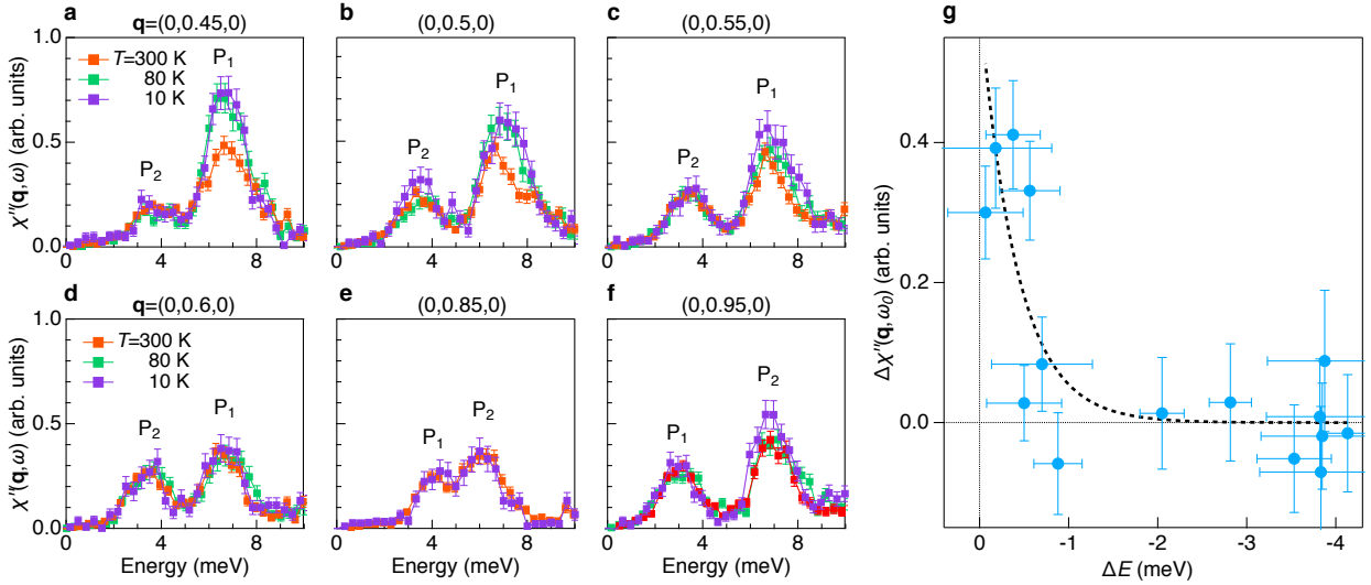
Figure 3 Itinerant MF-phonon coupling near \omega \sim J_K . (a-f) Spectra of the interlaced optical phonons at different reduced momentum transfer \mathbf{q} . Here, we define \mathbf{q}=(0,0,0) and (0,1,0) as \Gamma_1 and \Gamma_2 respectively, where the M point is at \mathbf{q}=(0,0.5,0) . The labels P_1 and P_2 denote the two optical phonon branches. Note the relative peak position of P_1 and P_2 switches at \mathbf{q}=(0,0.75,0) . The
