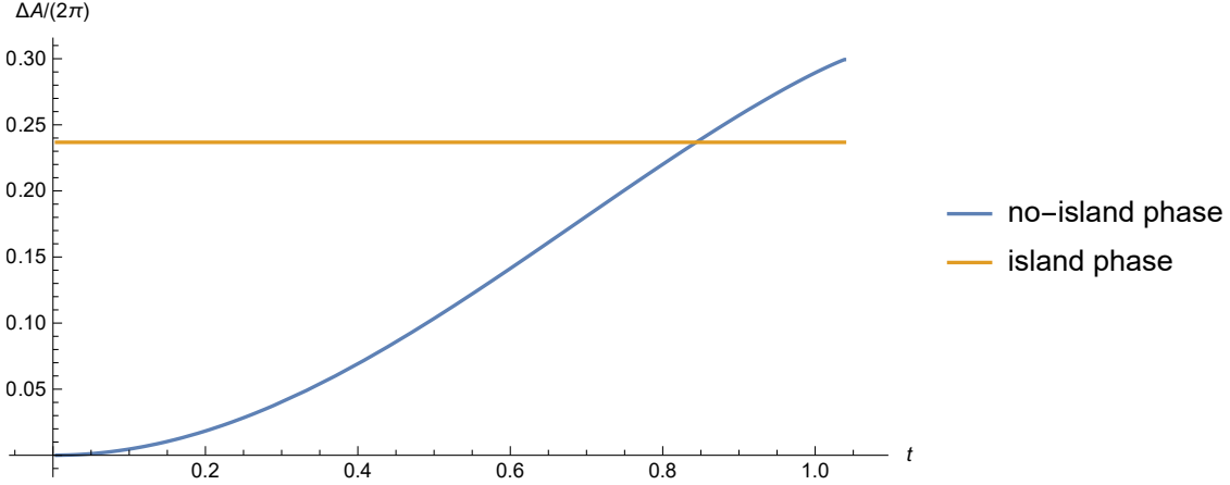
Figure 13: Page curve on codim-2 brane in \text{AdS}_4/\text{dCFT}_3 . Here we define \Delta A = A(t_R) - A(0) , choose z_{\text{bdy}} = 0.95 and use t to label the boundary time t_R = t_L for simplicity. The blue line denotes the area of extremal surface in the no-island phase, which increases with time and is not well-defined after t_m \approx 1.038 . The yellow line denotes the area of extremal surface in the island phase, which is constant and is always well-defined. The holographic entanglement entropy is dominated by the extremal surface with the smaller area. Thus the entanglement entropy first increases with time (blue line) and then becomes a constant (yellow line). In this way, the Page curve of eternal black hole is recovered. Note that the Page time t_P \approx 0.844 is smaller than t_m \approx 1.038 . Thus the unusual situation happens at t_m does not affect the Page curve.
