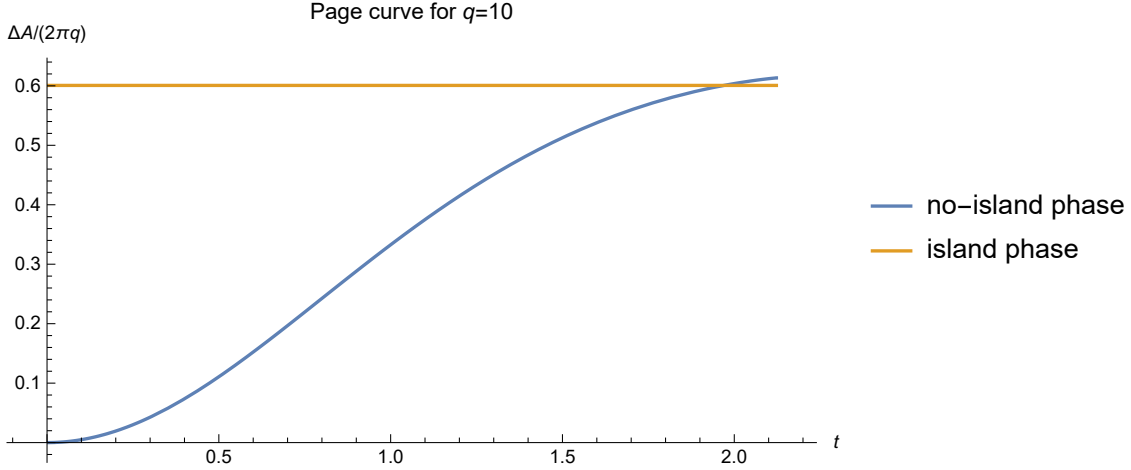
Figure 16: Page curve tensile codim-2 brane with q = 10 and z_{\text{bdy}} = 0.95 in \text{AdS}_4/\text{dCFT}_3 . The blue line and yellow line denote the no-island phase and the island phase, respectively. The Page curve is given by the blue line for t \leq t_P \approx 1.969 , and is given by the yellow line for t > t_P . Since the Page time t_P \approx 1.969 is smaller than the maximum time t_m \approx 2.123 in no-island phase, the unusual situation happens at t_m does not affect the Page curve.
