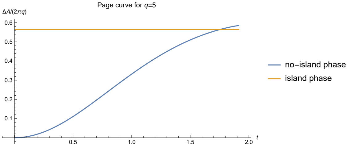
Figure 15: Page curve on tensile codim-2 brane with q = 5 and z_{\text{bdy}} = 0.95 in \text{AdS}_4/\text{dCFT}_3 . The blue line and yellow line denote the no-island phase and the island phase, respectively. The Page curve is given by the blue line for t \leq t_P \approx 1.754 , and is given by the yellow line for t > t_P . Since the Page time t_P \approx 1.754 is smaller than the maximum time t_m \approx 1.914 in no-island phase, the unusual situation happens at t_m does not affect the Page curve.
