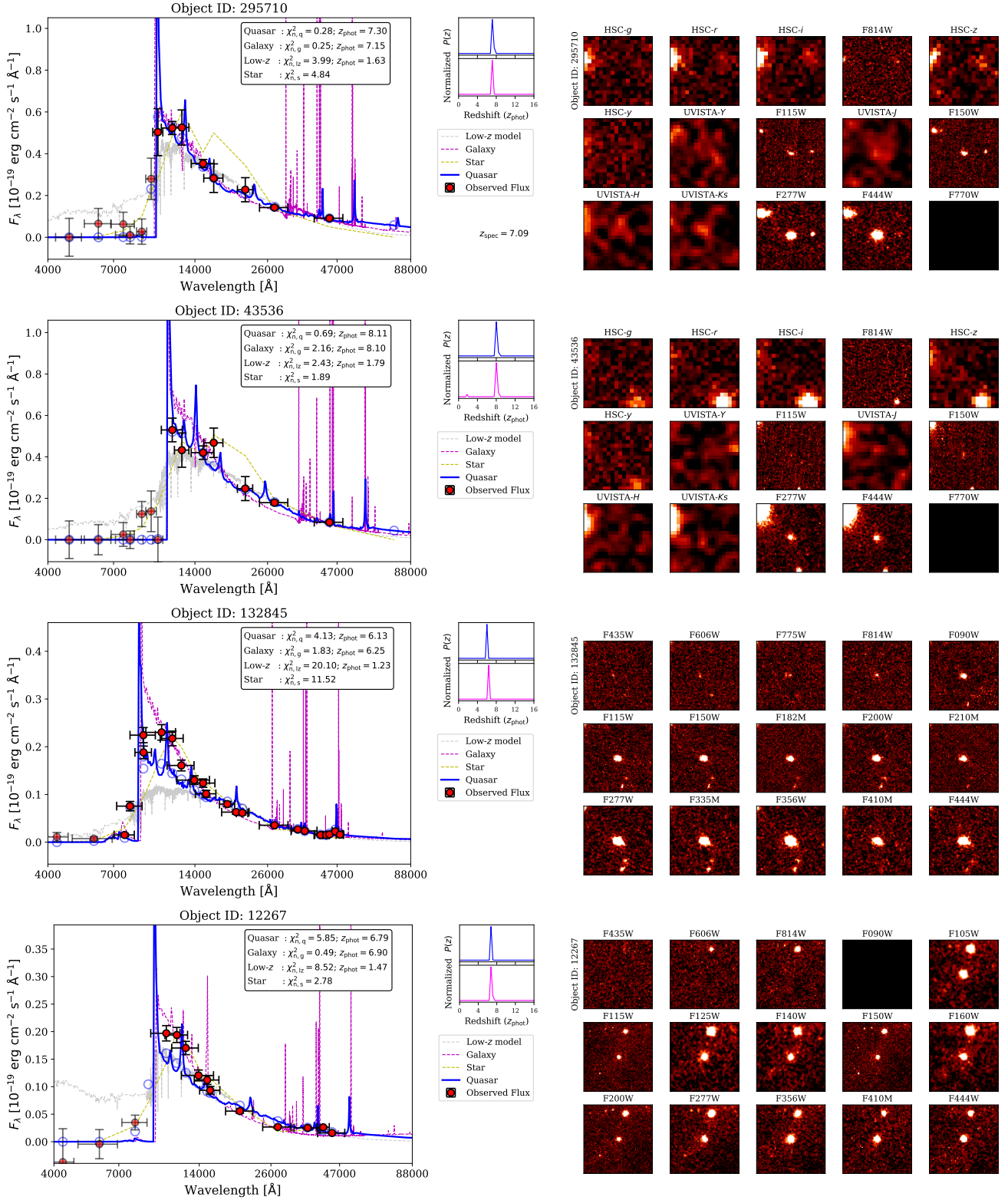
Fig. 1. Photometric SEDs of some quasar candidates. In the left part of each panel, we model the observed photometric data points with four types of spectral templates. Fluxes with S/N > 3 are marked with red circles, while those with lower values are shown with a bit transparent color. The best-fit quasar template and its associated synthetic photometry are presented with blue lines and circles. Models based on the galaxy and star/brown dwarf spectra are shown with magenta and yellow lines, with an additional fitted model of low- z sources displayed in gray color. The goodness-of-fit of each model and the estimated redshift are also reported (see main text for a detailed definition). We further indicate the calculated redshift probability distribution function, P(z) for quasar and galaxy models. Finally, the right part of each panel shows the multiband images of the z \geq 6 quasar candidate, each trimmed to 6'' size on a side.
