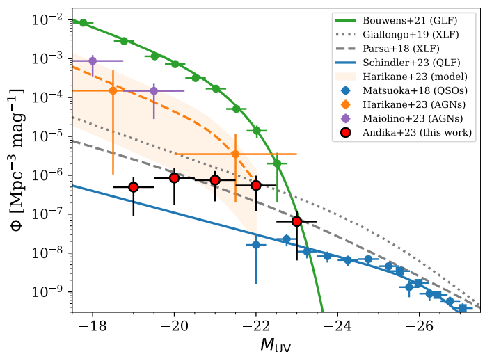
Fig. 5. UV luminosity functions of sources at z \sim 6 . The number densities of our quasar candidates as a function of UV absolute magnitude are marked with red circles with error bars. Blue circles and squares represent the data from Matsuoka et al. (2018) and Schindler et al. (2023), where their associated best-fit quasar luminosity function (QLF) is shown with a blue line. The fitted model and observed galaxy luminosity function (GLF) from Bouwens et al. (2021) are displayed with a green line and circles, respectively. A sample of JWST-confirmed AGNs from Harikane et al. (2023) is designated with orange circles, and their double power-law model, along with its uncertainty, is portrayed with an orange dashed line and shaded region. We also show the AGN luminosity function at z = 4 –6 reported by Maiolino et al. (2023a) with purple circles for comparison. The number density of our quasar candidates is higher than the extrapolation of the brighter QLF. Nevertheless, it is consistent with the X-ray selected AGN luminosity function (XLF) from Parsa et al. (2018) and Giallongo et al. (2019), which are denoted as dashed and dotted grey lines.
