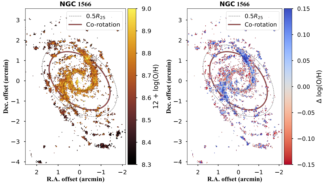
Figure 5. 2D maps of derived 12 + \log(\text{O}/\text{H}) and \Delta\log(\text{O}/\text{H}) of NGC 1566, overplotted with the defined spiral arms from Sec 3.3. The half R_{25} radius is shown as a dashed ellipse while the CR is shown as a solid ellipse. The 12 + \log(\text{O}/\text{H}) and \Delta\log(\text{O}/\text{H}) maps for the remaining sample are presented in Fig B.
