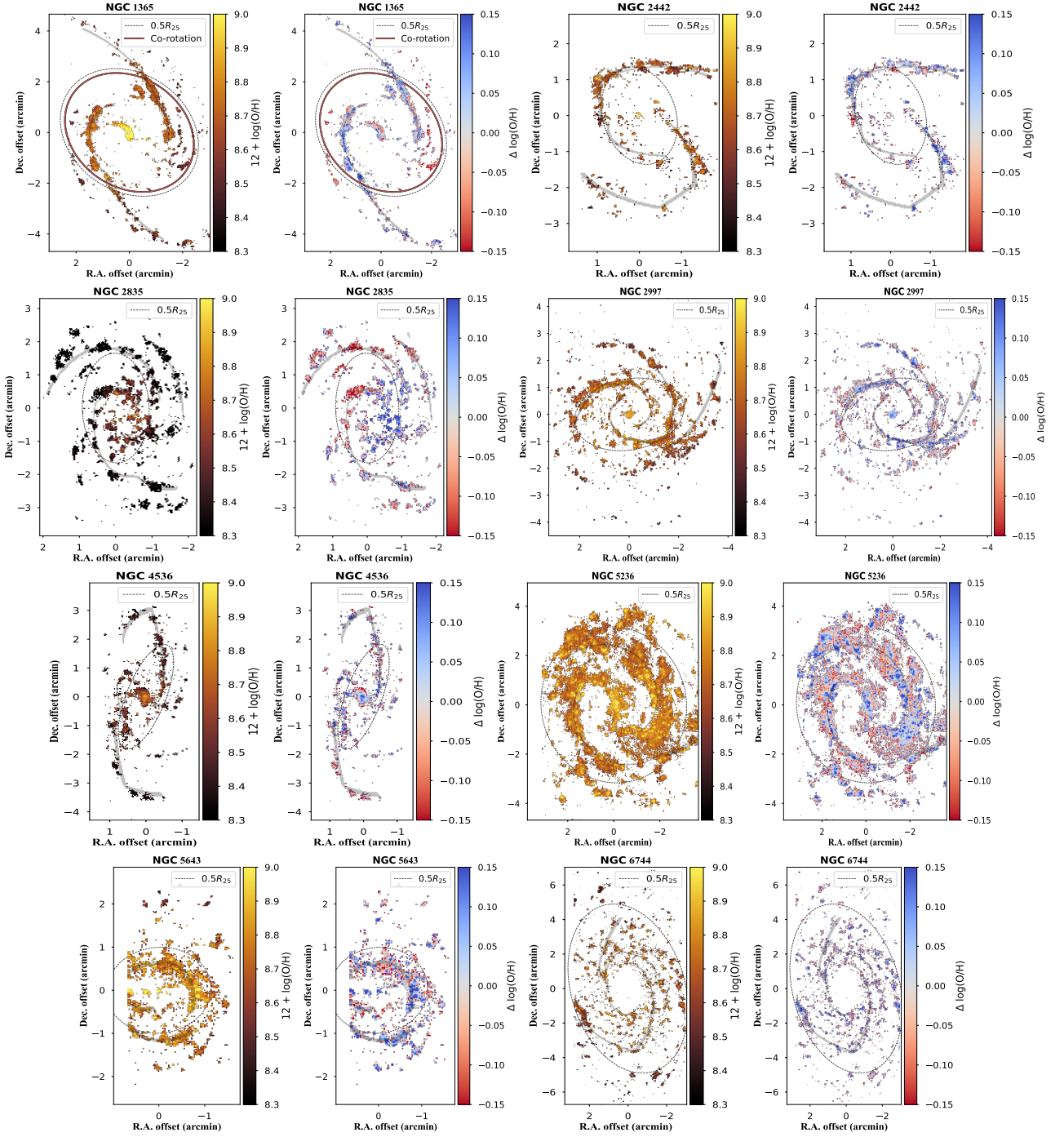
Figure B1. Column 1 & 3: 2D 12 + \log(\text{O}/\text{H}) maps of our galaxies, except for NGC 1566 (Fig 5). Column 2 & 4: Residual of metallicity ( \Delta \log(\text{O}/\text{H}) ) by subtracting the radial gradients. The dashed ellipse marks the location of half R_{25} and the red ellipse denotes the CR, if applicable. More detail on this analysis is in Sec 3.4.
