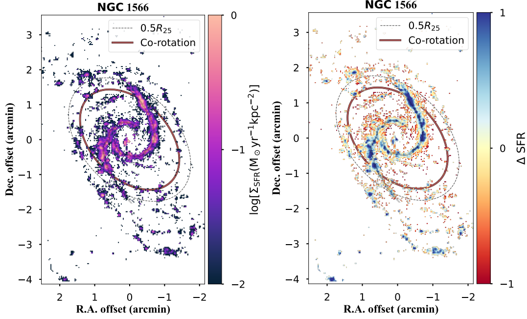
Figure 4. 2D maps of derived \Sigma_{\text{SFR}} and \Delta\Sigma_{\text{SFR}} of NGC 1566 after SNR limit and spaxel selection based on BPT diagram, overplotted with the defined spiral arms from Sec 3.3. The dashed ellipse marks the location of half R_{25} and the red ellipse denotes the co-rotation radius reported in previous publications (see Sec 5.3)
