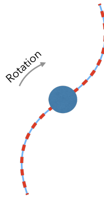
Figure 1. Theoretical expectations from the dynamic spiral theory (left) and density wave theory (right) regarding the location of young (blue) and old (red) stellar populations. The azimuthal offset between young and old stars is predicted by density wave theory but not by dynamic spiral theory, also see Fig 1 in Puerari & Dottori (1997) and Martínez-García et al. (2009). The rotation direction is based on the assumption that the observed spiral arms are trailing features, which will be applied to all spiral galaxies in this work. \Omega refers to the rotational velocity of material while \Omega_p denotes the rotational velocity of the spiral pattern.
