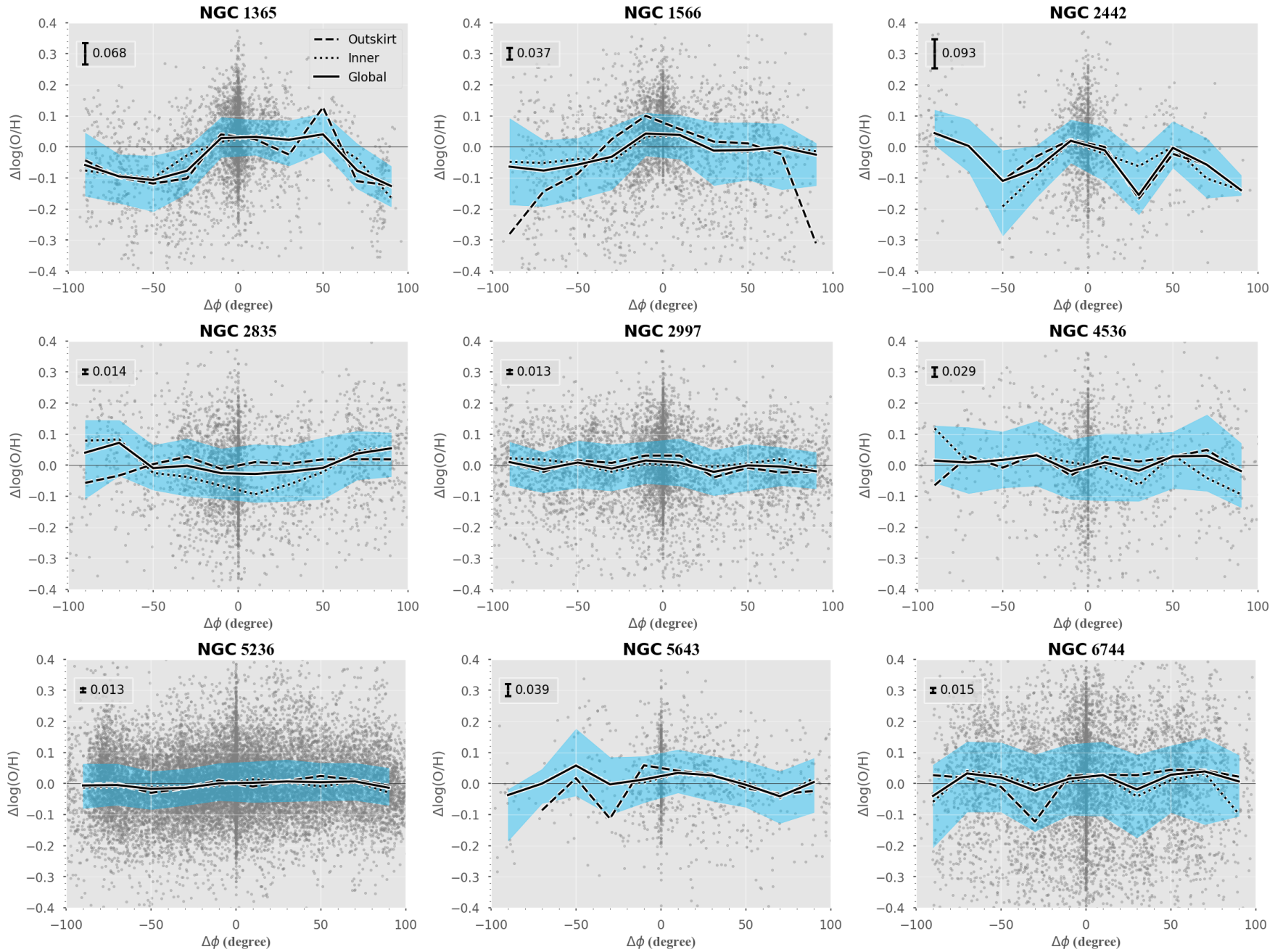
Figure 7. Similar to Fig 6 but for \Delta\log(\text{O}/\text{H}) . The gas flows (leftward) from 100^\circ to 0^\circ then towards -100^\circ . The higher the \Delta\log(\text{O}/\text{H}) is, the more metal-rich the spaxel is, compared to other spaxels at the same galactocentric distance. We find significant offsets ( > 0.1 dex) in the metallicity of NGC 1365 and NGC 1566 and NGC 2442 ( \Delta\phi > 50 ). We find no significant azimuthal variation in the other six spiral galaxies. We do not find any opposite trend of \Delta\log(\text{O}/\text{H})-\Delta\phi in the inner region versus the outskirts. The \Delta\log(\text{O}/\text{H}) in the inner region of NGC 2835 is significantly different from the \Delta\log(\text{O}/\text{H}) in the outskirts, indicative of environmental effects in the outskirts.
