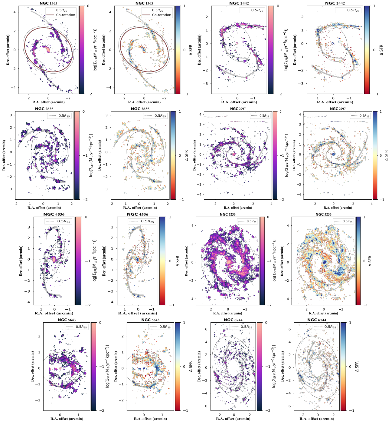
Figure A1. Column 1 & 3: 2D \Sigma_{\text{SFR}} maps of our galaxies, except for NGC 1566 (Fig 4). Column 2 & 4: Residual of \Sigma_{\text{SFR}} by subtracting the radial gradients. More detail on this analysis is in Sec 3.4. The dashed ellipse marks the location of half R_{25} and the red ellipse denotes the CR, if applicable.
