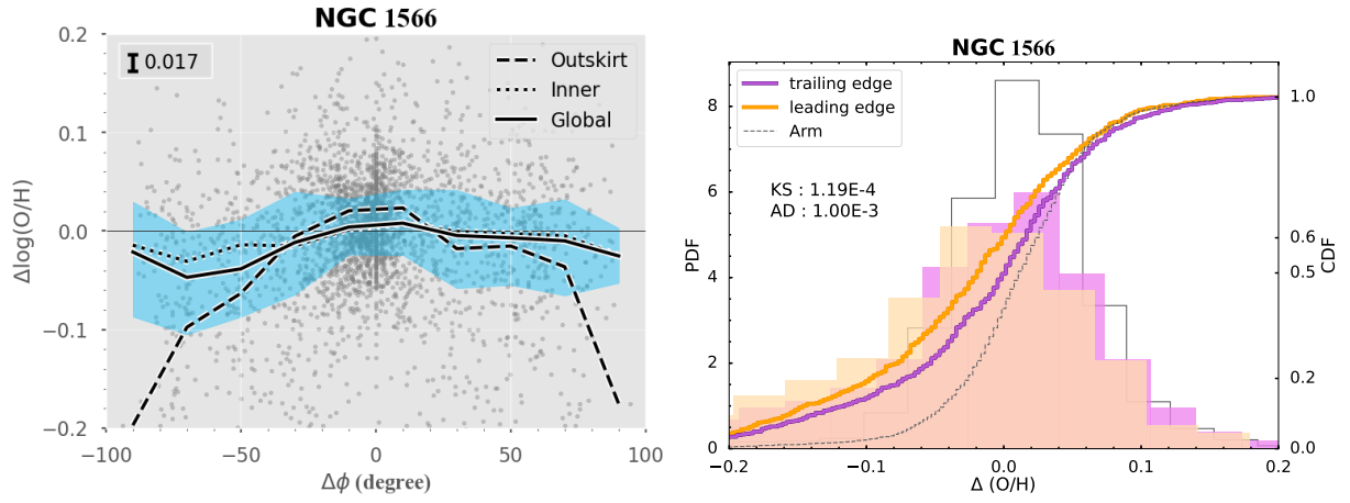
Figure C1. Left: density scatter plot of metallicity residual \Delta \log(\text{O}/\text{H}) versus azimuthal distance to the spiral arms \Delta \phi . \Delta \log(\text{O}/\text{H}) is calculated by subtracting the radial gradient from the S-cal metallicity. \Delta \phi is the same as Fig 3, described in Sec 3.3. We find slightly higher \Delta \log(\text{O}/\text{H}) in the trailing edge ( \Delta \phi > 0 ) than the leading edge ( \Delta \phi < 0 ), similar with the main results using N2S2-N2H \alpha diagnostic (Fig 7). right: comparing the CDFs of \Delta \log(\text{O}/\text{H}) from ScII among the trailing edge, leading edge and spiral arms. The p -value from the KS test and AD test are shown in the upper left. We find higher \Delta \log(\text{O}/\text{H}) in the trailing edge, with a p -value of 1.19 \times 10^{-4} , suggesting that the metallicity on both sides of the spiral arms are drawn from different distributions.
