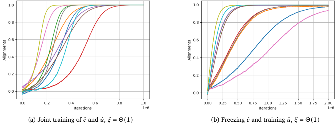
Figure 1: Evolution of \langle u_t, u \rangle during online SGD for 10 random instances with joint and frozen- \hat{c} training. Though time scales differ between (a) and (b), trajectories exhibit similar behavior.
