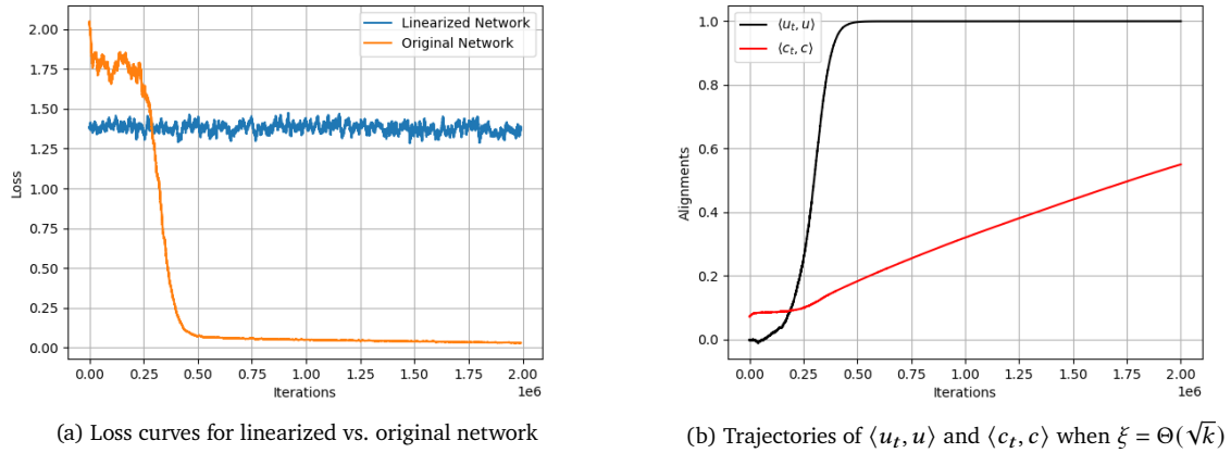
Figure 2: Linearized networks fail in low-rank fine-tuning, and cannot achieve small loss. When jointly training \hat{u} and \hat{c} , we observe incremental behavior in learning, where learning c becomes easier when u is learned to a certain level.
