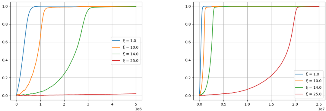
(a) Joint training of \hat{c} and \hat{u} for various choices of \xi (short time-scale) (b) Joint training of \hat{c} and \hat{u} for various choices of \xi (long time-scale)
