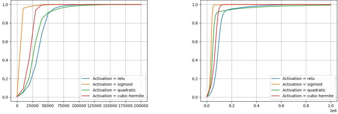
(a) Evolution of overlap \langle u_t, u \rangle for \xi = 1 and different activations
