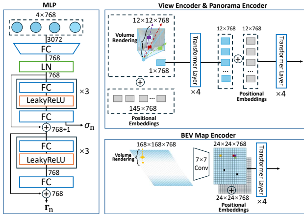
Figure 6. Architecture of modules in the g3D-LF model. FC denotes a fully connected layer, LN denotes layer normalization and LeakyReLU [38] is the activation function.
