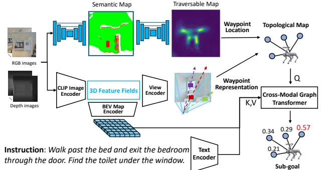
Figure 3. Monocular VLN framework based on VLN-3DFF [58].
