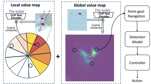
Figure 4. Zero-shot object navigation framework based on VLFM [62].
