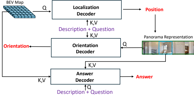
Figure 5. The framework of situated question answering [37].
