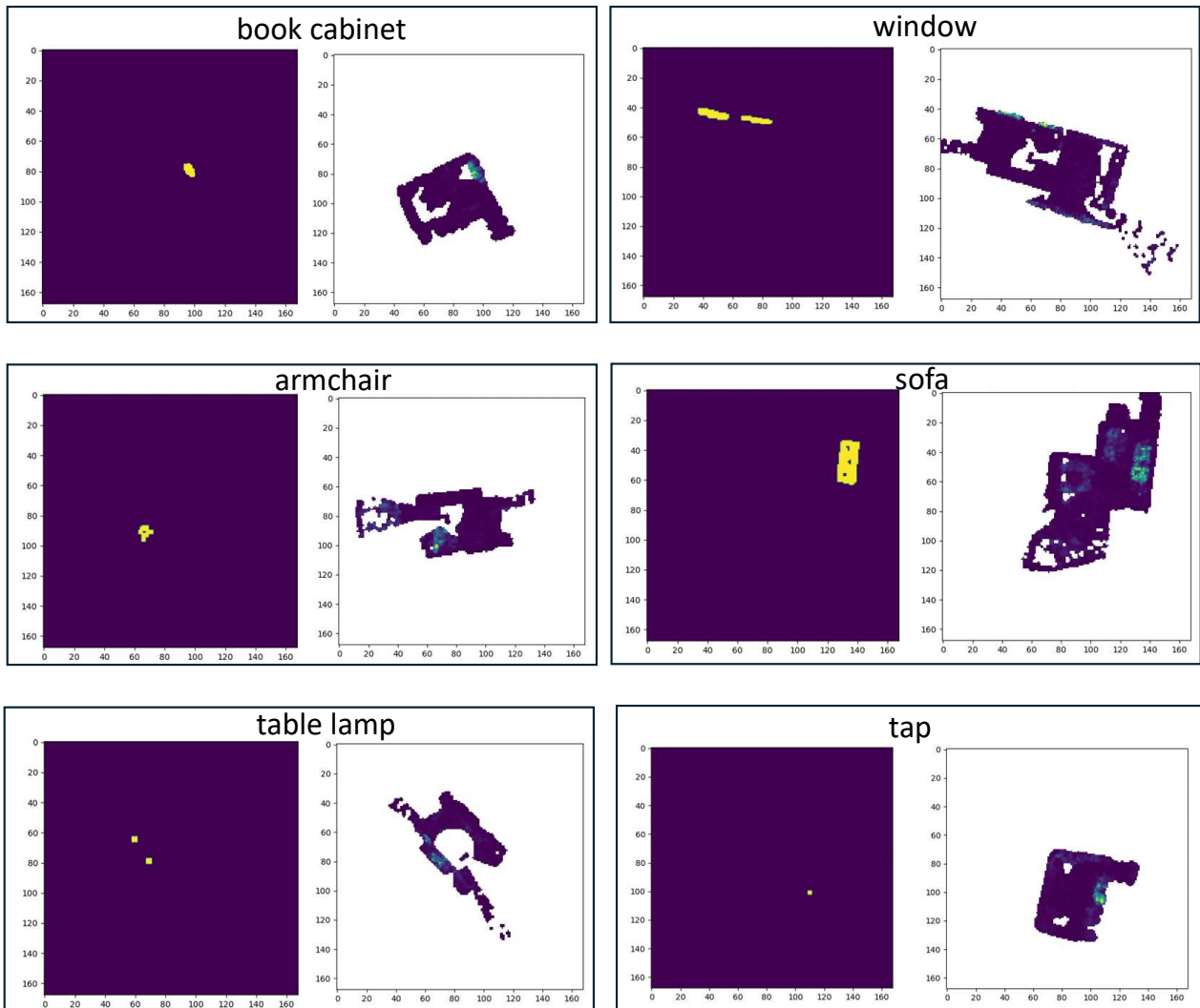
Figure 10. Visualization of querying objects on rays of the g3D-LF's BEV map. The left side of each example is GT, and the right side is the query result. Please zoom in for a better view.
