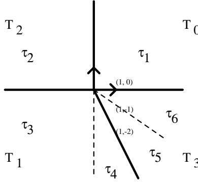
Fig.1 The secondary fan and the Gröbner fan for \mathbf{P}(2, 2, 2, 1, 1)
