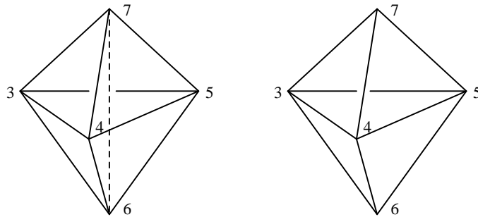
Fig.2 Two different triangulations T_A (left) and T_B (right) for the models X_7(7, 3, 2, 1, 1)
