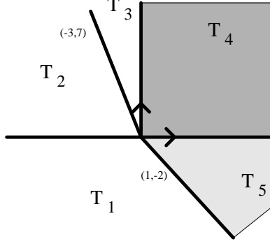
Fig.3 The secondary fan for the polyhedron \Delta^*(7, 3, 2, 1, 1)
