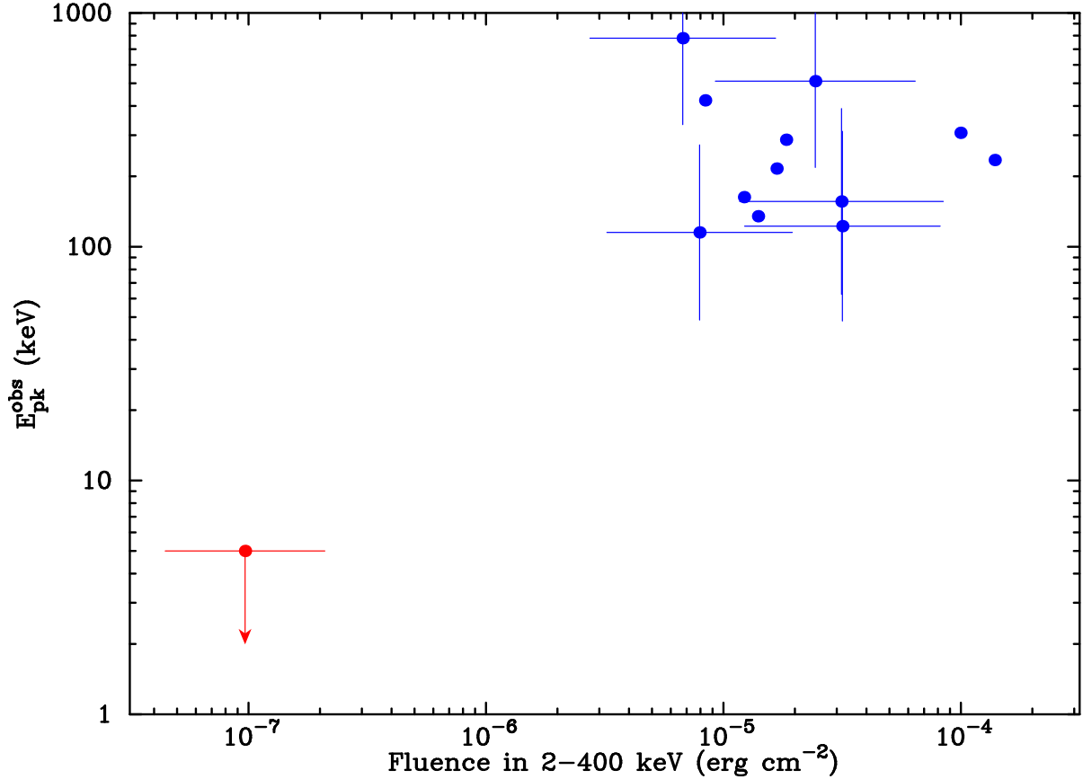
Fig. 7.— The (S_{2-400}, E_{\text{peak}}^{\text{obs}}) -plane, showing the location of XRF 020903. For E_{\text{peak}}^{\text{obs}} , we plot the 99.7% probability upper limit (5.0 keV). We calculate the 2-400 keV fluence using the best power-law model fit jointly to the WXM and the FREGATE data. The crosses show the locations of 12 of the HETE-2 GRBs studied by Barraud et al. (2003) for which E_{\text{peak}}^{\text{obs}} is relatively well determined. The properties of XRF 020903 are consistent with an extension by two decades of the hardness-intensity correlation found by Barraud et al. (2003).
