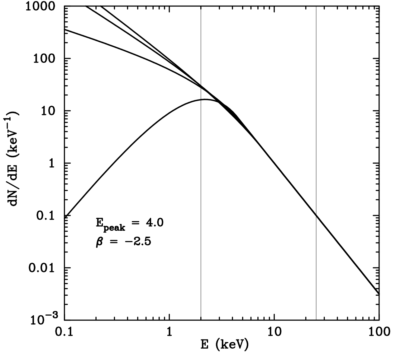
Fig. 11.— Constrained Band functions, with E_{\text{peak}} = 4 keV and \beta = -2.5 , for different values of E_{\text{pivot}} . All functions have been normalized to 1 \text{ keV}^{-1} at 10 keV. The two vertical lines at 2 keV and at 25 keV show the WXM bandpass. The spectra shown are (increasing monotonically at low energy) for E_{\text{pivot}} = 2 keV, 4 keV, 6 keV, and 8 keV, respectively. Once again, as the low-energy curvature disappears, the resulting power-law is produced by the high-energy part of the Band function. Note also that the shape of the constrained Band function is insensitive to the specific choice of E_{\text{pivot}} within a reasonable range.
