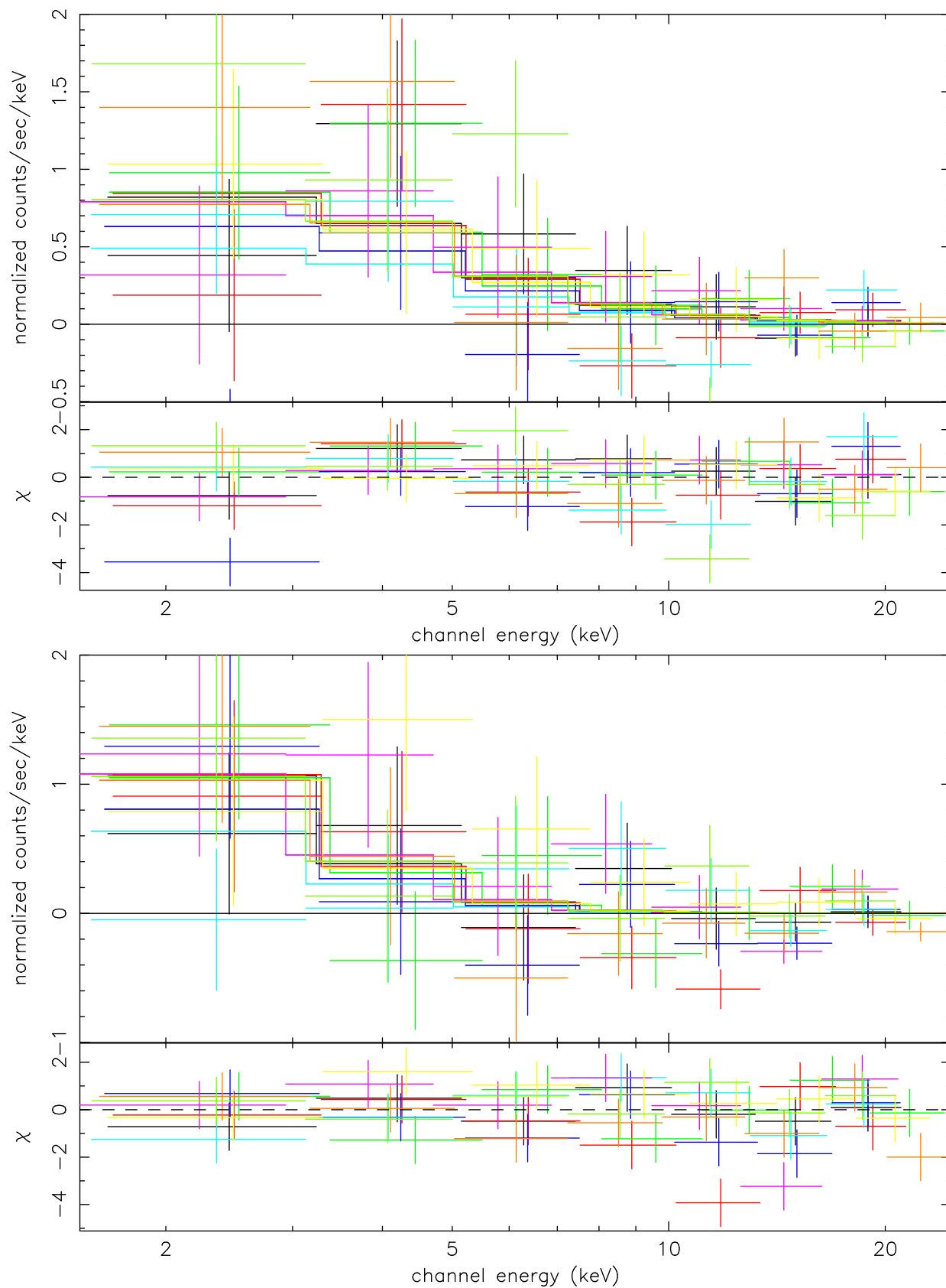
Fig. 3.— Comparison of the WXM spectra for the time intervals 0-8 and 8-13 s. The observed (crosses) and predicted (histogram) count rates are shown in a different color for each of the nine WXM wires that we have included in the fits. The spectral model is a power
