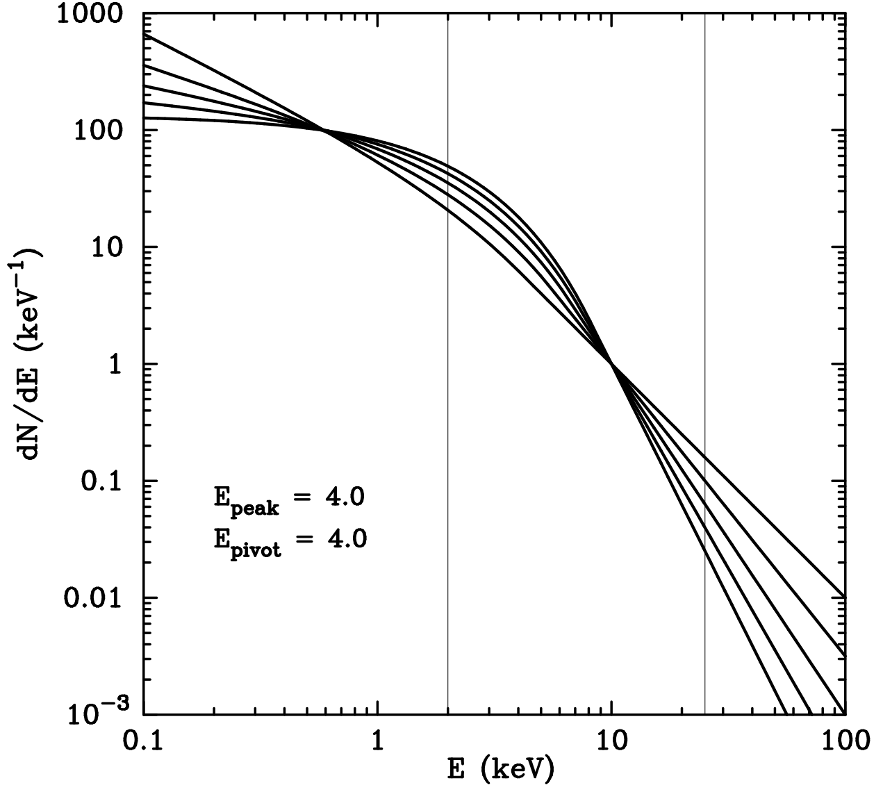
Fig. 10.— Constrained Band functions, with E_{\text{peak}} = 4 keV and E_{\text{pivot}} = 4 keV, for different values of \beta . All functions have been normalized to 1 \text{ keV}^{-1} at 10 keV. The two vertical lines at 2 keV and at 25 keV show the WXM bandpass. The spectra shown are for \beta = -2.0, -2.5, -3.0, -3.5, and -4.0 , which can be distinguished by the increasing steepness of their slopes at high energy. The progression from some curvature at low energy ( \beta = -4.0 ) to almost none ( \beta = -2.0 ) is evident, as is the fact that as the curvature disappears, the resulting power-law is produced by the high-energy part of the Band function.
