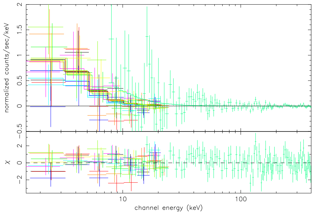
Fig. 4.— The WXM and FREGATE spectra for the entire time interval 0-13 s. The observed (crosses) and predicted (histogram) count rates are shown in a different color for each of the nine WXM wires that we have included in the fits. The spectral model is a power law with fixed photoelectric absorption (see Table 2).
