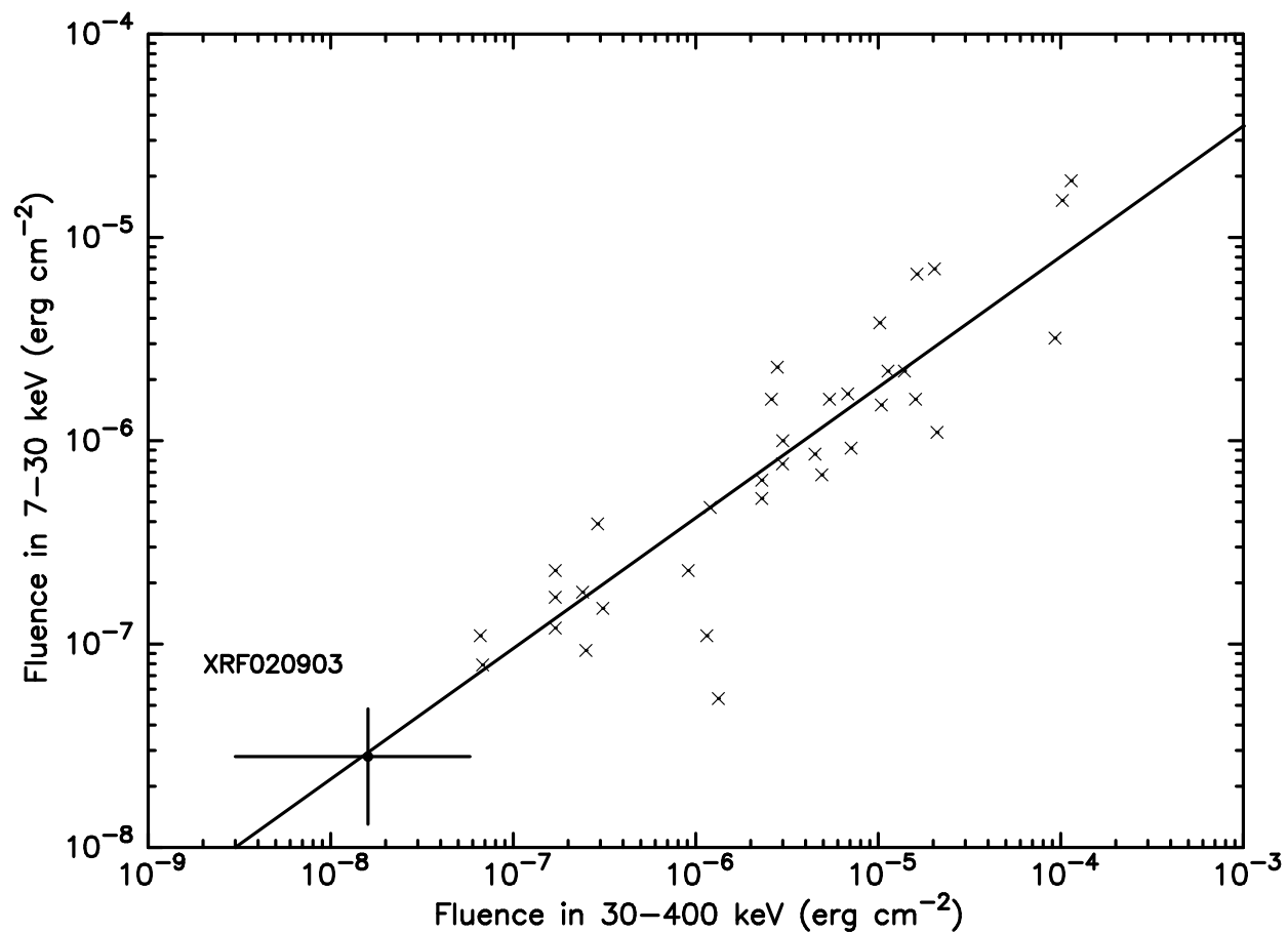
Fig. 6.— The (S_{7-30}, S_{30-400}) -plane, showing the location of XRF 020903, using the total fluence in the 7-30 keV energy band and in the 30-400 keV energy band (filled circle). The crosses are the locations of the 35 HETE/FREGATE GRBs studied by Barraud et al. (2003). The solid line is the relation, S_{7-30} = 3 \times 10^{-3} S_{30-400}^{0.643} , found by Barraud et al. (2003). The properties of XRF 020903 are consistent with this relation.
