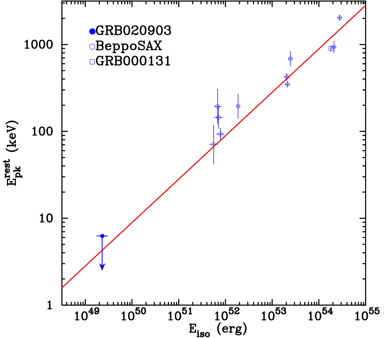
Fig. 8.— The (E_{\text{iso}}, E_{\text{peak}}) -plane, where E_{\text{iso}} is the isotropic-equivalent radiated energy between 1\text{-}10^4 keV and E_{\text{peak}} is the peak of the \nu F_{\nu} spectrum, both measured in the rest frame of the burst. The filled circle in the lower left-hand corner is the location of XRF 020903. The ten open circles are the BeppoSAX GRBs reported by Amati et al. (2002). The solid line is given by the equation, E_{\text{peak}} = 89(E_{\text{iso}}/10^{52}\text{erg})^{0.5} keV. The properties of XRF 020903 are consistent with an extension of this relation by a factor \sim 300 .
