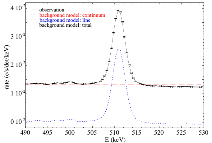
Fig. 1. Raw spectrum and background model components.
