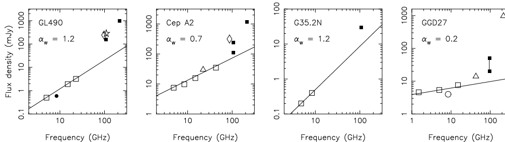
Figure 3. Spectral energy distributions at wavelengths longer than 1.3 mm. Our data are marked by filled squares; others are taken from the literature. The two points at 107 GHz for Cep A2 are for the A-array data alone (lower point) and A+B combined (upper point). The 2.7-mm flux for GGD27-IRS shows the range of values. The radio spectral index ( \alpha_w ) is shown for each source.
