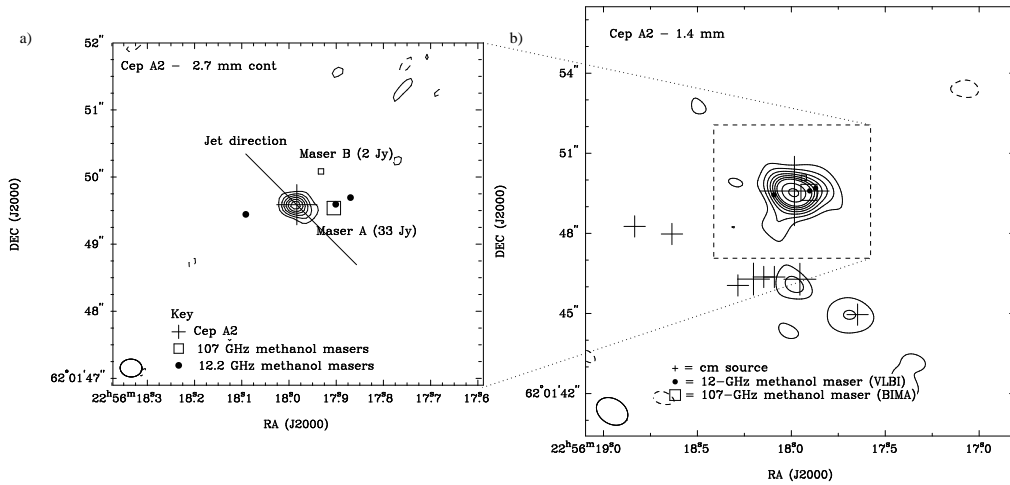
Figure 2. Continuum emission towards Cep A at a) 2.7-mm and b) 1.4 mm. Radio sources are marked by crosses, and methanol masers by filled circles (12 GHz) and open squares (107 GHz). The beams are marked in the lower left-hand corner of each panel. The direction of the radio jet is marked by the straight line.
