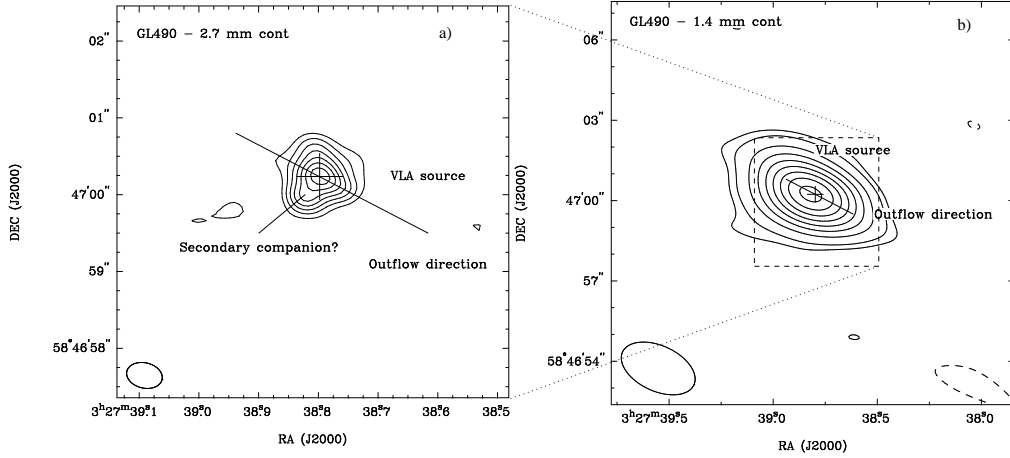
Figure 1. Continuum emission towards GL490 at a) 2.7-mm and b) 1.4 mm. The radio source is marked by a cross. The beams are marked in the lower left-hand corner of each panel by an open ellipse. The direction of the CO outflow is marked by the straight line.
