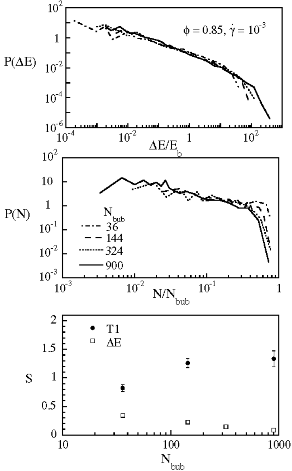
FIG. 10. Effect of system size at \phi = 0.85 and \dot{\gamma} = 10^{-3} . (a) There is no change in the power-law region of the probability density distribution compared with Fig. 6a. However, the cutoff increases and there is no convergence for the largest system sizes. (b) Even at the largest system sizes, the largest events involve a significant fraction of the bubbles in the system, indicating that the events are much more spatially extended than at \phi = 1 . (c) As in Fig. 7c, the number of T1 events and energy drops show the opposite trend. The event rates for energy drops indicate that finite size effects are more pronounced at this lower area fraction. Unlike the saturation seen in Fig. 7c, the event rate continues to drop as the system size increases.
