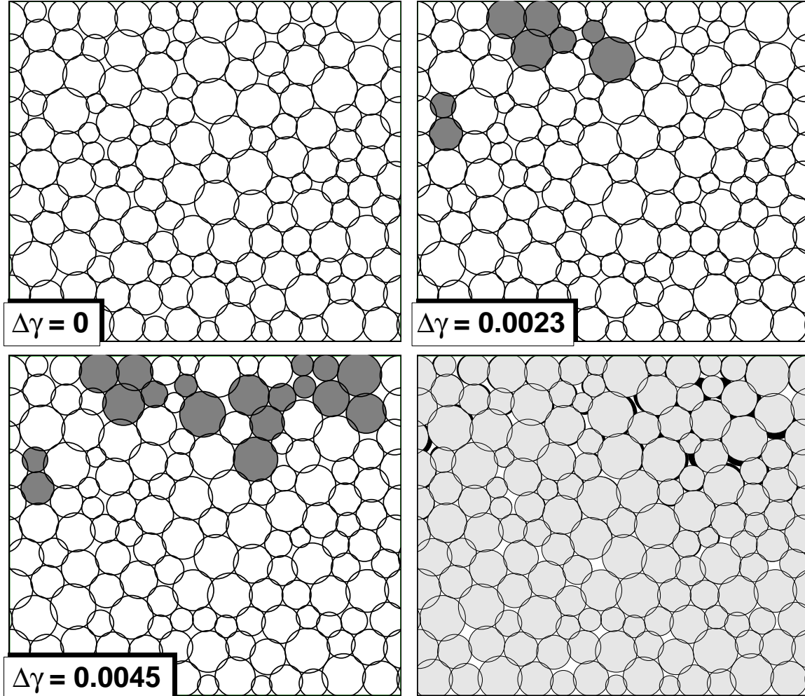
FIG. 2. Sequence of snapshots showing the nature of bubble rearrangements during an energy drop of average size in a 144-bubble system at \phi = 1.0 sheared at a rate of \dot{\gamma} = 10^{-3} . The magnitude of the drop ( \Delta E/E_b = 2.61 ) and the fraction of bubbles that change overlapping neighbors ( N/N_{bub} = 0.18 ) are both close to average. The first three frames show the configurations of bubbles at the start, middle and end of the energy drop, respectively. As the event proceeds, more and more bubbles change overlapping neighbors, as shown by the gray bubbles. The fourth frame shows the final configuration with bubbles in light gray superimposed on the initial configuration with bubbles in black. Most of the bubble motions involve subtle shifts of bubble positions; there are no topological rearrangements in this event. Note that although this event appears to nucleate at the top, in general the events appear randomly throughout the sample.
