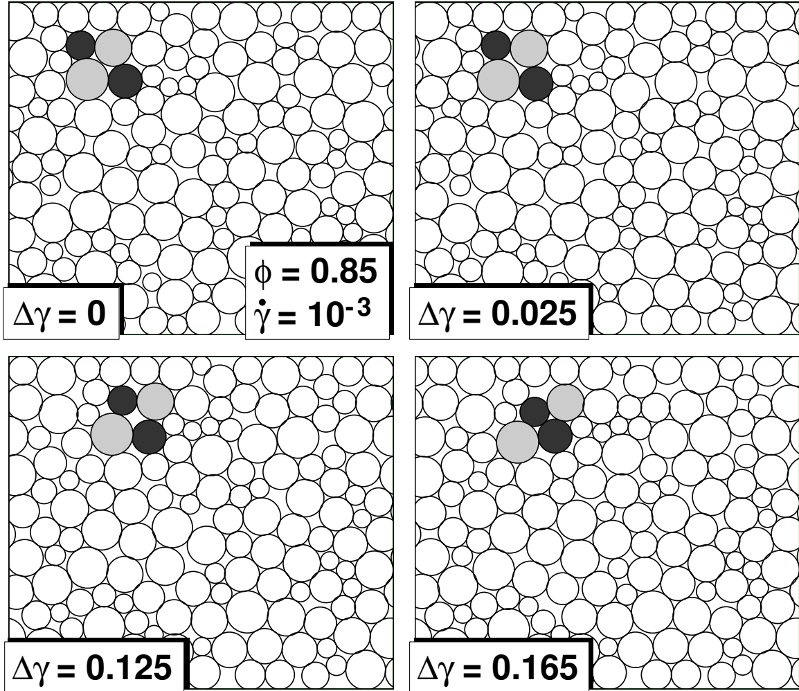
FIG. 5. A sequence of snapshots showing a T1 event in a wet foam at \phi = 0.85 as the system is strained at \dot{\gamma} = 10^{-3} . During the event, the black pair of bubbles moves together and the gray pair moves apart.
