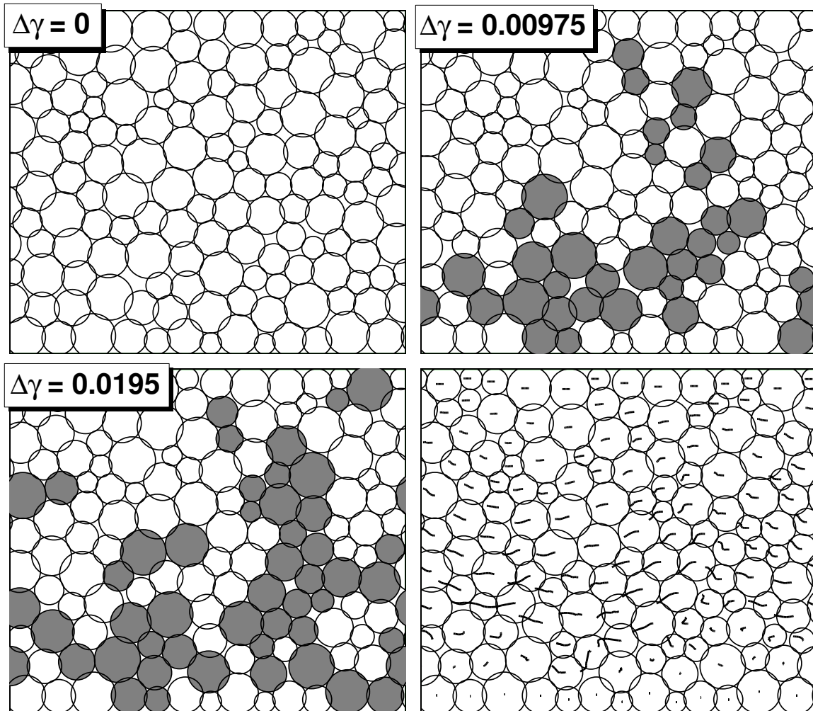
FIG. 3. Sequence of snapshots showing bubble rearrangements during a large energy drop in a 144-bubble system at \phi = 1.0 and \dot{\gamma} = 10^{-3} . The magnitude of the drop ( \Delta E/E_b = 13.18 ) and the fraction of bubbles that change overlapping neighbors ( N/N_{bub} = 0.44 ) both fall in the upper tails of the distributions. The first three frames show the configurations at the beginning, middle and end of the energy drop; the gray bubbles have changed overlapping neighbors since the start of the drop. The fourth frame shows the final configuration along with the tracks made by the centers of the bubbles during the event. We did not use the same scheme as in the fourth frame of Fig. 2 to show the rearrangements because the bubble motions were too extensive in this case.
