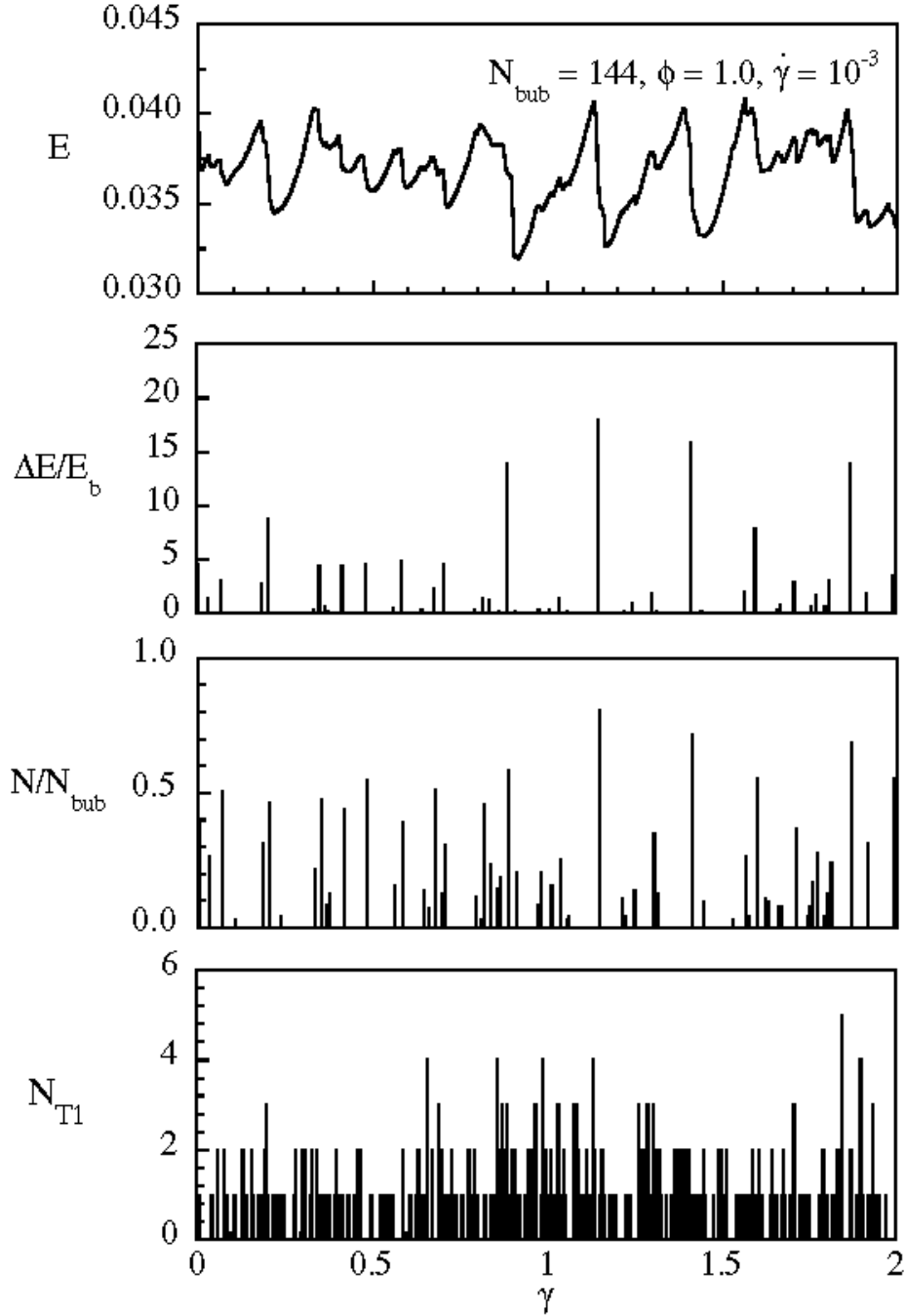
FIG. 1. Elastic energy and rearrangements vs strain for a 144-bubble system, with gas (area) fraction \phi = 1 , being slowly sheared at rate \dot{\gamma} = 10^{-3} . The top plot (a) shows the total elastic energy stored in the “springs” of overlapping bubbles. Plot (b) shows the size of the energy drops that occur as the system is sheared. Note that the duration of an energy drop is very short compared to the time between energy drops at this low shear rate. Plot (c) shows the corresponding fraction of bubbles that experience a change in overlapping neighbors during each precipitous energy-drop event. The bottom plot (d) marks the mid-point of each T1 event, where two bubbles begin to intrude between two others; these have no direct correspondence to the energy drop events seen in (a) and (b). The behavior of all the properties shown here indicates that flow is accomplished inhomogeneously and intermittently by sudden rearrangements.
