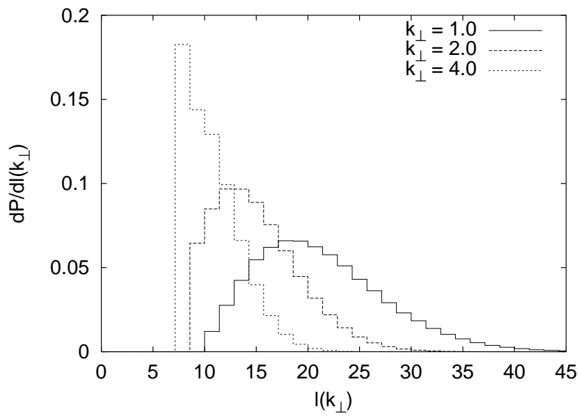
Figure 3: The \ell(k_{\perp}) -distribution for different k_{\perp} -values at \sqrt{s} = 200 GeV.
