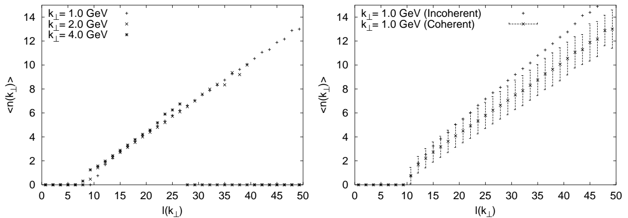
Figure 5: The figure to the left shows a plot of \langle n(k_{\perp}) \rangle versus \ell(k_{\perp}) for an e^+e^- event with \sqrt{s} = 200 GeV from PYTHIA. The figure to the right shows \langle n(k_{\perp}) \rangle \pm \sigma versus \ell(k_{\perp}) at \sqrt{s} = 200 GeV, k_{\perp} = 1.0 GeV for coherent and incoherent showers in PYTHIA.
