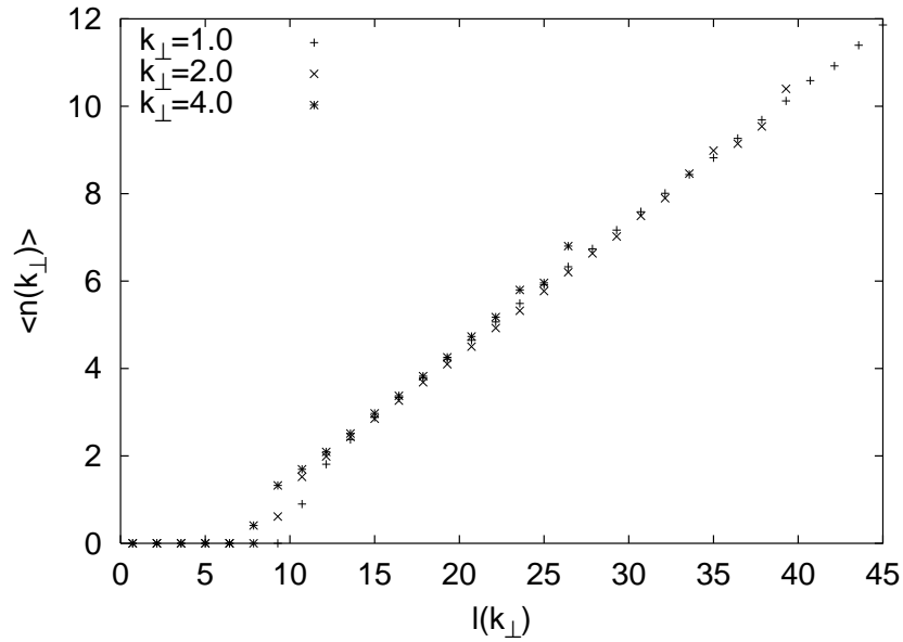
Figure 2: The figure shows a plot of \langle n(k_{\perp}) \rangle versus \ell(k_{\perp}) for an e^+e^- -event with \sqrt{s} = 200 GeV from ARIADNE.
