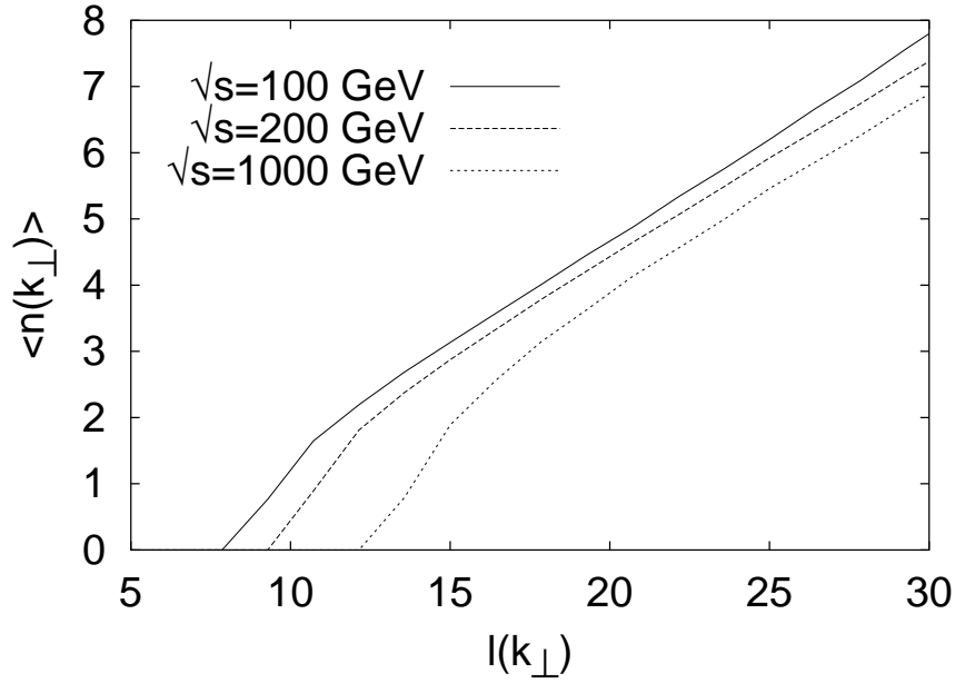
Figure 4: The figure shows a plot of \langle n(k_{\perp}) \rangle versus \ell(k_{\perp}) ( k_{\perp} = 1.0 GeV) for different cms energies from ARIADNE.
