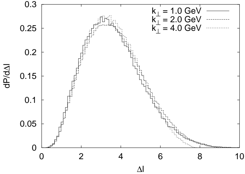
Figure 7: The \frac{dP}{d(\Delta\ell)} \equiv P_\ell(\Delta\ell) -distribution from ARIADNE.
