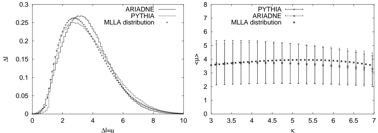
Figure 12: The figure to the left shows the distribution f_\delta(\mu, \kappa) , obtained from the MLLA approach at k_\perp = 1\text{GeV} , compared with the P_\ell(\Delta\ell) distribution from ARIADNE and PYTHIA (cf. Fig. 10). The figure to the right shows the average value of \mu as a function of \kappa , from the same distribution f_\delta(\mu, \kappa) . In the figure to the right, we also compare with the average value of \ell (cf. Eq. (21)) as a function of \kappa obtained from ARIADNE and PYTHIA, and we also include the standard deviation in the result from PYTHIA and ARIADNE. This result is obtained using \alpha_0 = 0.7 and C_r = 2 in the MLLA distribution as explained in the text.
