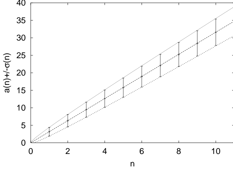
Figure 9: The figure shows the average \Delta\ell (and the standard deviations around it) for chains of n connected \Delta\ell called a(n) ( a(n) \equiv \langle \sum_{j=1}^n \Delta\ell_j \rangle ). The statistics is collected from events with a fixed number of gluons.
