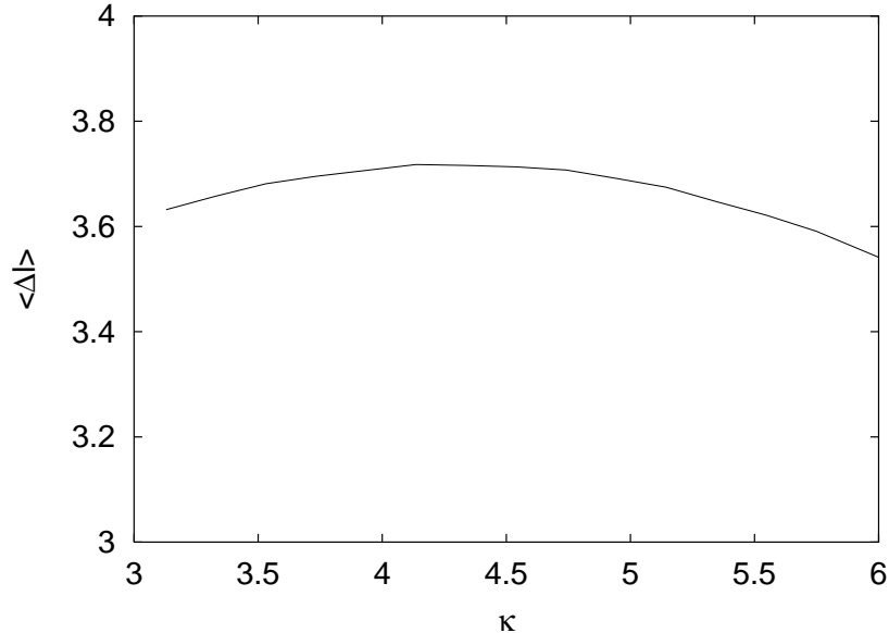
Figure 8: The average value of \Delta\ell as a function of \kappa \equiv \ln(k_{\perp}^2/\Lambda^2) . Note that the variation in the average \Delta\ell in the figure is much smaller than the width of the distribution of \Delta\ell as seen in Fig. 7.
