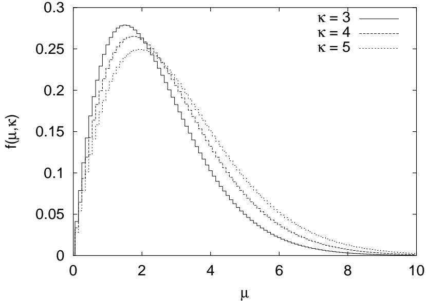
Figure 11: The f_\kappa(\mu) function, obtained from Eq. 31, normalised to unity.
