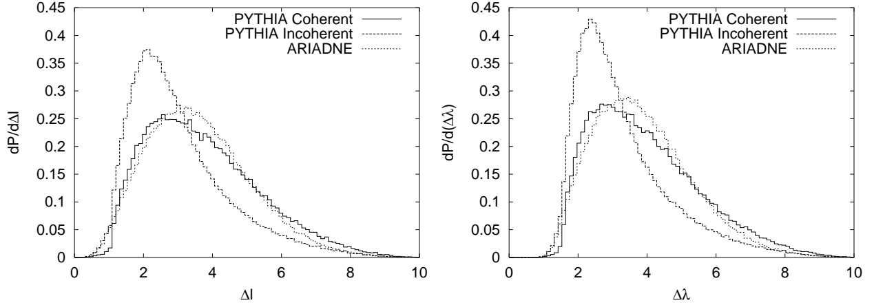
Figure 10: The figure to the left shows the P_\ell(\Delta\ell) -distribution from PYTHIA compared to the distribution obtained from ARIADNE. The figure to the right shows the corresponding plot for the P_\lambda(\Delta\lambda) distribution.
