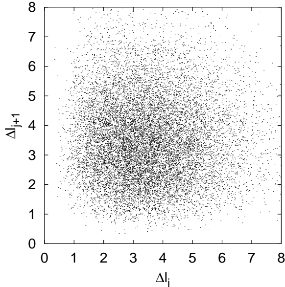
Figure 6: Scatter plot of two adjacent \Delta\ell values
